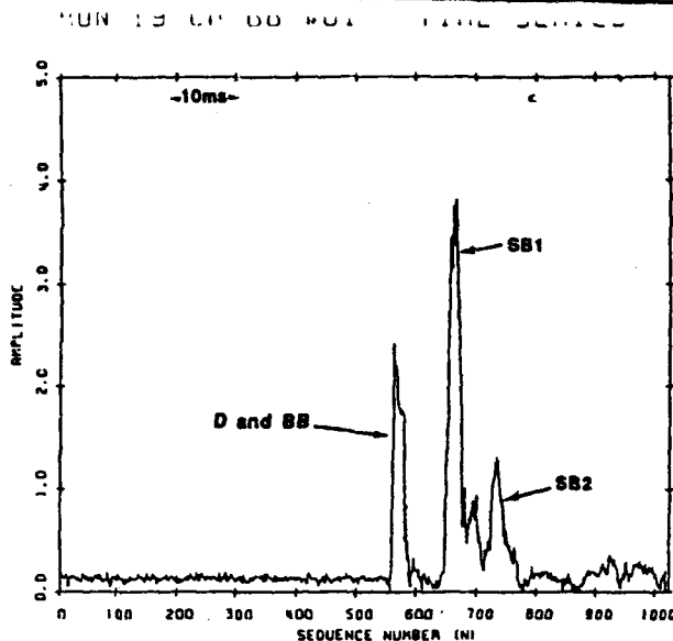
Figure 2. Event arrivals.
