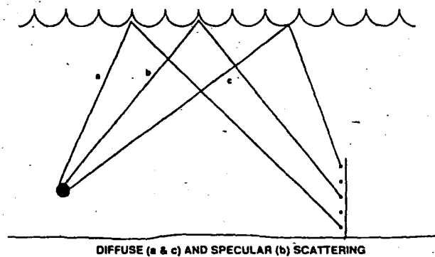
Figure 6. Scattering geometries.
