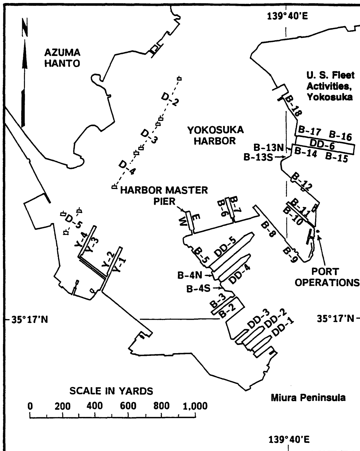
Figure V-3. Harbor configuration of Fleet Activities, Yokosuka.
