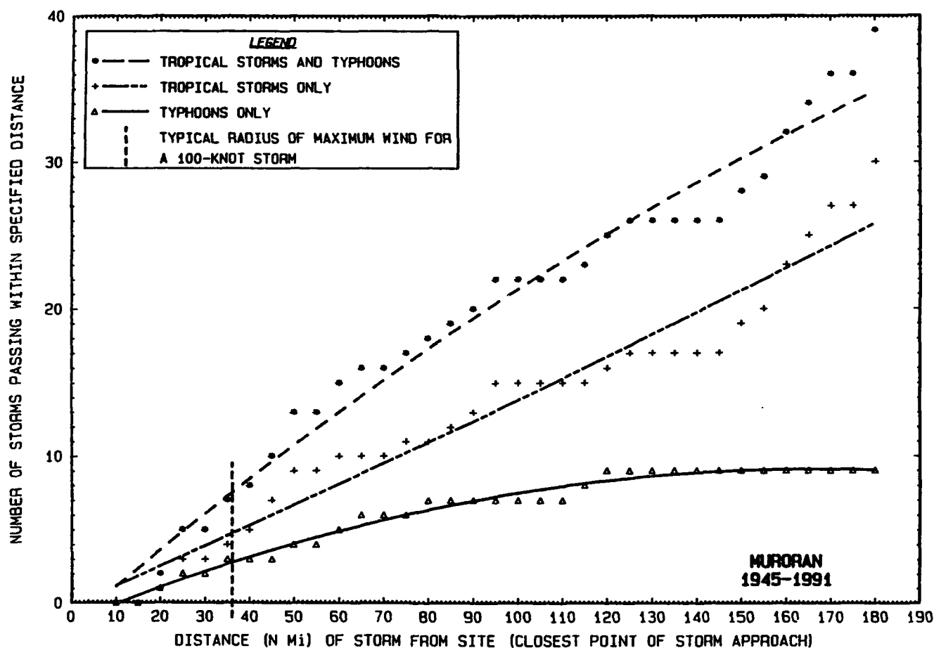
Figure V-137. Number of tropical cyclones passing at various distances from Muroran during the 47-year period of record. Tropical storm or typhoon classification is based on maximum wind near storm center while that center was within 180 nmi of Muroran, and not necessarily at CPA. Sloping lines represent mathematical fit to data points. Average radii of maximum wind for 34, 100, and 140 kt storms at Muroran are 37.6, 36.0, and 33.1 nmi respectively.
