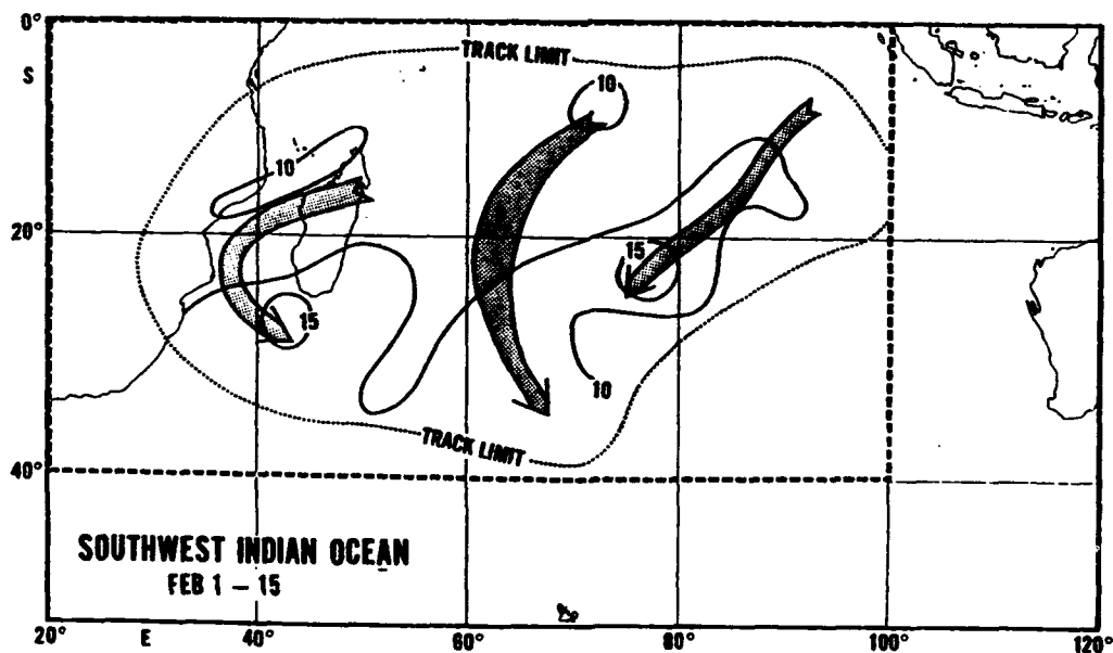
Figure C-2. Preferred Southwest Indian Ocean tropical storm and hurricane tracks (Feb 1-15). Isolines show the average storm speed of movement in knots.
