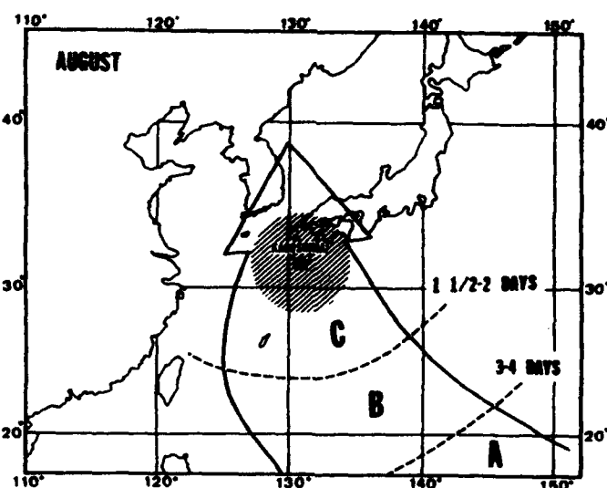
Figure V-88. Tropical cyclone threat axis for Kagoshima for the month of August. Approach times to Kagoshima are based on typical speeds of movement for tropical cyclones affecting Kagoshima.
