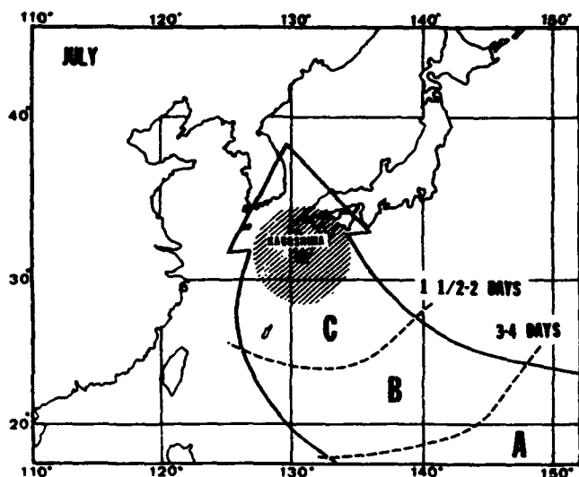
Figure V-87. Tropical cyclone threat axis for Kagoshima for the month of July. Approach times to Kagoshima are based on typical speeds of movement for tropical cyclones affecting Kagoshima.
