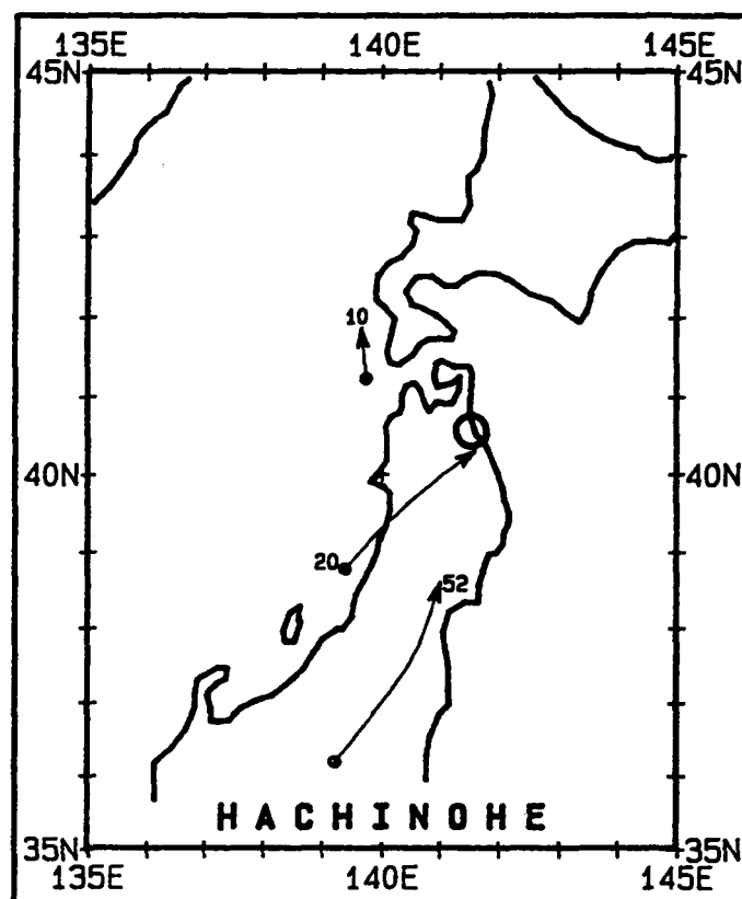
Figure V-154. Track segments of the 3 tropical storms or typhoons causing sustained winds of at least 34 kt at Hachinohe during the 43-year period 1948-1991. Index numbers correspond to those given in Table V-35.
