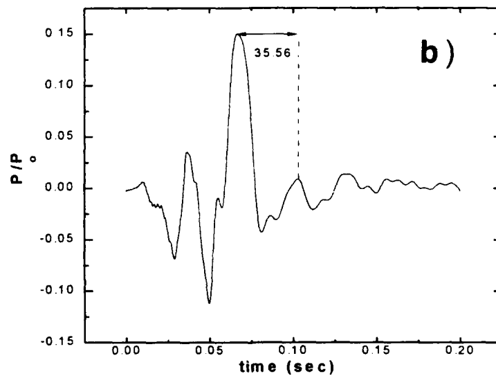
Fig. 5.8 Envelope a 50 cycle burst at a frequency 4.2 kHz at 10.74 m from the drivers. The acoustic intensity at the source is a) 150 dB and b) 178 dB.
