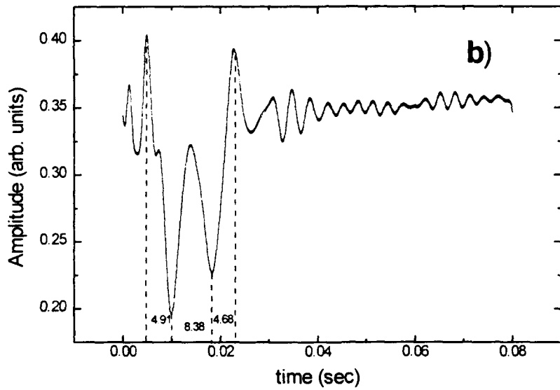
Fig. 5.7 Modulation envelope of a 4500 Hz carrier wave at 7.69 m the source showing peak to peak time intervals. The intensity level at the source is: a) 144 dB, and b) 156 dB.
