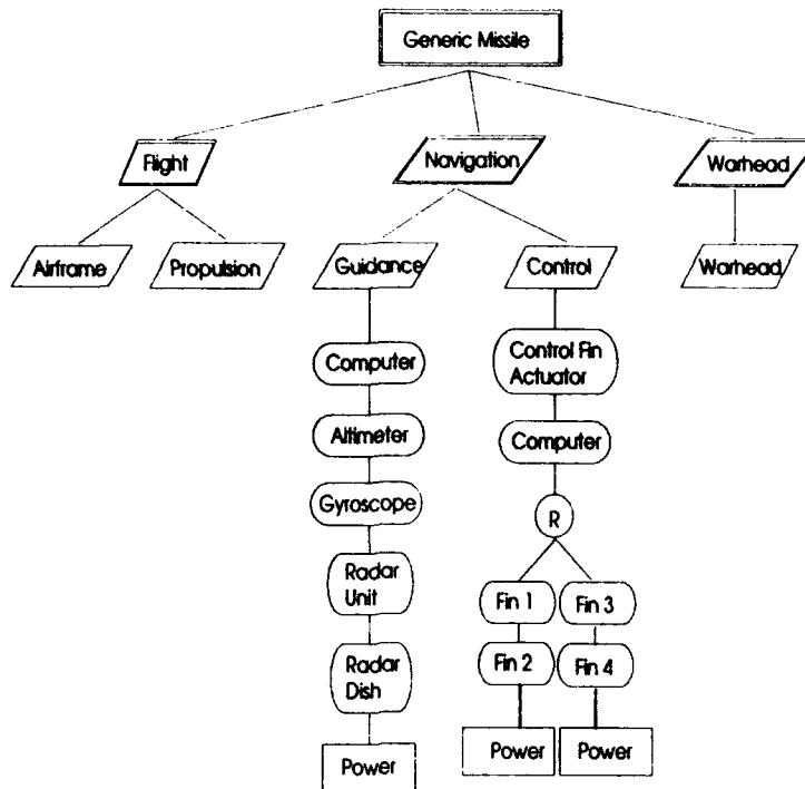
Figure 9: Fault Tree Description of Generic Missile With Power Module.
