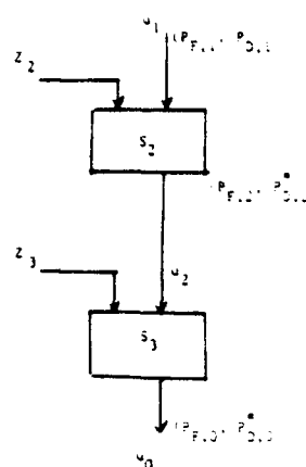
Fig. 16(b). Serial scheme with three sensors.
