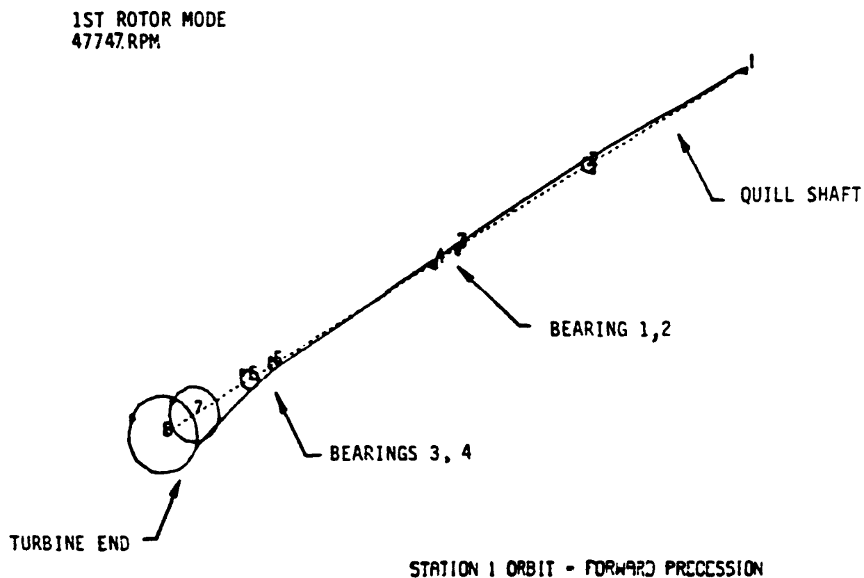
Figure 16 Rotor Group Mode Shape MX 49-F TURBINE TESTER - DAMPED CRITICAL SPEEDS DESIGN - DUPLEX SLAVE BRGS, 1.45 IN SHAFT DIA BETWEEN BRGS
