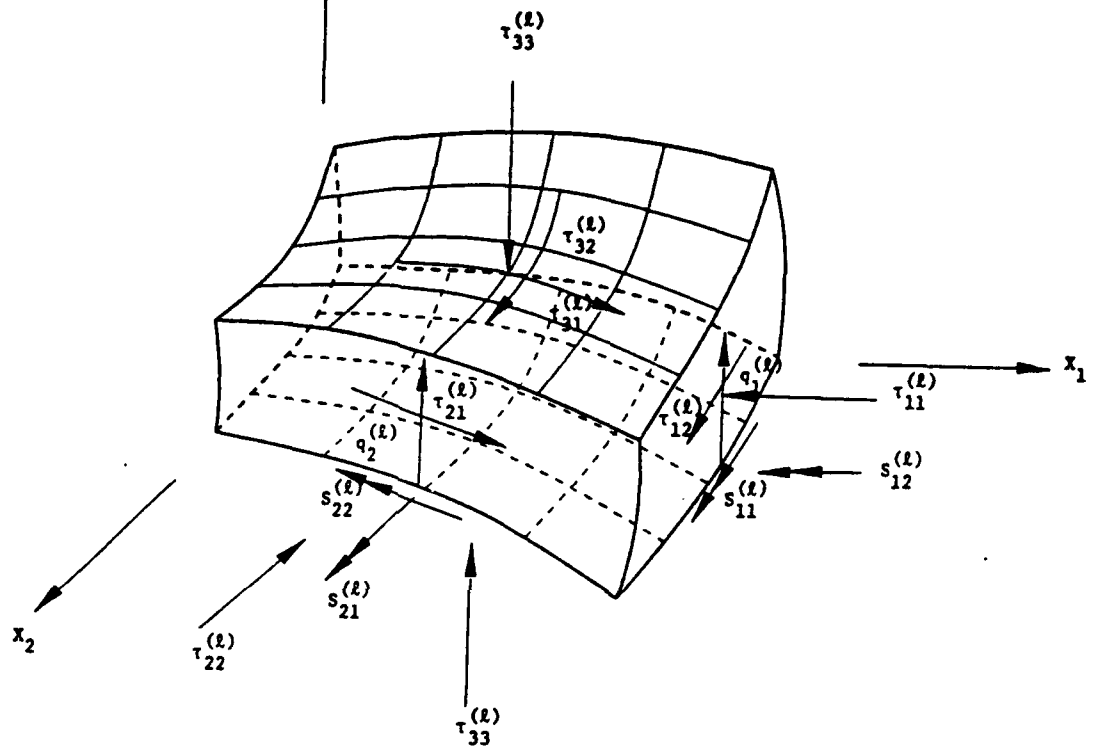
Fig. 13.1b Stress representation on a typical finite element layer
