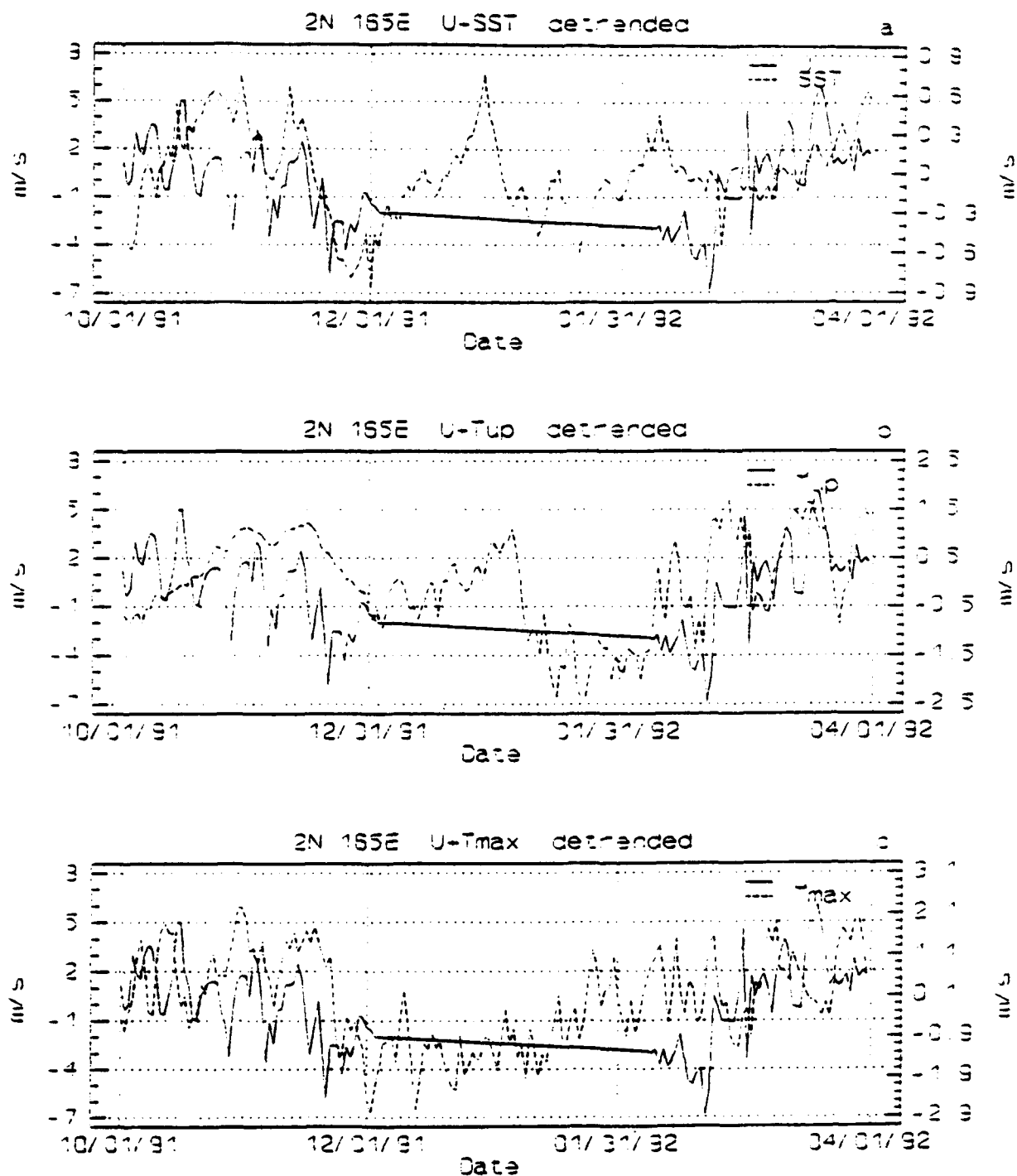
Fig. 25. U/ocean temp. relations at 2°N 165°E, within transition region. Time series of detrended U and overlaid: a) SST, b) Twp, and c) Tmax. Long straight lines are data gaps.
