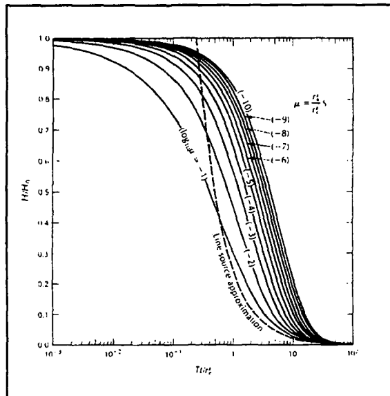
Figure 3 Transmissivity / Time Function Curves
