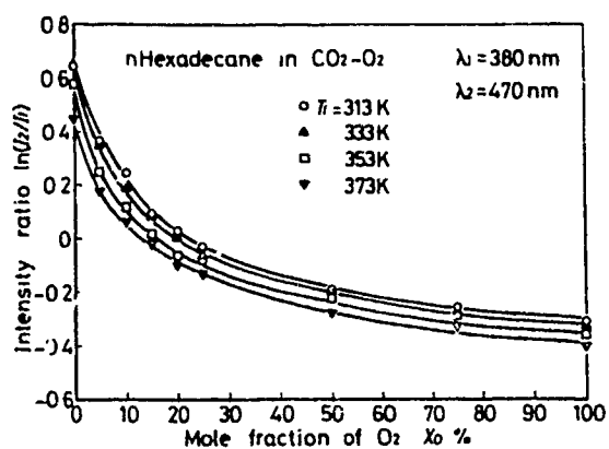
Fig. 3 Relationship between intensity ratio and Oxygen concentration (n-Hexadecane in CO_2-O_2 )
