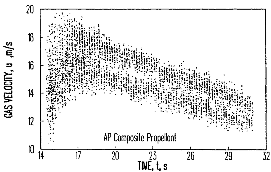
Fig.3 Data obtained by LDA technique with a forcing frequency f=5 Hz in the frequency response.
