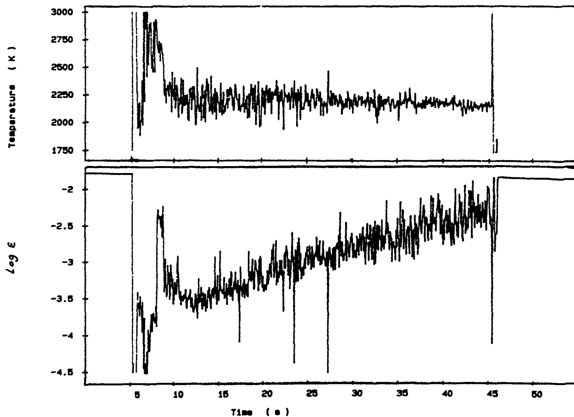
Figure 5 Two-colour temperature (top) and emissivity (bottom)
