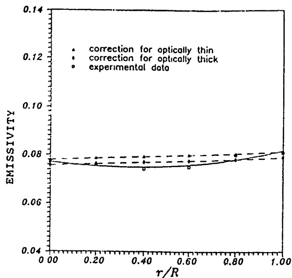
Fig.3 Empirical value of emissivity compared with standard value.
