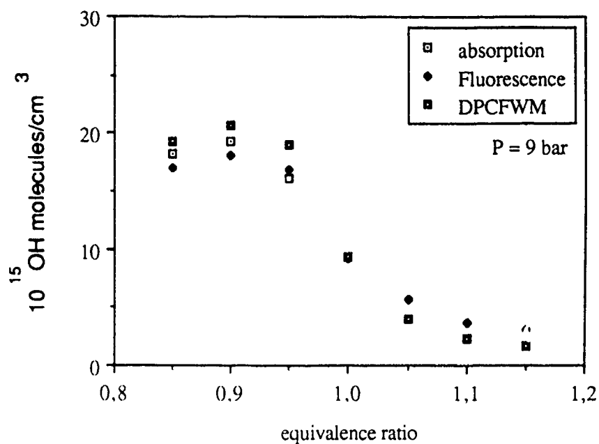
Figure 1 : OH number density in the postflame gases (i.e. 5 mm above the burner) as a function of equivalence ratio at 9 bar obtained by absorption, LIF, and DPCFWM. To take into account quenching effects the LIF intensities have been multiplied by 7.0
