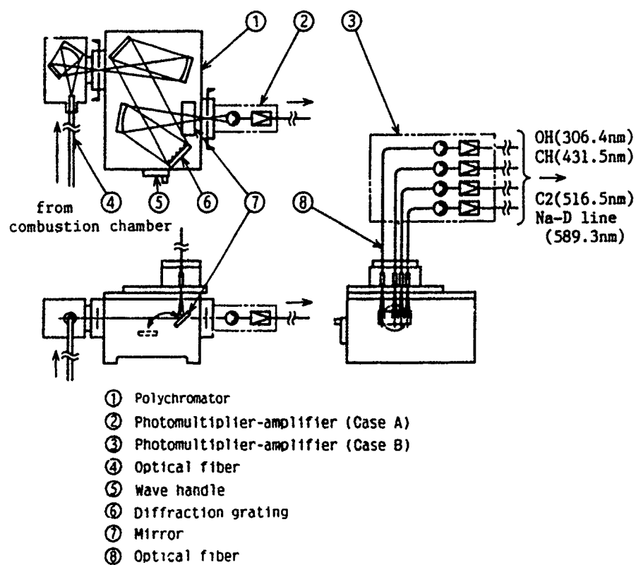
Fig.1 Polychromator for measuring emission and absorption behavior at four wavelengths simultaneously
