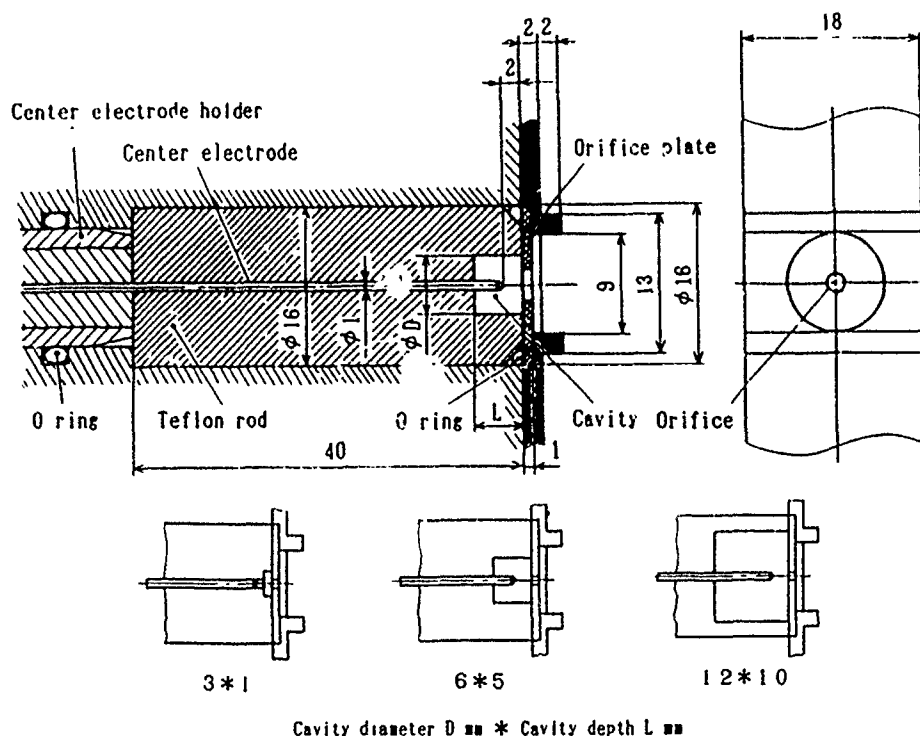
Fig. 1 Cross section of plasma jet igniter and three kinds of cavity. Three different cavity are 3*1, 6*5 and 12*10. Symbol of 3*1 denotes the cavity diameter D of 3 mm and the cavity depth L of 1 mm. Each volume is about 7.1, 141.4 and 1131.0 mm 3 .
