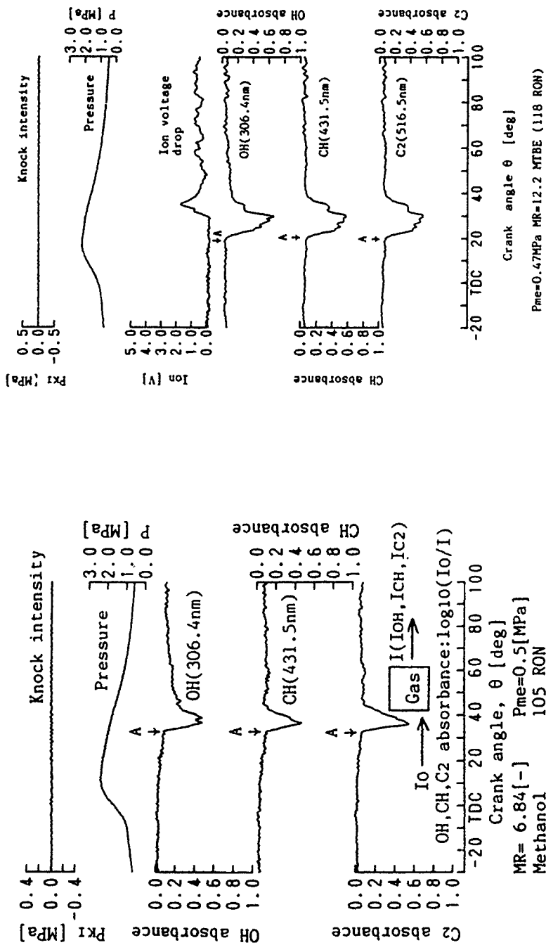
Fig.9 Normal combustion with methanol with (105 RON) Fig.10 Normal combustion with MTBE (118 RON)
