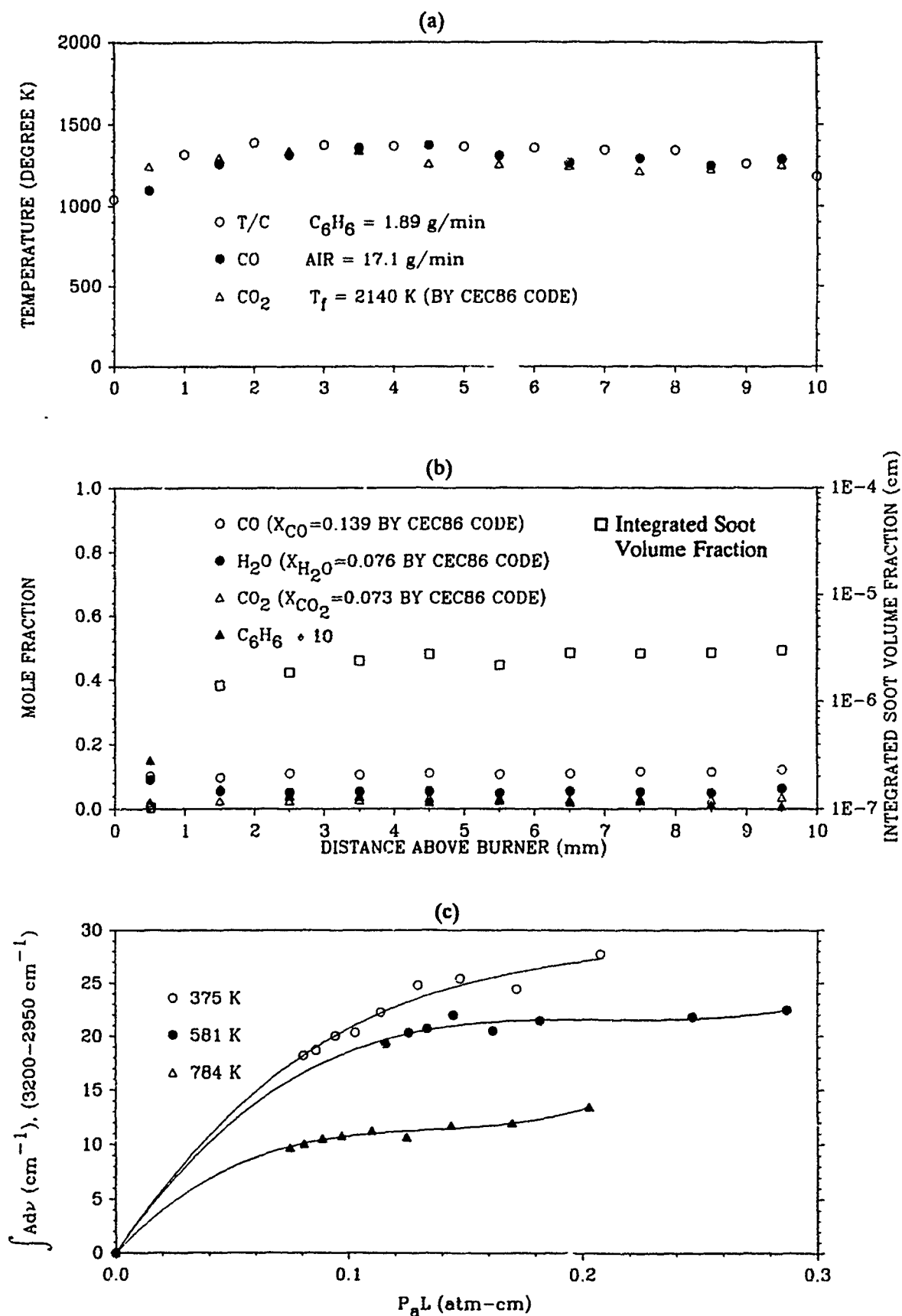
Fig. 2 Measured profiles of temperature, absolute species mole fractions, and integrated soot volume fraction in a premixed C_6H_6 /air flame with an equivalence ratio \phi=1.47 , as well as calibration data between integrated absorbance and partial pressure of C_6H_6 .
