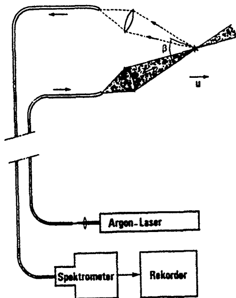
Fig. 1 Optical arrangement for flow velocity measurements
