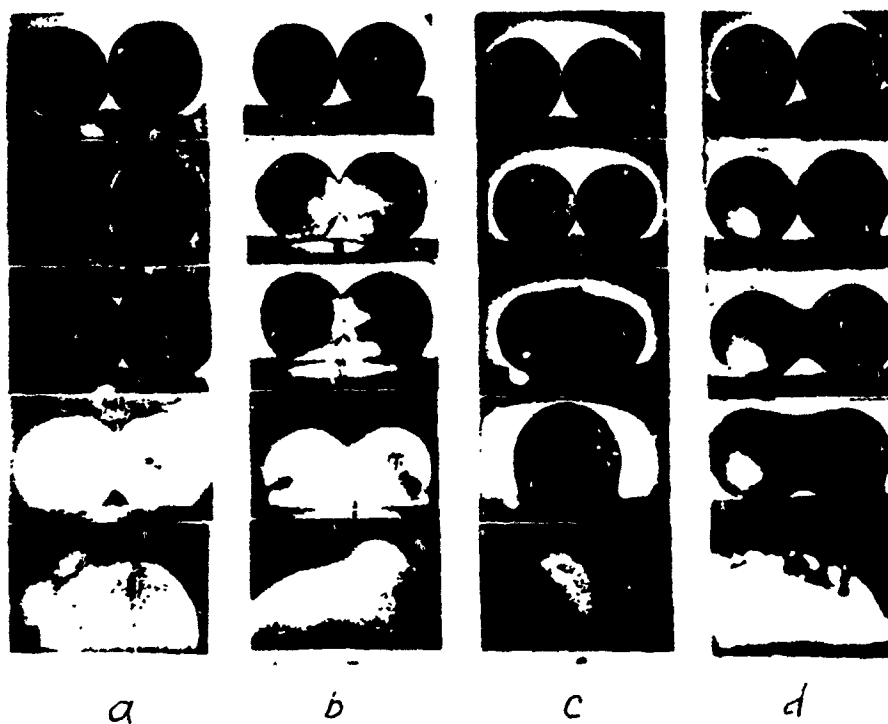
Fig.1. Typical agglomeration pattern of aluminium particles.
