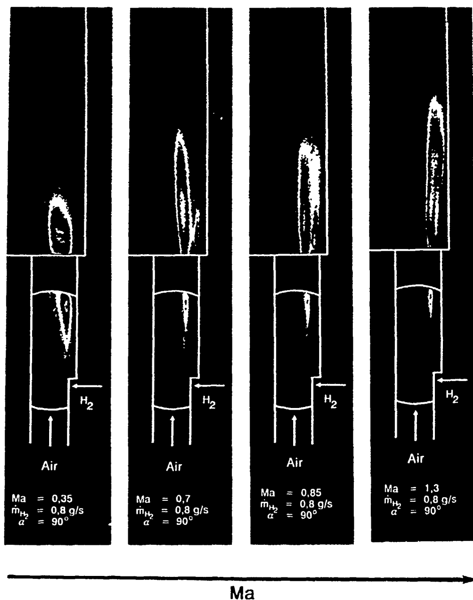
Fig. 2: Stabilization and structure of H_2 -air flames as a function of the air Mach number (self fluorescence: exposure time t_{exp} = 1 \text{ ms} )
