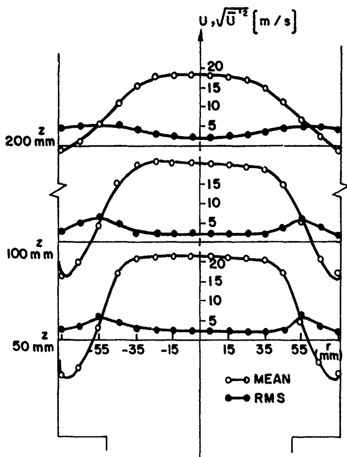
Fig. 3. Mean and r.m.s. velocity measurement by LDA 22 .
