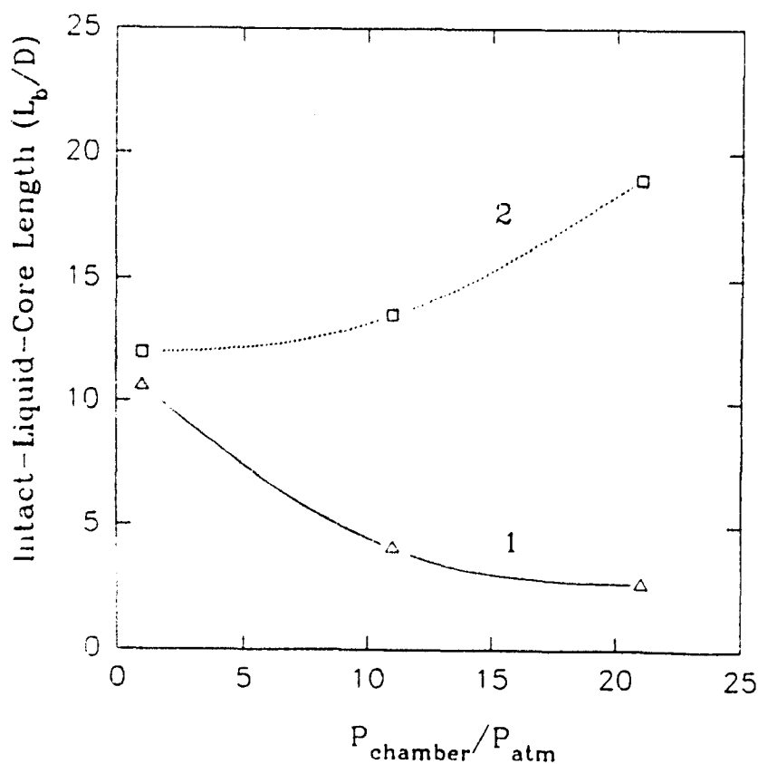
Figure 3. Effect of chamber pressure on intact-liquid-core length.
