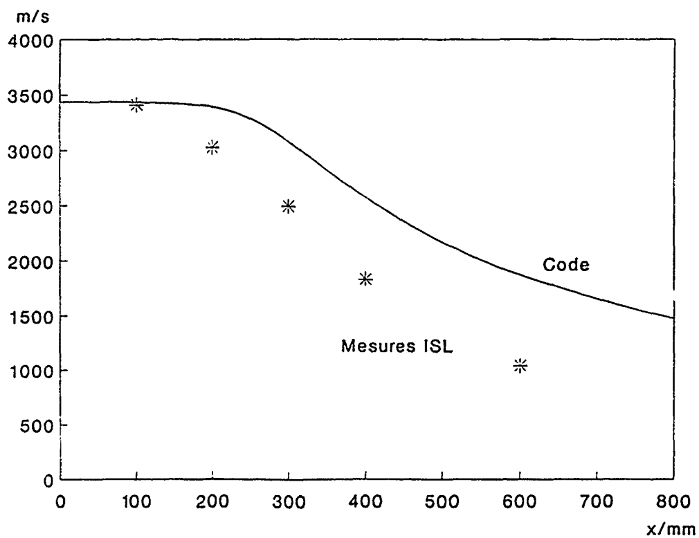
Fig. 3 Mean velocities at the axis of hydrogen combustor jet
