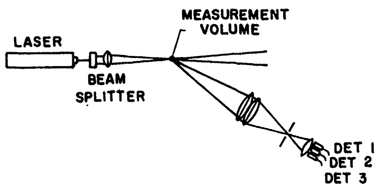
Fig. 4. PDA optical system.
