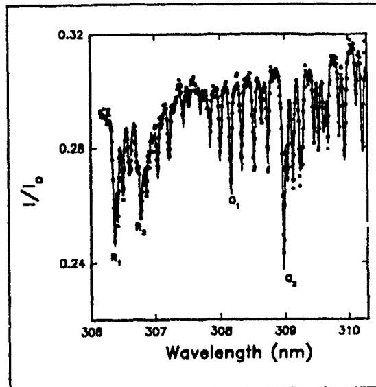
OH Absorption Spectrum Taken in the Luminous Flame Region of JA2 burning in 1.6 MPa nitrogen.
