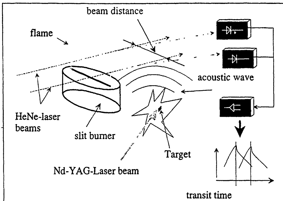
Fig.1 Temperature measurement by opto-acoustic laser beam deflection
