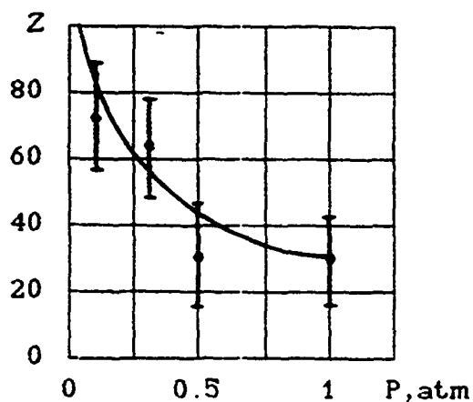
Fig.1 The dependence of MgO particles net charge on external pressure:
