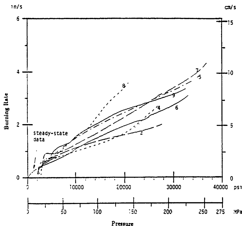
Fig. 1 Transient burning rate versus pressure
