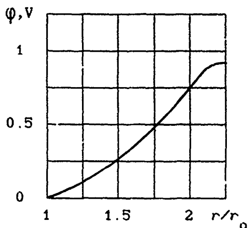
Fig.2 Distribution of the electrical potential near the burning Mg particle, ( r_0 - particle radius)
