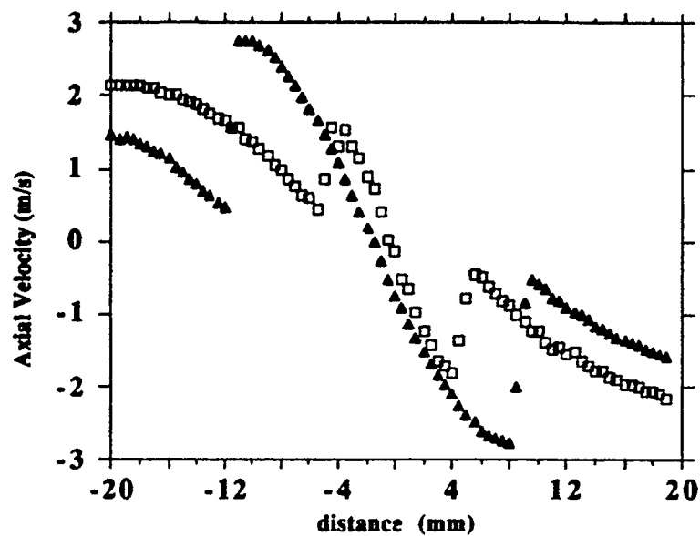
Fig.4. LDA axial velocity profiles for a stoichiometric flames and various inlet velocity (1.5 and 2 m/s).
