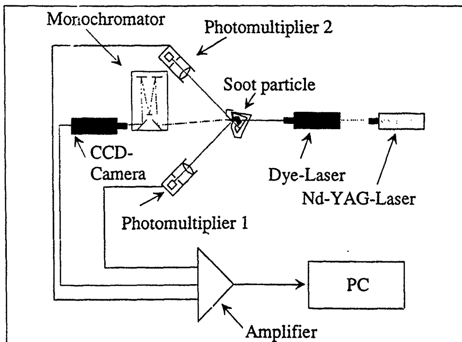
Fig. 2: Scattering light experiment for particle measurement
