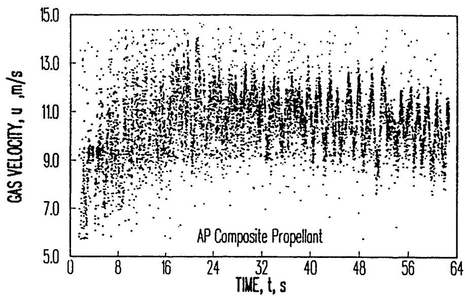
Fig.2 Typical gas velocity behavior in the self-sustained oscillatory combustion regime.
