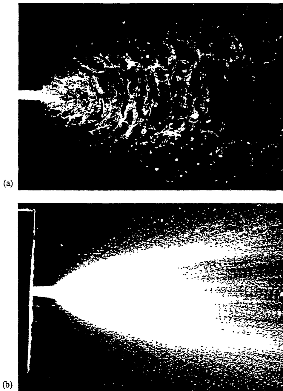
Figure 1. Copper-vapor-laser-sheet-illuminated images of like-on-like impinging jets. (a) Instantaneous picture. (b) Multiple-exposure picture.
