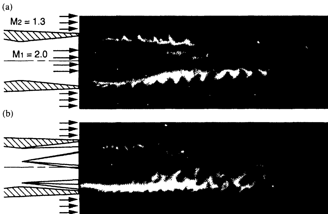
Figure 1. Planar Mie scattering images of supersonic coaxial air jets. The center jet is seeded with ethanol vapor and the outer jet is unseeded. (a) circular nozzle, (b) nozzle with five swept ramps on the expansion side.
