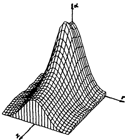
Fig. 3. Absorption coefficient \kappa vs. radius r and distance from the burner z .
