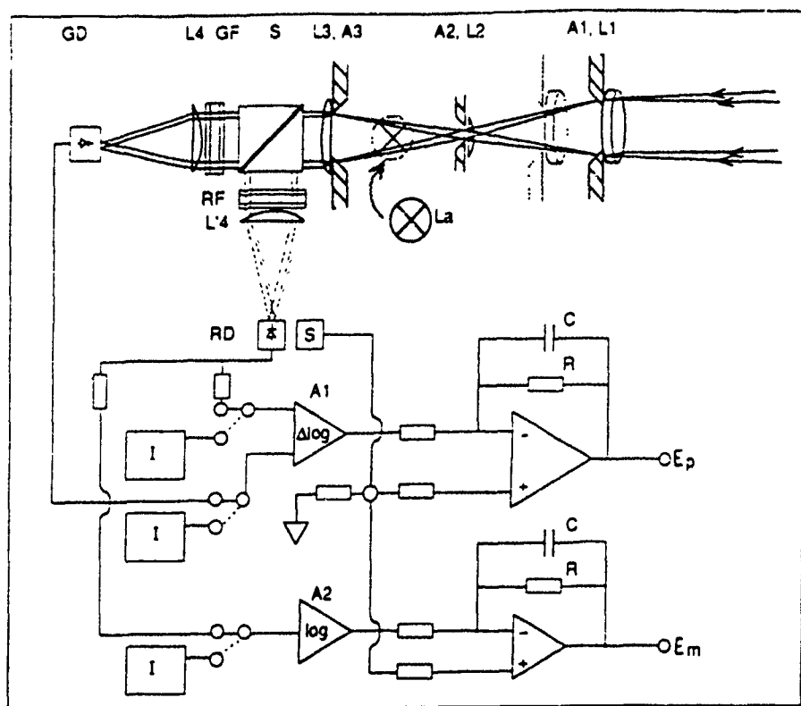
Figure 4 Layout of the two-colour pyrometer
