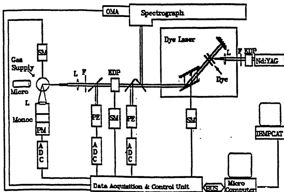
Fig.1. The schematic of the experimental rig.
