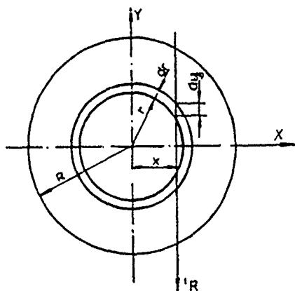
Fig. 1. Gas volume in cylindrical geometry.
