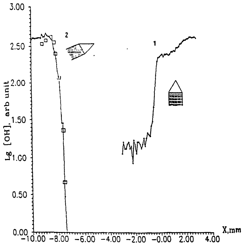
Fig.2. Profiles of the fluorescence signal for methane -air flames ( \phi=1.3 ). 1. Vertical position of Bunsen burner. 2. Horizontal position of luminous front. Points - OH concentration for flame with \phi = 1.25 [1].
