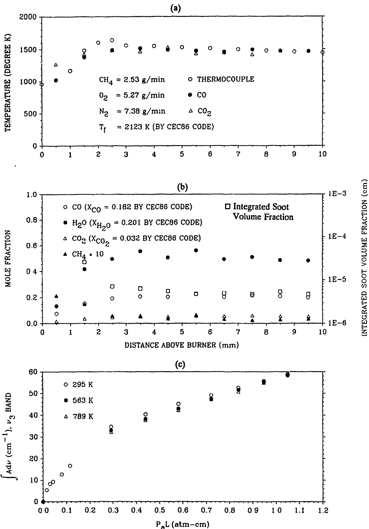
Fig. 1 Measured profiles of temperature, absolute species mole fractions, and integrated soot volume fraction in a premixed CH 4 /air flame with an equivalence ratio \phi=1.94 , as well as calibration data between integrated absorbance and partial pressure of CH 4 .
