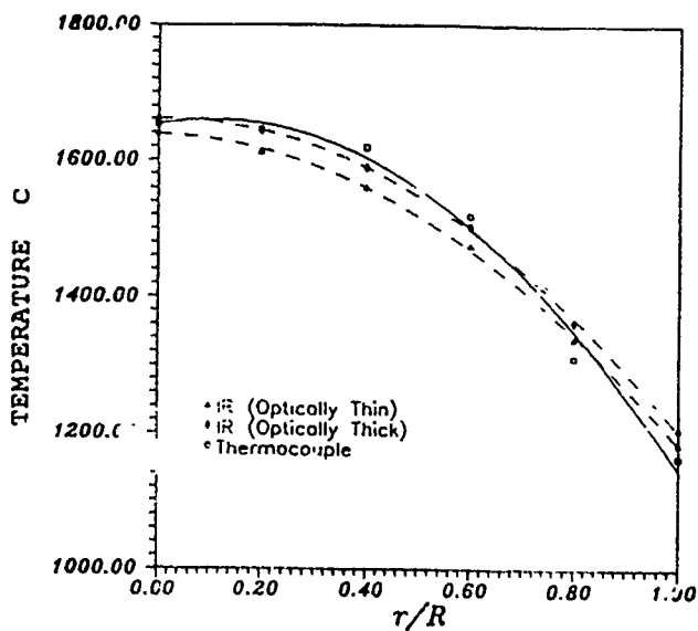
Fig.4 The IR temperature which is deduced by empirical correlation equation compared with thermocouple temperature.
