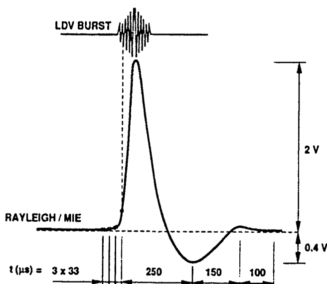
Figure 2. Schematic diagram of the simultaneous measurement of LDV and Rayleigh scattering, giving rise to the Mie contamination on the Rayleigh signal
