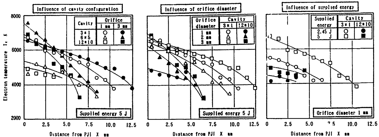
Fig.6 Local electron temperature T_e measured at the time when the most intense luminous intensity was measured as a function of distance X from plasma jet igniter for various conditions.
