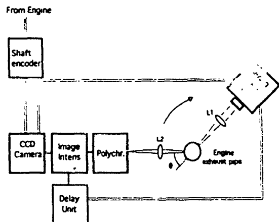
Fig.1 Experimental set-up
