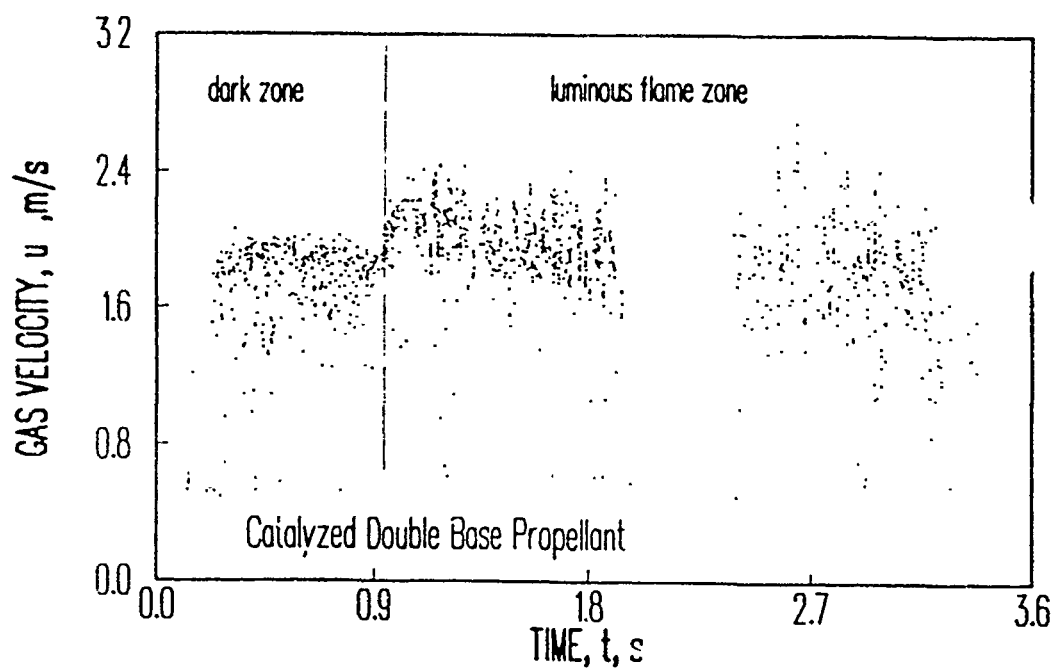
Fig.1 Double Base flame structure by LDA technique.
