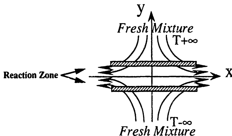
Fig.1. Strained premixed flames formed by counterflow mixtures.
