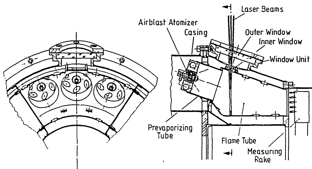
Figure 1. Combustor segment with window unit
