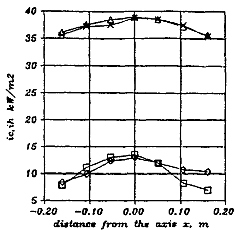
Fig. 2. Measured values of radiation intensity with cold- and hot background.
