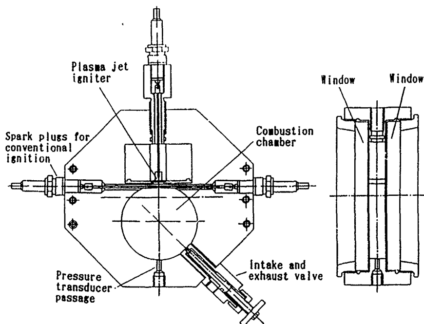
Fig. 2 Figure of constant volume combustion vessel. The combustion chamber has a cylindrical shape; diameter of 80 mm, depth of 20 mm and volume of 100 c.c..
