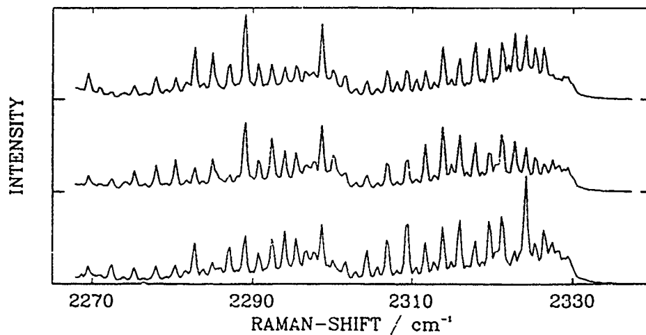
Fig.2: The first three single shots of the ensemble corresponding to Fig.1.
