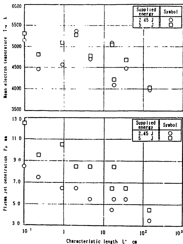
Fig.7 Mean electron temperature T_m and the penetration depth of plasma jet P_p as a function of characteristic length L^* .
