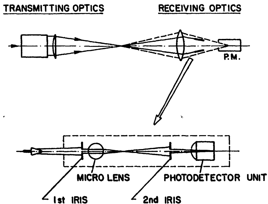
Fig. 2. LDA flow speed and particles size measurement 21 .
