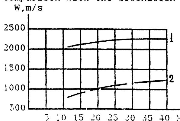
Fig.1. Curves of thrown plates acceleration.
