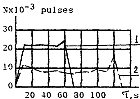
Fig. 2. Plot of registrations of AE signal intensity under explosive material combustion in a chamber with holes: 1 - 3 mm \phi , 2 - 4 mm \phi ; N - AE intensity, pulses; \tau - time, s.
