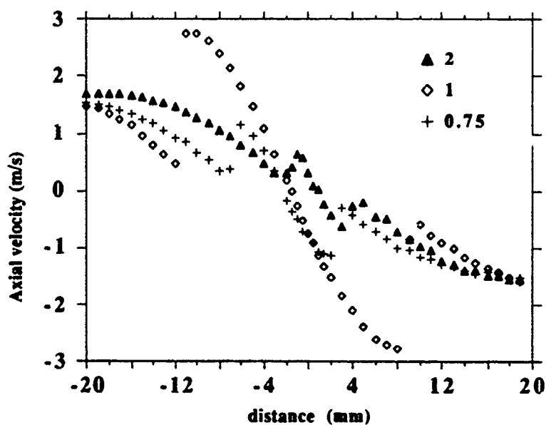
Fig.5. LDA axial velocity profiles for lean, stoichiometric and rich flames, inlet velocity = 1.5 m/s.
