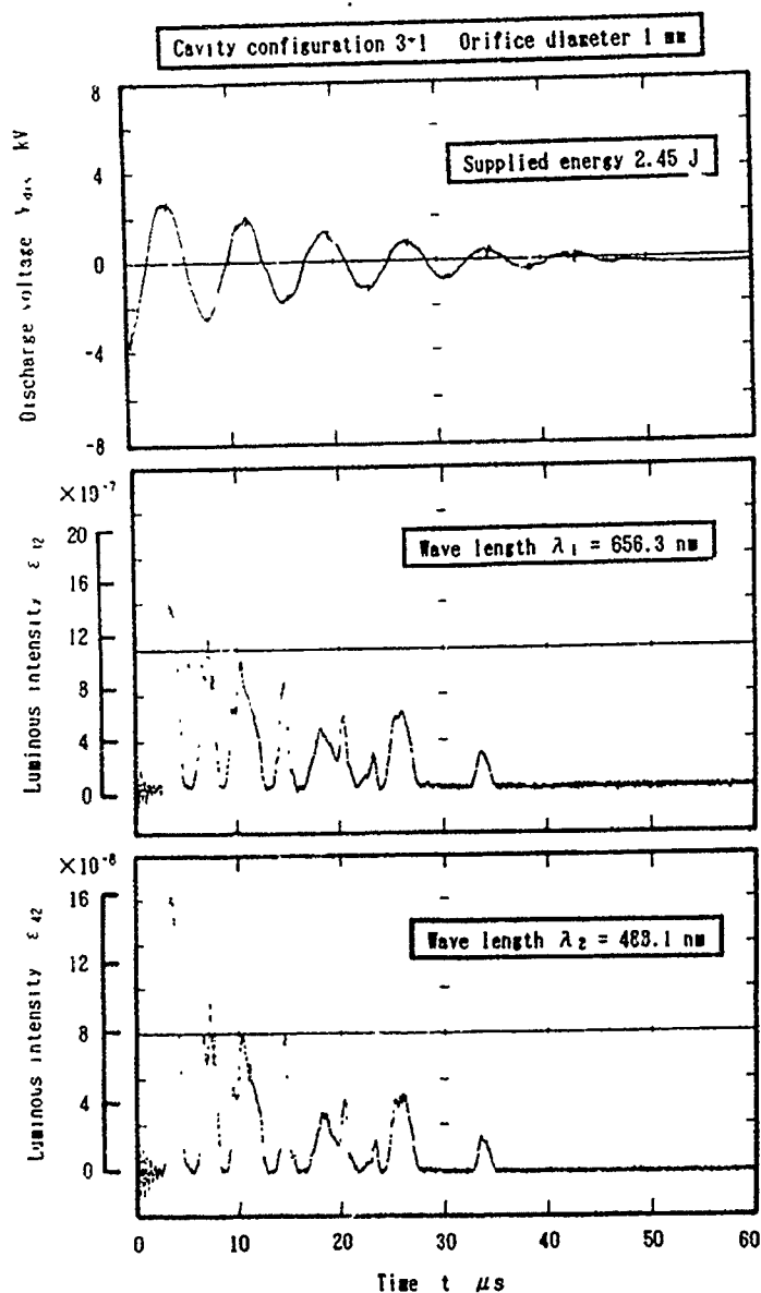
Fig.5 Typical wave forms of discharged voltage at supplied electric energy of 2.45 J and luminous intensities of wave length 486.1 nm and 656.3 nm measured at distance of 1.5 mm from plasma jet igniter. Cavity configuration: 3*1; orifice diameter: 1 mm.
