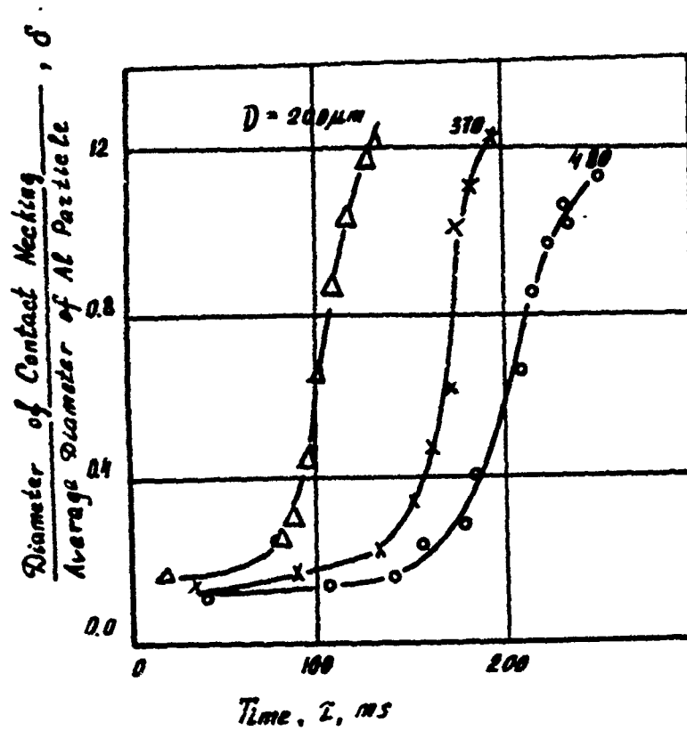
Fig.2. The dependence of contact necking growth from particle size.
