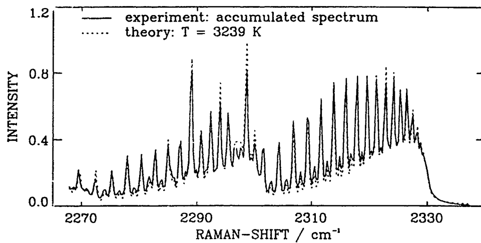
Fig.1: Temperature fit to an experimental nitrogen spectrum consisting of 15 accumulated single shots.
