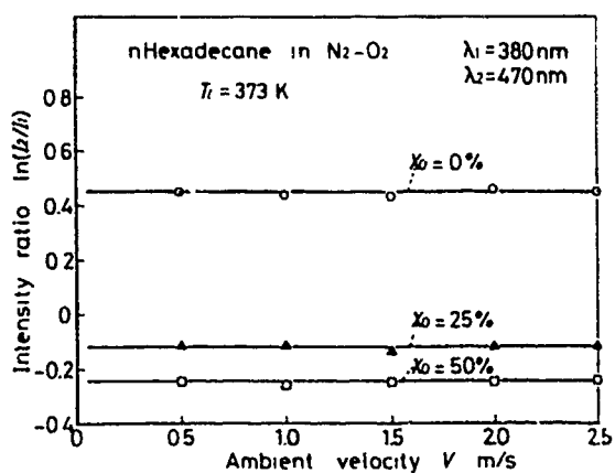
Fig. 4 Relationship between intensity ratio and gas velocity (n-Hexadecane in N_2-O_2 )
