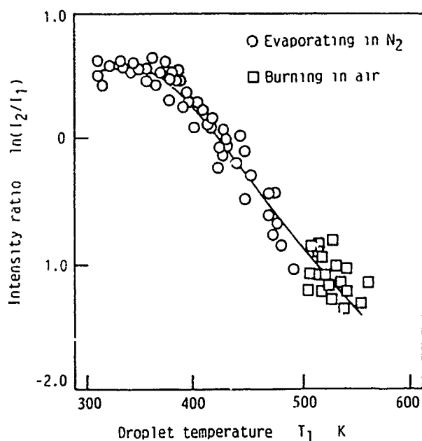
Fig. 2 Relationship between intensity ratio and droplet temperature (n-Hexadecane burning in air and evaporating in N_2 )
