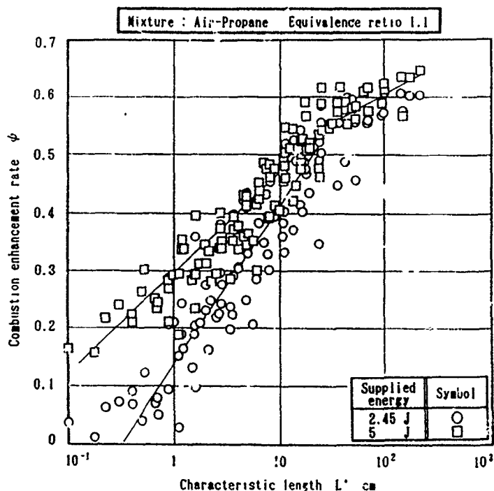
Fig.4 Combustion enhancement rate \phi as a function of characteristic length L^* . Air-propane mixture equivalent ratio:1.1. Here the combustion enhancement rate \phi is defined by the ratio of the burning time of the plasma jet ignition \tau_{pl} and that of the conventional ignition \tau_{con} , \phi is expressed by the equation; \phi = 1 - \tau_{pl} / \tau_{con} .
