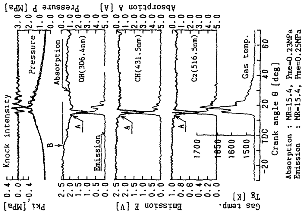
Fig.5 Abnormal combustion with n-heptane (0 RON)
