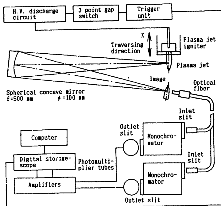
Fig.3 Schematic of local electron temperature measurement system by the two-line radiance ratio method. The apparatus can measure intensities of two different wavelength at a point simultaneously.
