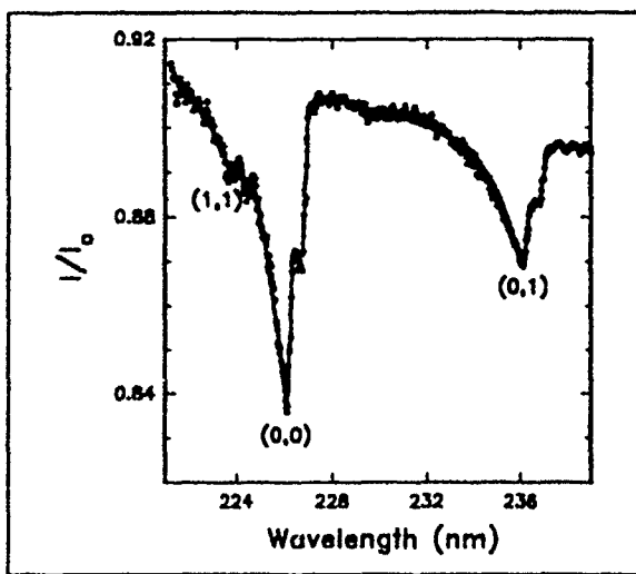
NO Absorption from lean \text{CH}_4/\text{N}_2\text{O} Flame.
