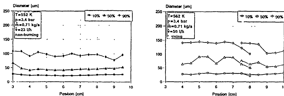
Figure 2: Characteristic diameters with regard to the volume distribution
