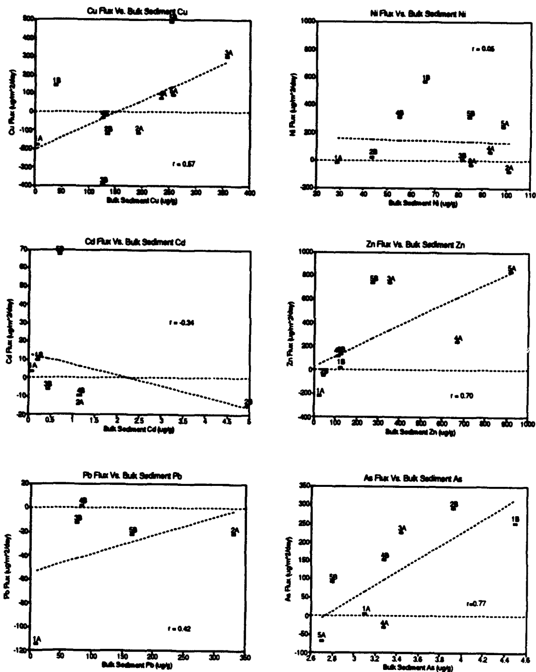
Figure 56. Correlations for trace metal flux rates and bulk sediment metal concentrations.
