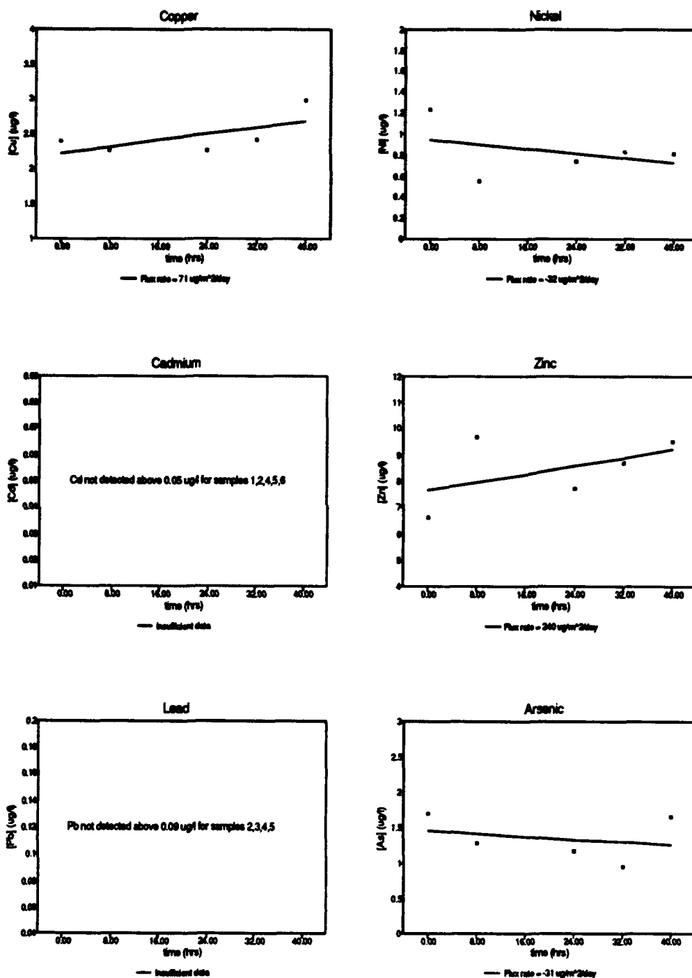
Figure 35. Time-series chamber samples and flux rates at site 4A based on a linear regression over the sampling period. Data not used in the regression are indicated by \blacktriangle (see table 4).
