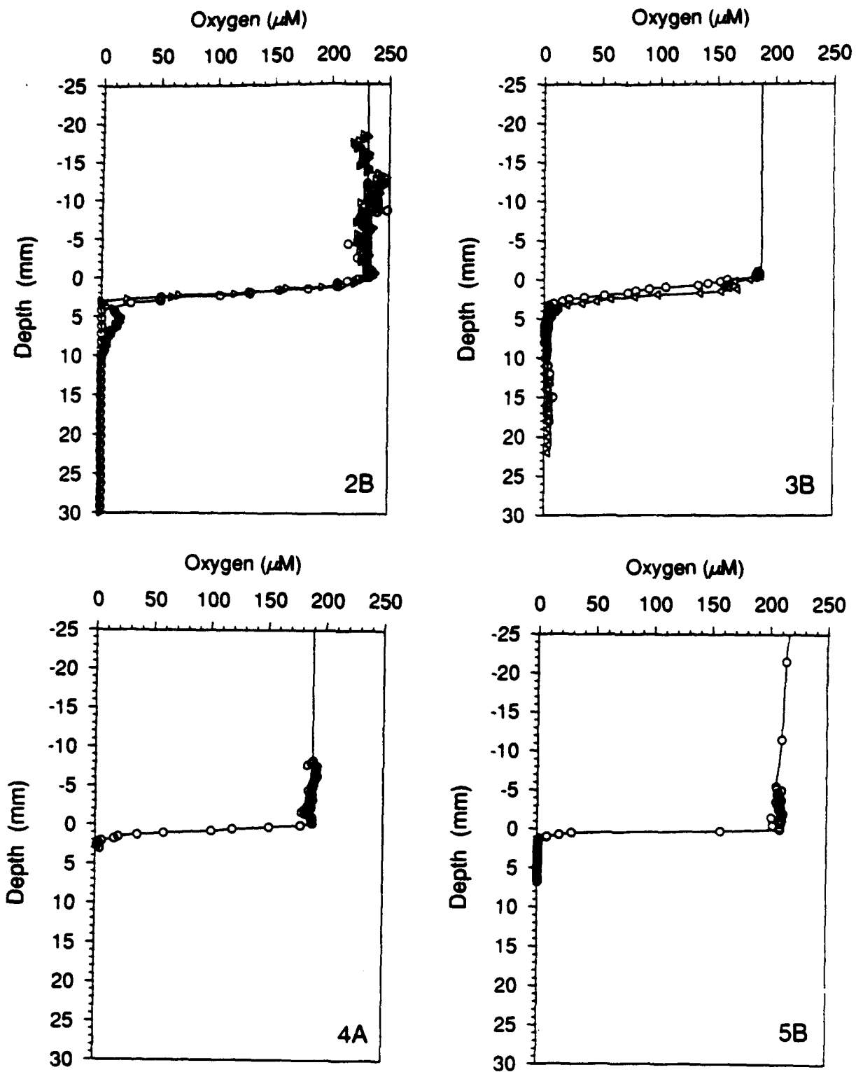
Fig. 2. Oxygen microprofiles from Sinclair Inlet. Many profiles do not extend very far into the sediment because the microelectrodes were broken by the coarse sand or debris.
