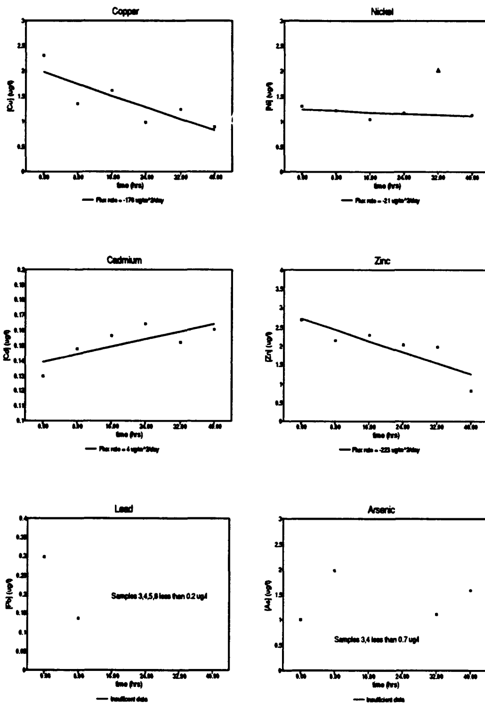
Figure 29. Time-series chamber samples and flux rates at site 1A based on a linear regression over the sampling period. Data not used in the regression are indicated by \Delta (see table 4).
