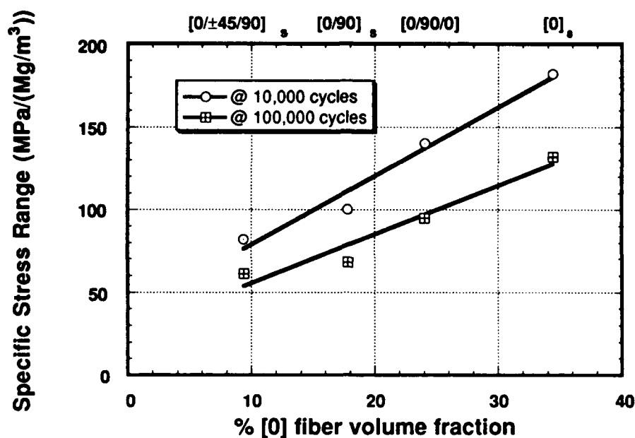
Fig. 15. SCS-6/TIMETAL®21S fatigue stress range versus volume fraction of [0] fibers.
