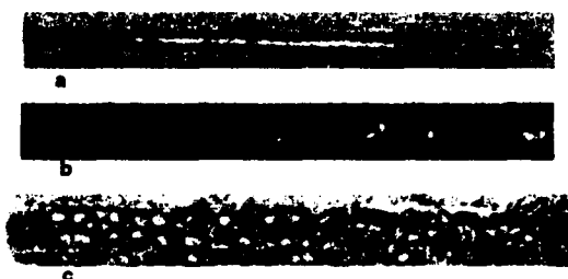
Figure 2 (a) Image of Single Fiber embedded in Homogenous Ti-6Al-4V Matrix with fine equiaxed \alpha + \beta microstructure. (b) Single Fiber Image in Ti-6Al-4V Single Fiber. (c) Ti-6-4 Three Fibers.
