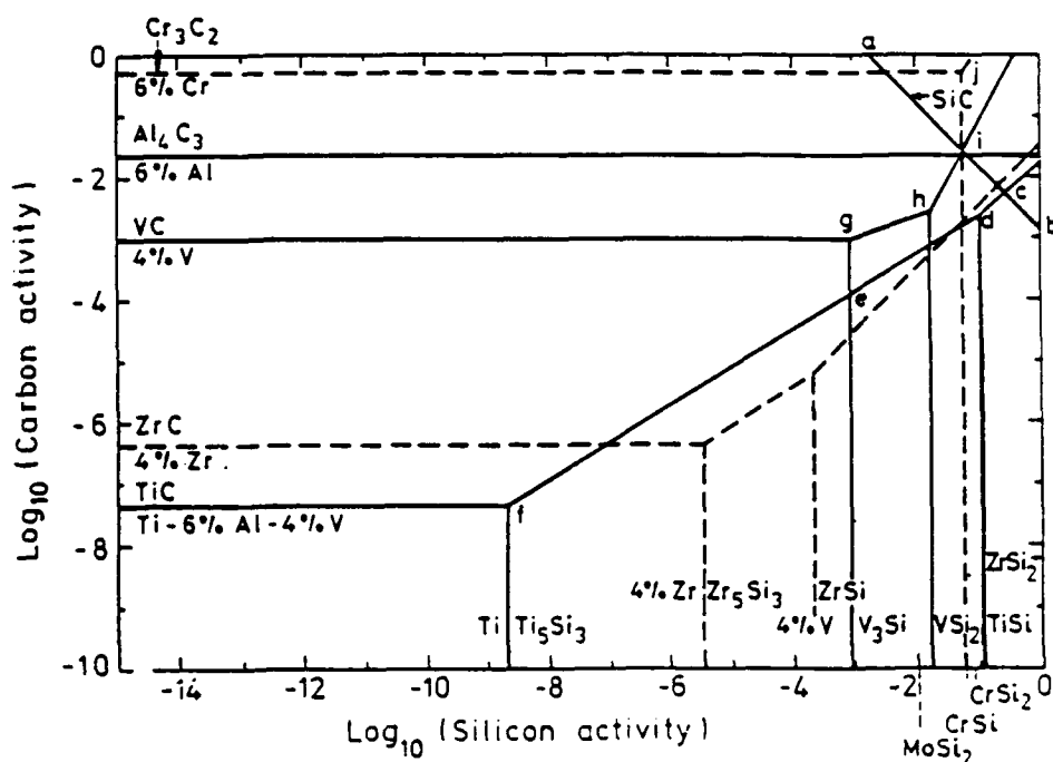
Fig 3. Predominance area diagram for carbides and silicides in Ti alloys at 1200K (Ref. 5)
