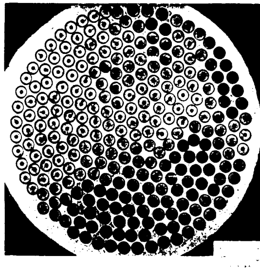
Fig.2 SiC-Ti6Al4V- composite with a fibre volume fraction of 0.57 (inside the reinforced region)
