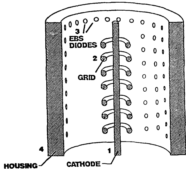
Figure 4. 100-kW EBS amplifier cross section diagram.
