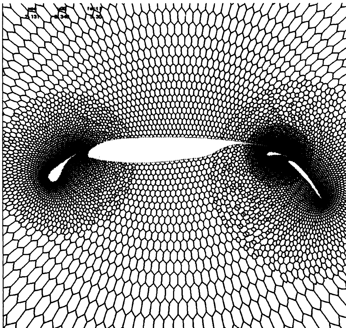
Figure 6: Dual to the fine grid having 11340 vertices about a 4-element airfoil.
