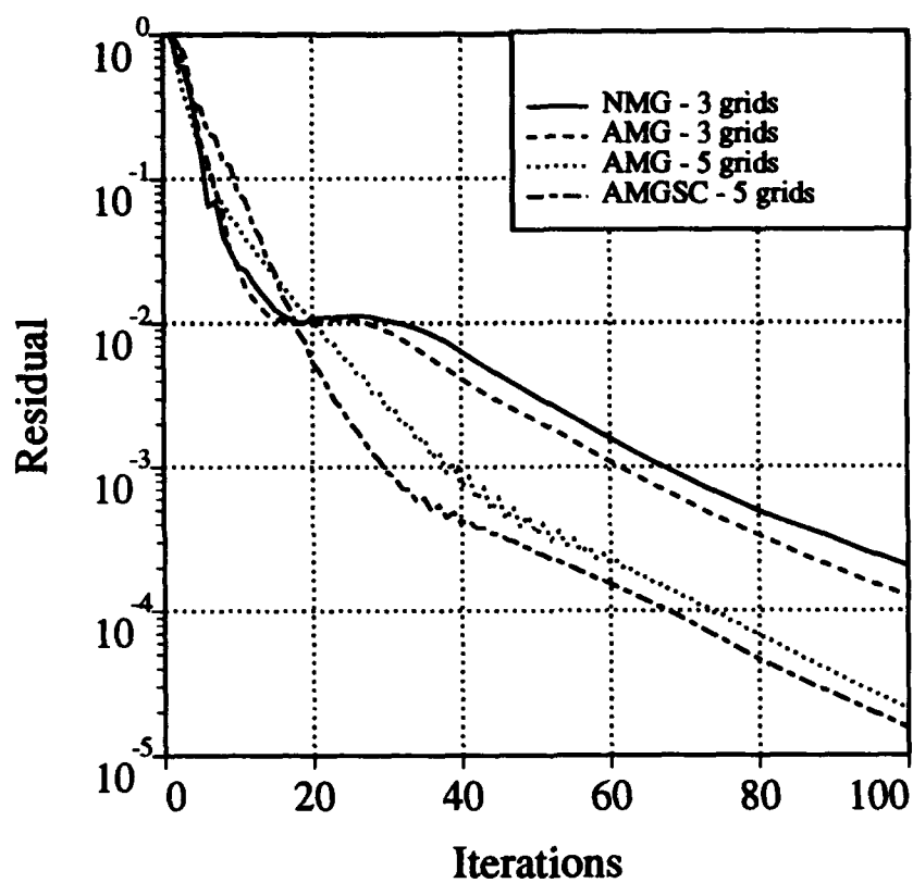
Figure 8: Convergence histories with the agglomerated and original multigrid. NMG – Non-nested multigrid; AMG – Agglomerated multigrid using the isotropic algorithm; AMGSC – Agglomerated multigrid using the semi-coarsened algorithm.
