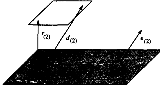
Figure 27: In the method of Conjugate Gradients, each new residual is orthogonal to all the previous residuals and search directions; and each new search direction is constructed (from the residual) to be A -orthogonal to all the previous residuals and search directions. The endpoints of r_{(2)} and d_{(2)} lie on a plane parallel to the shaded subspace. In CG, d_{(2)} is a linear combination of r_{(2)} and d_{(1)} .
