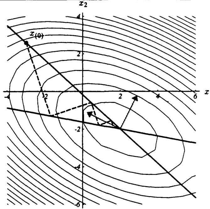
Figure 19: Solid lines represent the starting points that give the worst convergence for Steepest Descent. Dashed lines represent steps toward convergence. Note that if the first iteration starts from a worst-case point, so do all succeeding iterations. Each step taken intersects the paraboloid axes (grey arrows) at precisely a 45^\circ angle. Here, \kappa = 3.5 .
