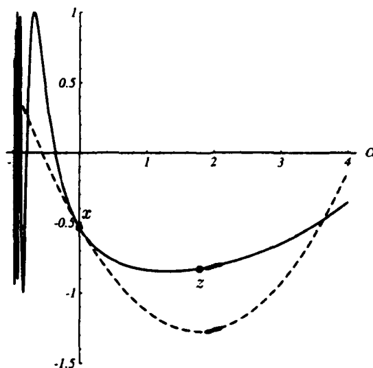
Figure 39: The Secant method for minimizing a one-dimensional function (solid curve). Starting from the point x , calculate the first derivatives at two different points (here, \alpha = 0 and \alpha = 2 ), and use them to construct a quadratic approximation to the function (dashed curve). Notice that both curves have the same slope at \alpha = 0 , and also at \alpha = 2 . As in the Newton-Raphson method, a new point z is chosen at the base of the parabola, and the procedure is iterated until convergence.
