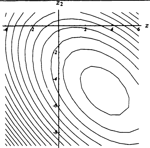
Figure 35: Contour lines of the quadratic form of the diagonally preconditioned sample problem.
