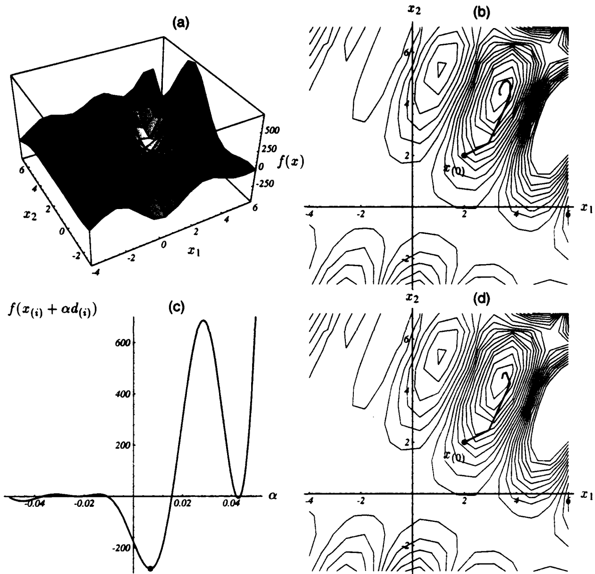
Figure 36: Convergence of the nonlinear Conjugate Gradient Method. (a) A complicated function with many local minima and maxima. (b) Convergence path of Fletcher-Reeves CG. Unlike linear CG, convergence does not occur in two steps. (c) Cross-section of the surface corresponding to the first line search. (d) Convergence path of Polak-Ribière CG.
