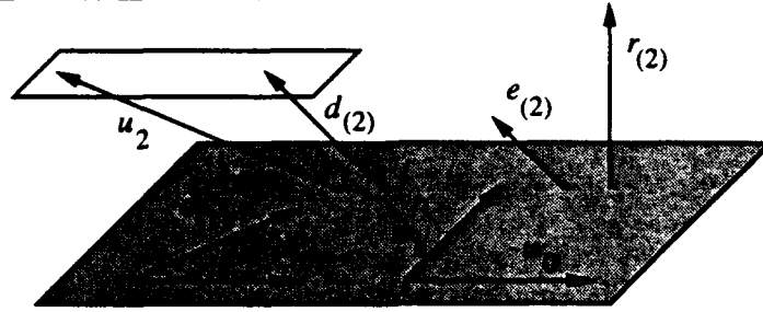
Figure 26: Because the search directions d_{(0)}, d_{(1)} are constructed from the vectors u_0, u_1 , they span the same subspace (the grey-colored plane). The error term e_{(2)} is A -orthogonal to this subspace, the residual r_{(2)} is orthogonal to this subspace, and a new search direction d_{(2)} is constructed (from u_2 ) to be A -orthogonal to this subspace. The endpoints of u_2 and d_{(2)} lie on a plane parallel to the shaded subspace, because d_{(2)} is constructed from u_2 by Gram-Schmidt conjugation.
