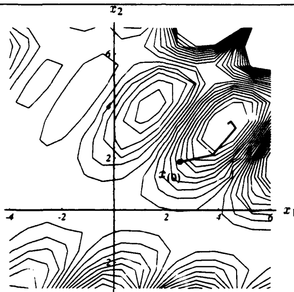
Figure 40: The preconditioned nonlinear Conjugate Gradient Method, using the Polak-Ribière formula and a diagonal preconditioner. The space has been “stretched” to show the improvement in circularity of the contour lines around the minimum.
