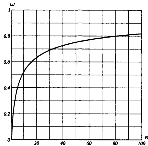
Figure 33: Convergence of Conjugate Gradients (per iteration) as a function of condition number. Compare with Figure 20.
