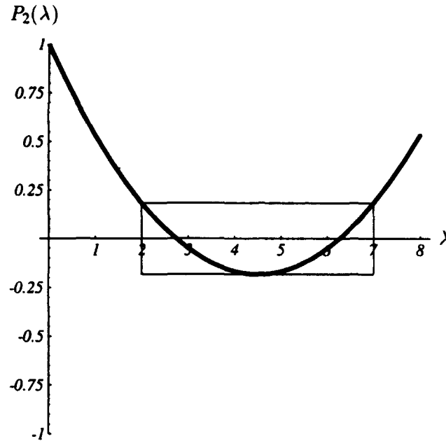
Figure 32: The polynomial P_2(\lambda) that minimizes Equation 49 for \lambda_{min} = 2 and \lambda_{max} = 7 in the general case. This curve is a scaled version of the Chebyshev polynomial of degree 2. The energy norm of the error term after two iterations is no greater than 0.183 times its initial value. Compare with Figure 30(c), where it is known that there are only two eigenvalues.
