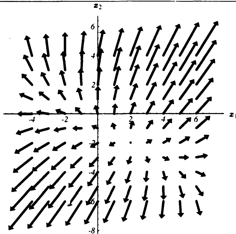
Figure 4: Gradient f'(\mathbf{x}) of the quadratic form. For every \mathbf{x} , the gradient points in the direction of steepest increase of f(\mathbf{x}) , and is orthogonal to the contour lines.
