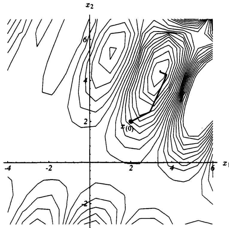
Figure 37: Nonlinear CG can be more effective with periodic restarts.
