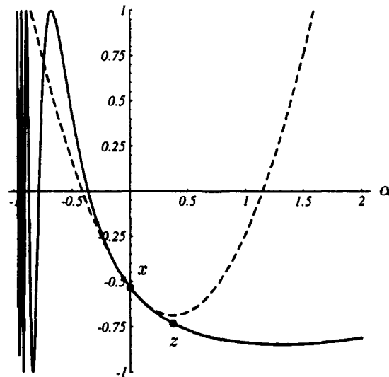
Figure 38: The Newton-Raphson method for minimizing a one-dimensional function (solid curve). Starting from the point x , calculate the first and second derivatives, and use them to construct a quadratic approximation to the function (dashed curve). A new point z is chosen at the base of the parabola. This procedure is iterated until convergence is reached.
