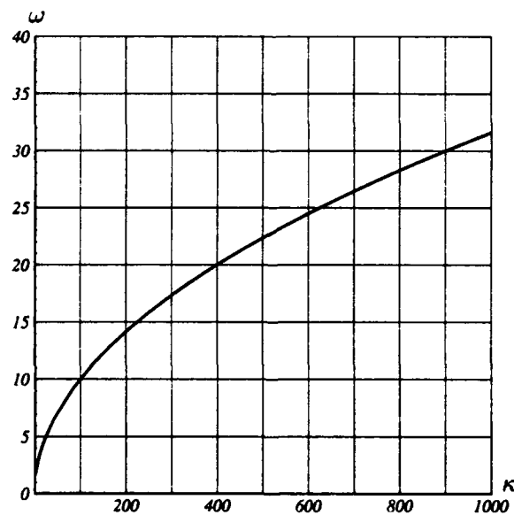
Figure 34: Number of iterations of Steepest Descent required to match one iteration of CG.
