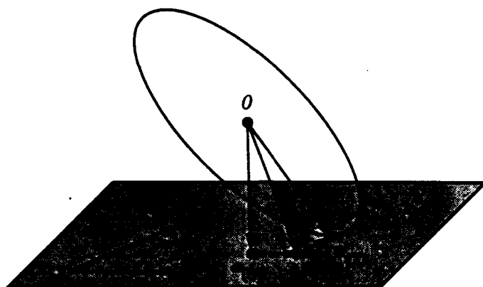
Figure 29: In this figure, the shaded area is \mathcal{E} = e_{(0)} + \text{span}\{d_{(0)}, d_{(1)}\} . The ellipsoid is a contour on which the energy norm is constant. After two steps, CG finds e_{(2)} , the point on \mathcal{E} which minimizes \|e\|_A .
