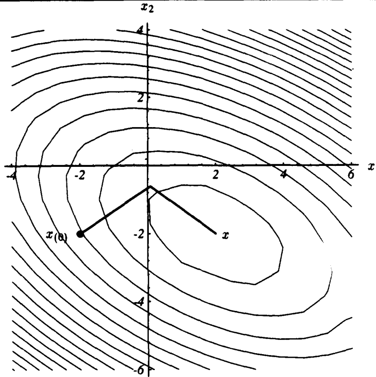
Figure 28: The method of Conjugate Gradients.
