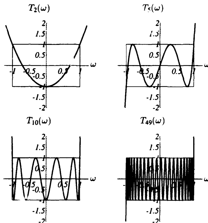
Figure 31: Chebyshev polynomials of degree 2, 5, 10, and 49.
