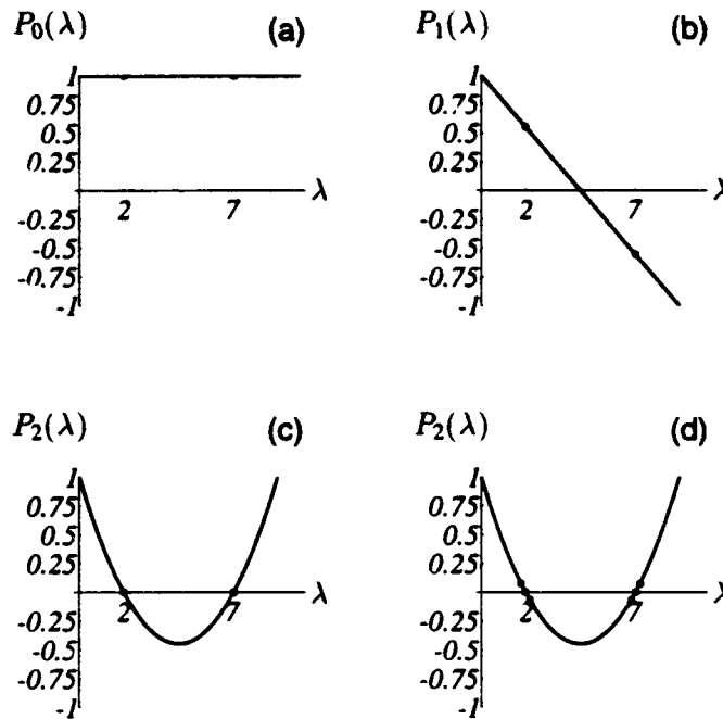
Figure 30: The convergence of CG after i iterations depends on how close a polynomial P_i of degree i can be to zero on each eigenvalue, given the constraint that P_i(0) = 1 .
