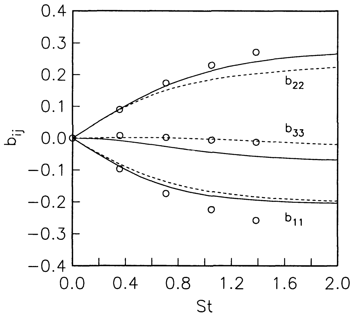
Figure 5. Time evolution for the anisotropy tensor in plane strain for \epsilon_0/Sk_0 = 2.0 . The predictions of the 2DMFI model ———, the SL model ----, and the direct numerical simulations of Lee and Reynolds (1985).
