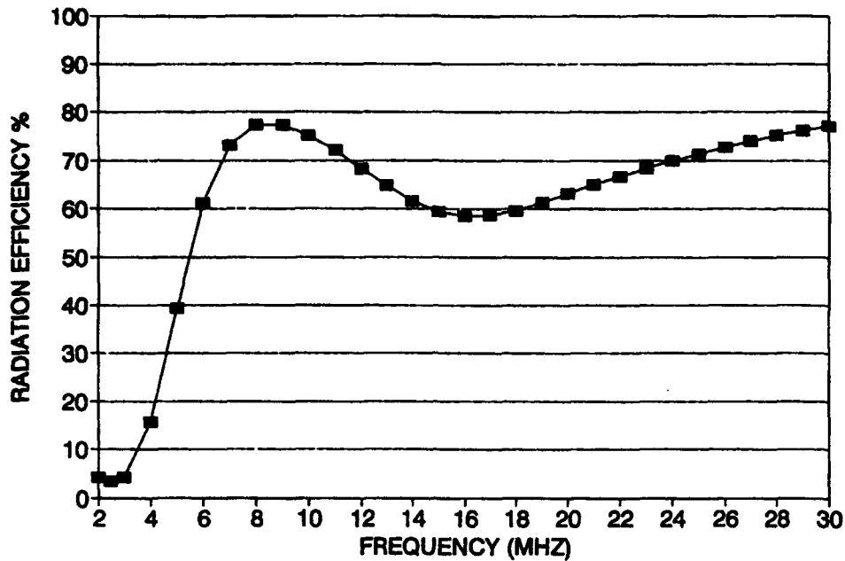
Figure 17. Radiation efficiency of final 11.6-meter, twin-loaded, twin-whip antenna.
