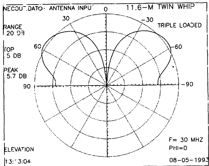
Figure 43. Vertical radiation patterns (calculated) for 11.6-meter, triple-loaded, twin-whip antenna at 30 MHz.
