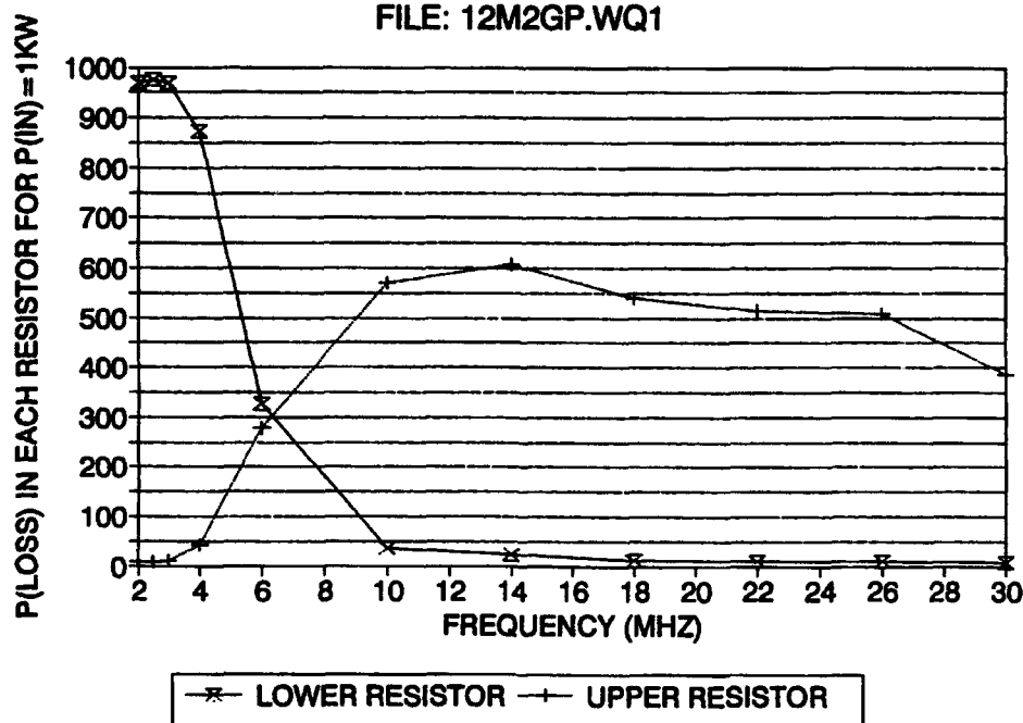
Figure 7. Power dissipation in each loading resistor with 1 kW input to antenna for redesigned 12-meter, twin-loaded, single-whip antenna.
