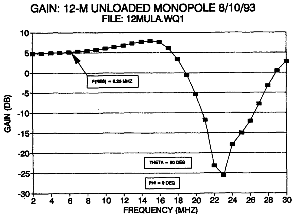
Figure 50. Gain versus frequency in horizontal plane for 12-meter, unloaded, monopole antenna.
