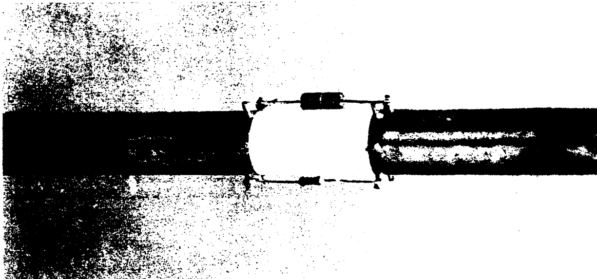
Figure 57. Photograph of 1/10-scale model of 11.6-meter, twin-loaded, twin-whip antenna loading elements and teflon insulator.
