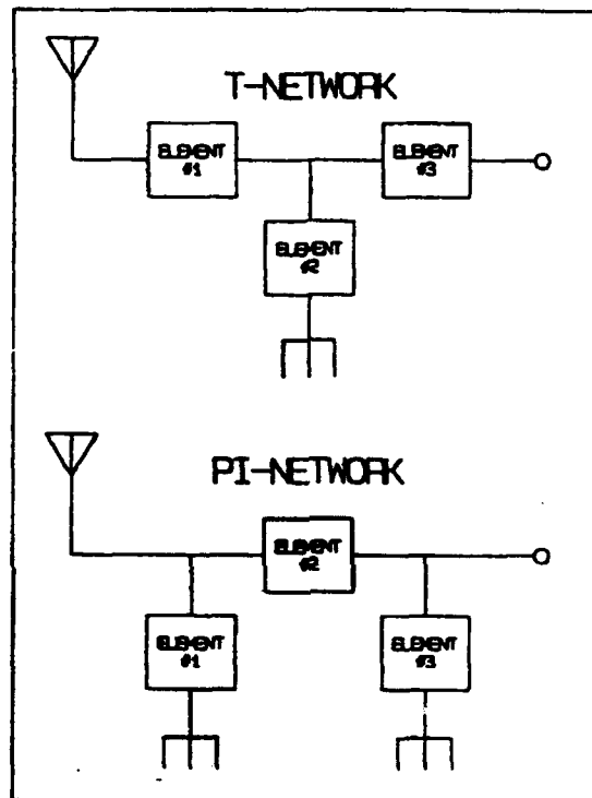
Figure 1. T-network and Pi-network diagram.
