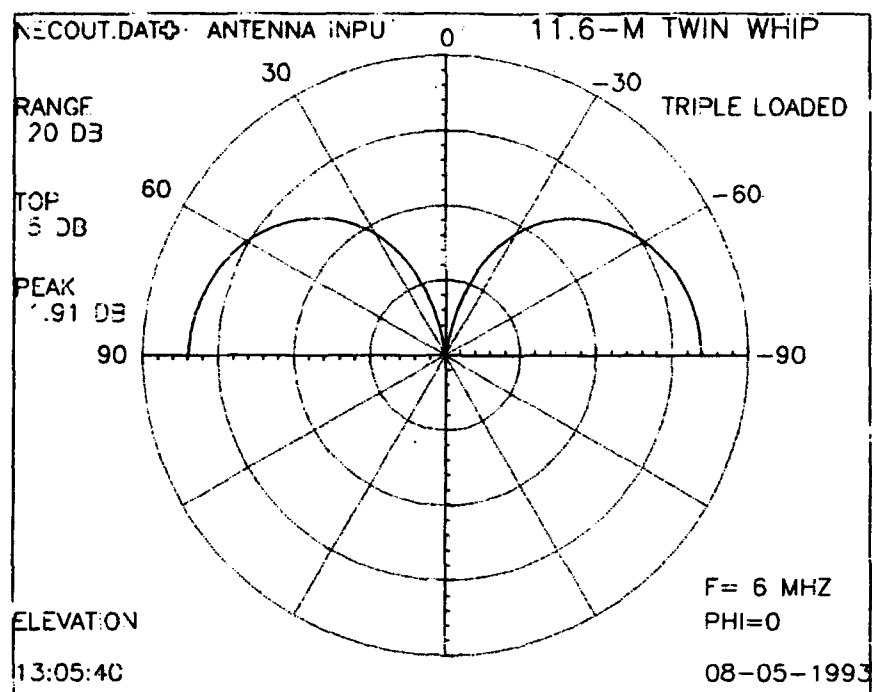
Figure 40. Vertical radiation patterns (calculated) for 11.6-meter, triple-loaded, twin-whip antenna at 6 MHz.
