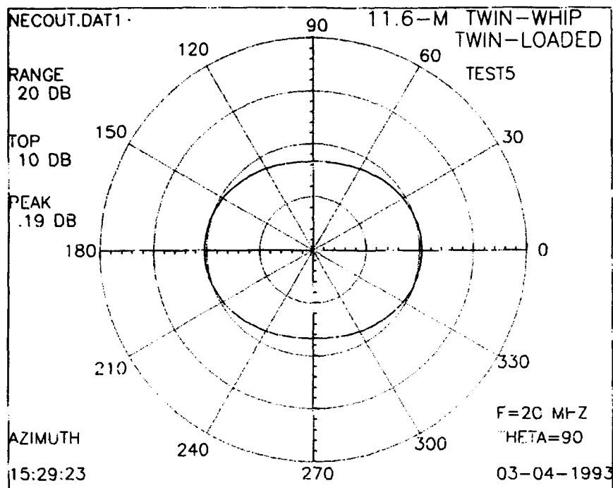
Figure 36. Horizontal radiation patterns (calculated) for 11.6-meter, twin-loaded, twin-whip antenna at 20 MHz.
