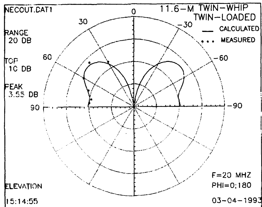
Figure 68. Vertical radiation patterns (calculated and measured) for 11.6-meter, twin-loaded, twin-whip, 1/10-scale model antenna at 20 MHz.
