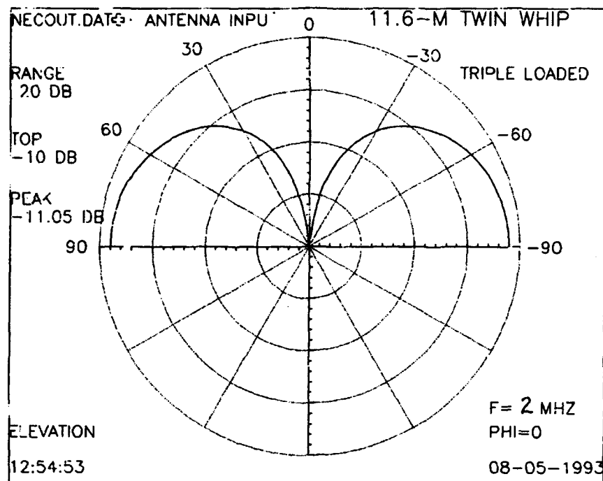
Figure 38. Vertical radiation patterns (calculated) for 11.6-meter, triple-loaded, twin-whip antenna at 2 MHz.
