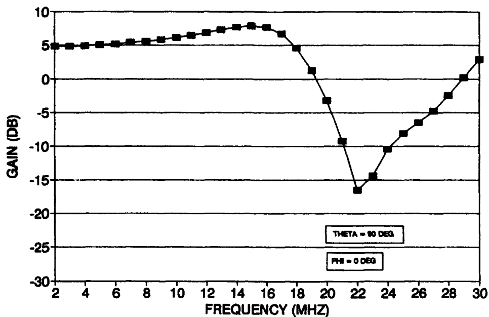
Figure 51. Gain versus frequency in horizontal plane for 11.6-meter, unloaded, twin-whip antenna.
