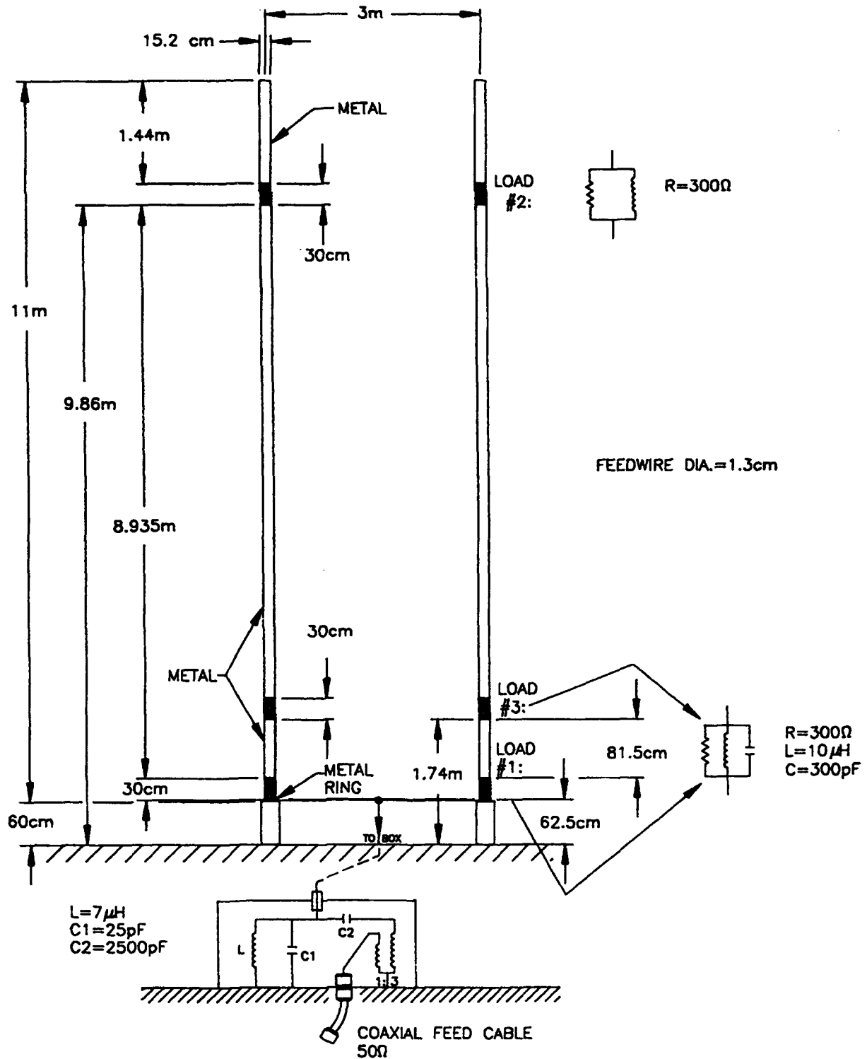
Figure 19. Drawing of final 11.6-meter, triple-loaded, twin-whip antenna design.
