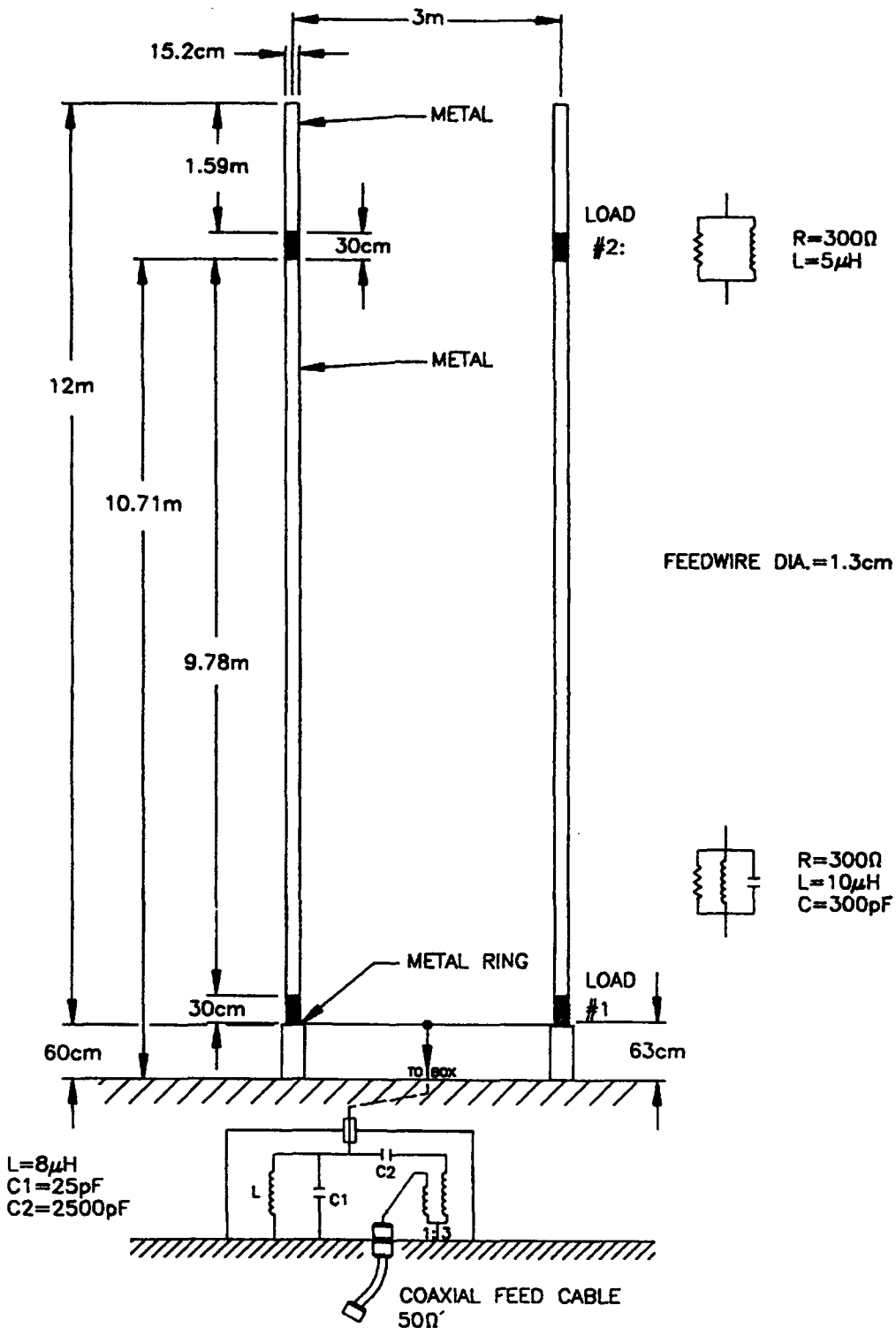
Figure 8. Drawing of final 12.6-meter, twin-loaded, twin-whip antenna design.
