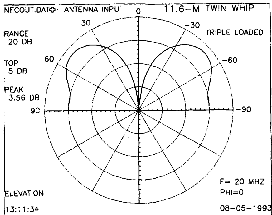
Figure 42. Vertical radiation patterns (calculated) for 11.6-meter, triple-loaded, twin-whip antenna at 20 MHz.
