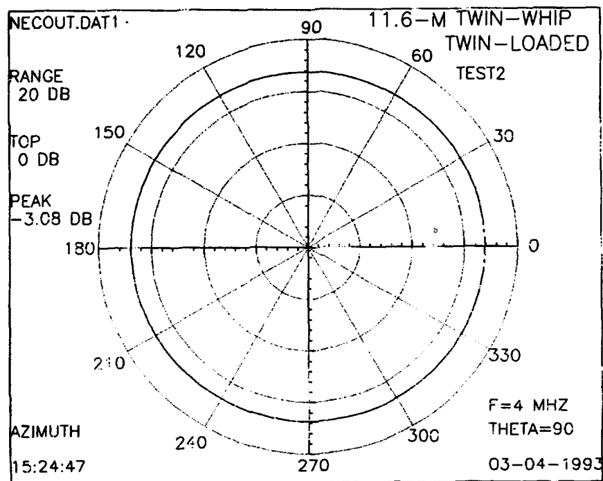
Figure 33. Horizontal radiation patterns (calculated) for 11.6-meter, twin-loaded, twin-whip antenna at 4 MHz.
