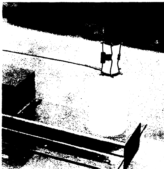
Figure 56. Photograph of 1/10-scale model of 11.6-meter, twin-loaded, twin-whip antenna, bottom section view.
