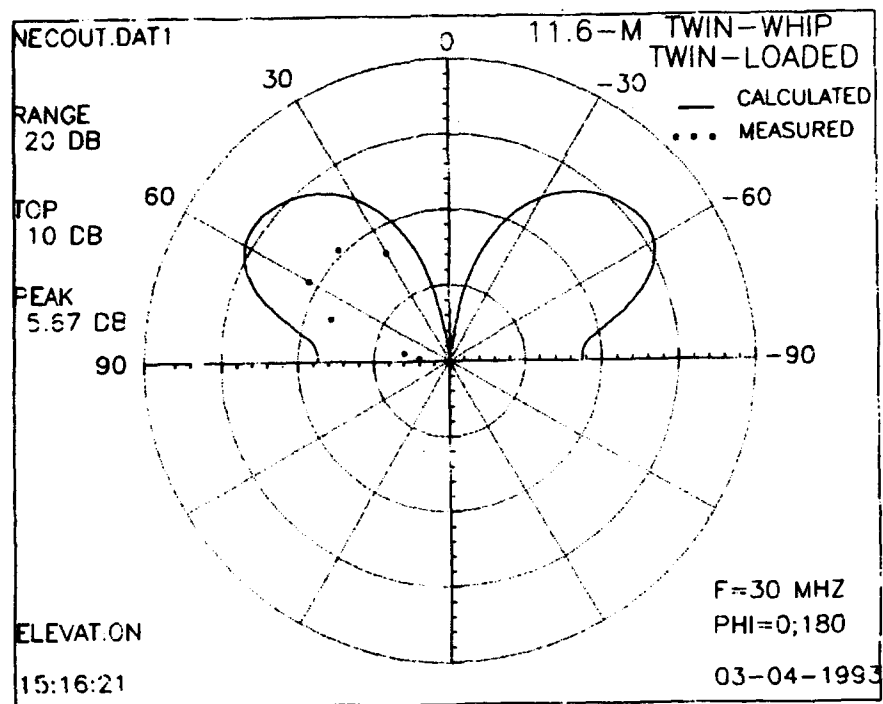
Figure 69. Vertical radiation patterns (calculated and measured) for 11.6-meter, twin-loaded, twin-whip, 1/10-scale model antenna at 30 MHz.
