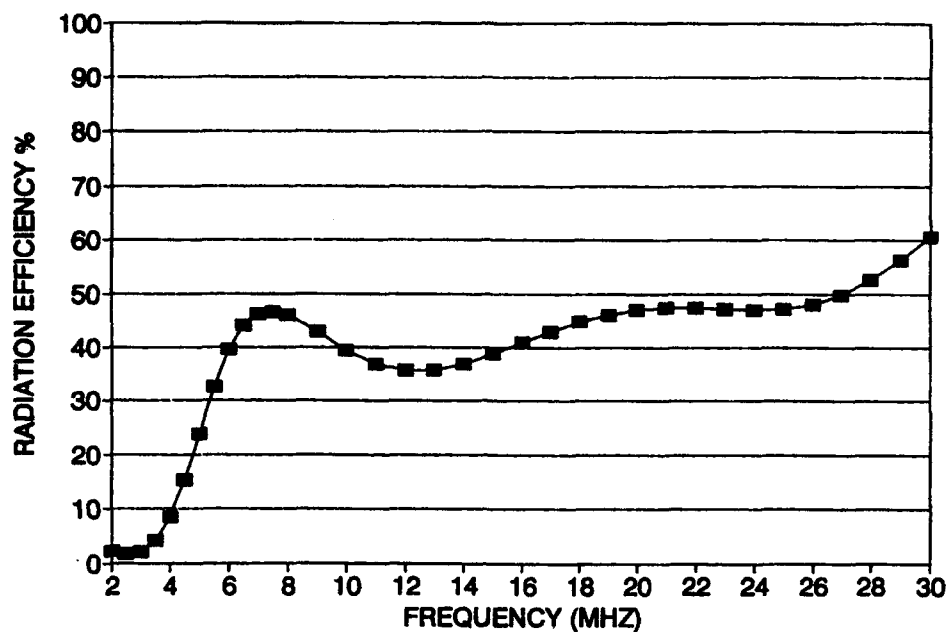
Figure 6. Radiation efficiency of redesigned 12-meter, twin-loaded, single-whip antenna.
