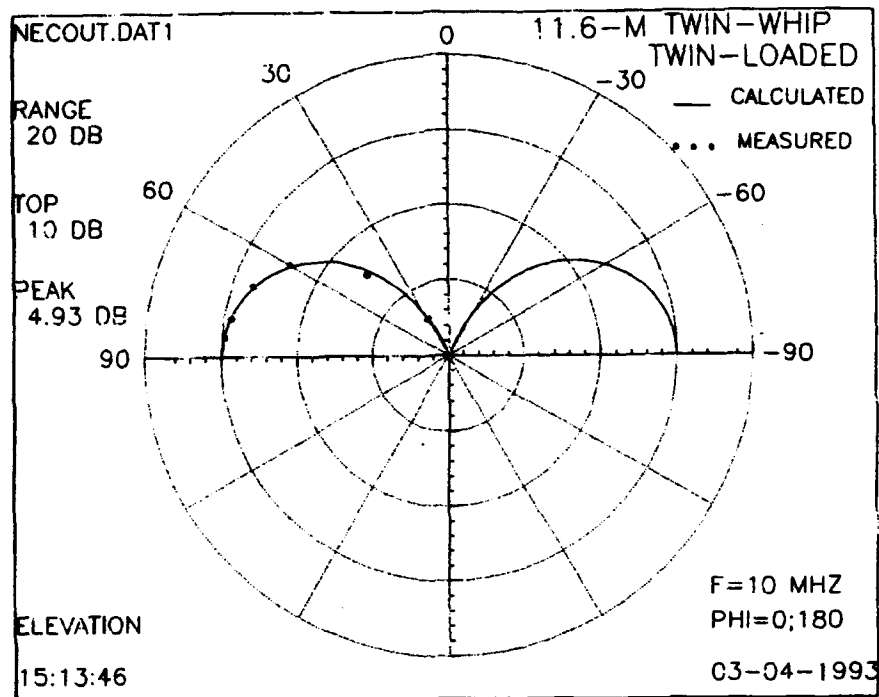
Figure 67. Vertical radiation patterns (calculated and measured) for 11.6-meter, twin-loaded, twin-whip, 1/10-scale model antenna at 10 MHz.
