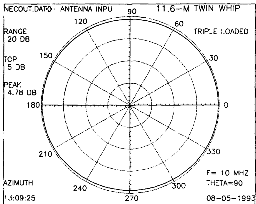
Figure 47. Horizontal radiation patterns (calculated) for 11.6-meter, triple-loaded, twin-whip antenna at 10 MHz.
