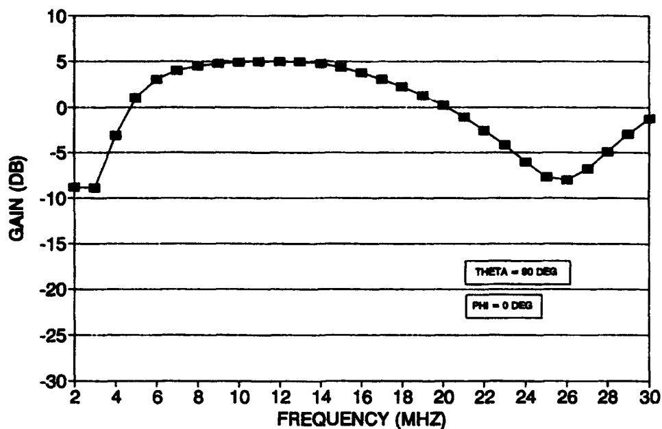
Figure 53. Gain versus frequency in horizontal plane for 11.6-meter, twin-loaded, twin-whip antenna.
