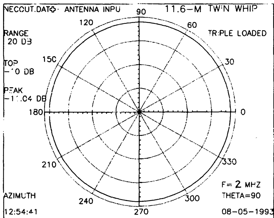
Figure 44. Horizontal radiation patterns (calculated) for 11.6-meter, triple-loaded, twin-whip antenna at 2 MHz.
