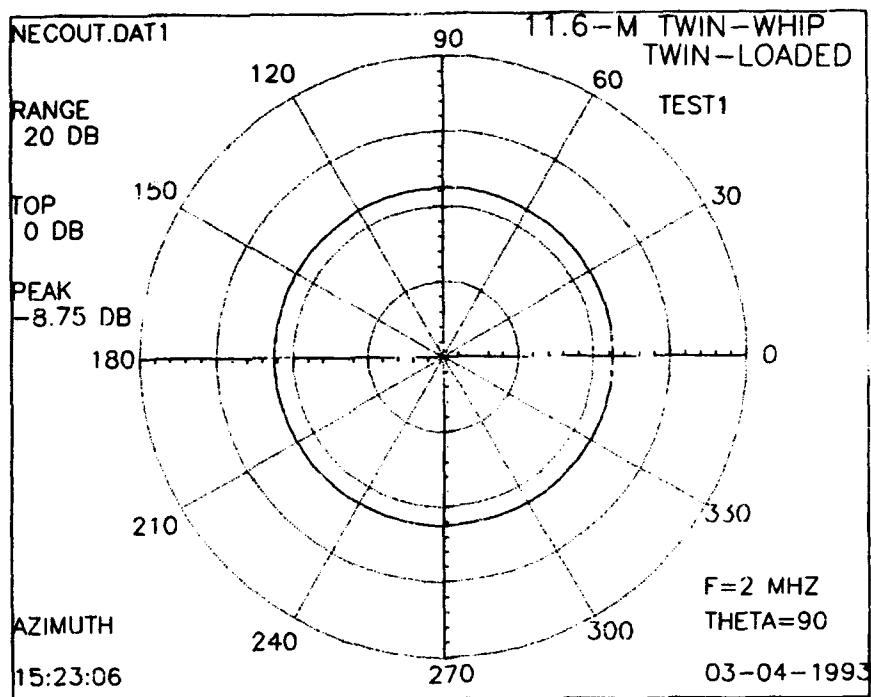
Figure 32. Horizontal radiation patterns (calculated) for 11.6-meter, twin-loaded, twin-whip antenna at 2 MHz.
