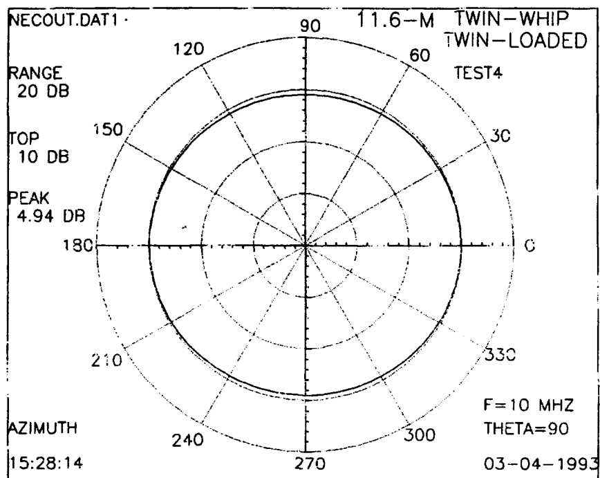
Figure 35. Horizontal radiation patterns (calculated) for 11.6-meter, twin-loaded, twin-whip antenna at 10 MHz.
