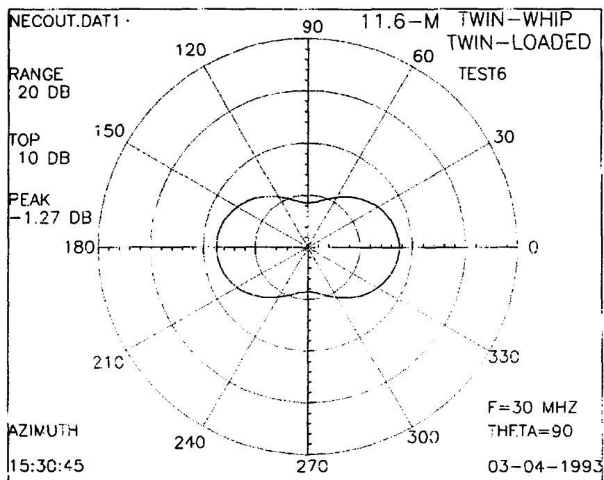
Figure 37. Horizontal radiation patterns (calculated) for 11.6-meter, twin-loaded, twin-whip antenna at 30 MHz.
