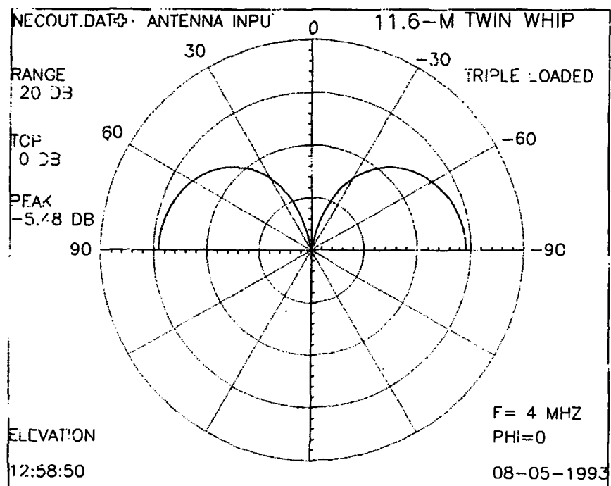
Figure 39. Vertical radiation patterns (calculated) for 11.6-meter, triple-loaded, twin-whip antenna at 4 MHz.
