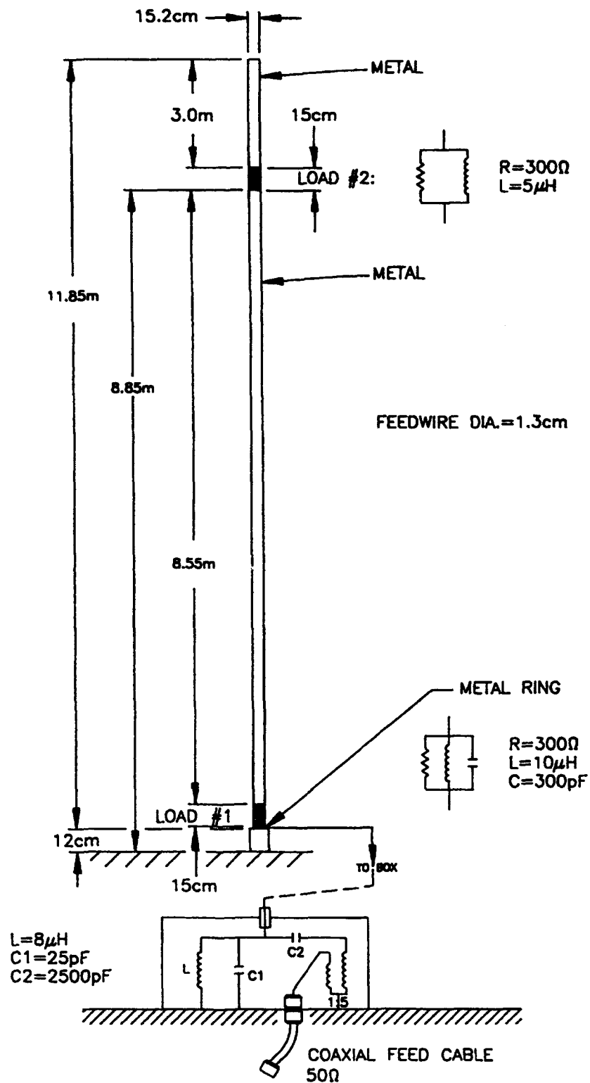
Figure 4. Drawing of 12-meter, twin-loaded, single-whip antenna redesigned to cover 2-30 MHz.
