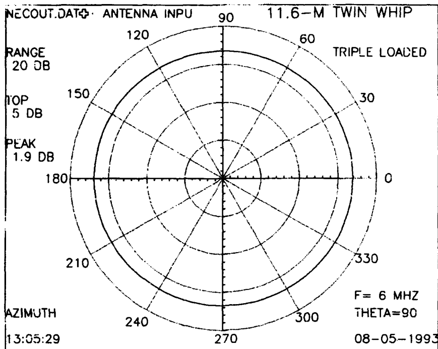
Figure 46. Horizontal radiation patterns (calculated) for 11.6-meter, triple-loaded, twin-whip antenna at 6 MHz.
