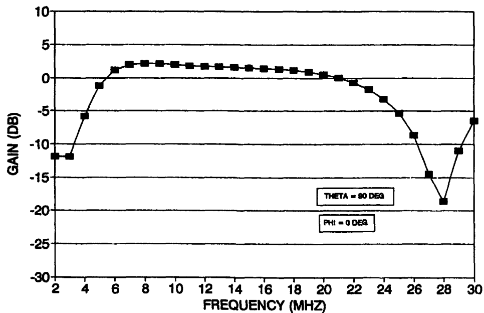
Figure 52. Gain versus frequency in horizontal plane for 12-meter, twin-loaded, single-whip antenna.
