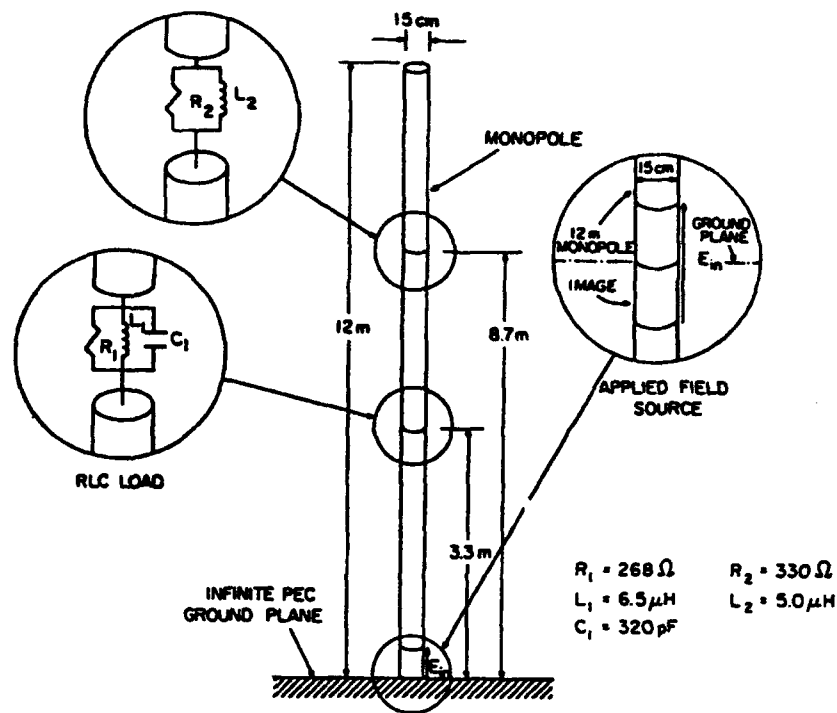
Figure 2. Drawing of Halpern and Mittra 12-meter, twin-loaded, single-whip antenna, reprinted from reference 1.
