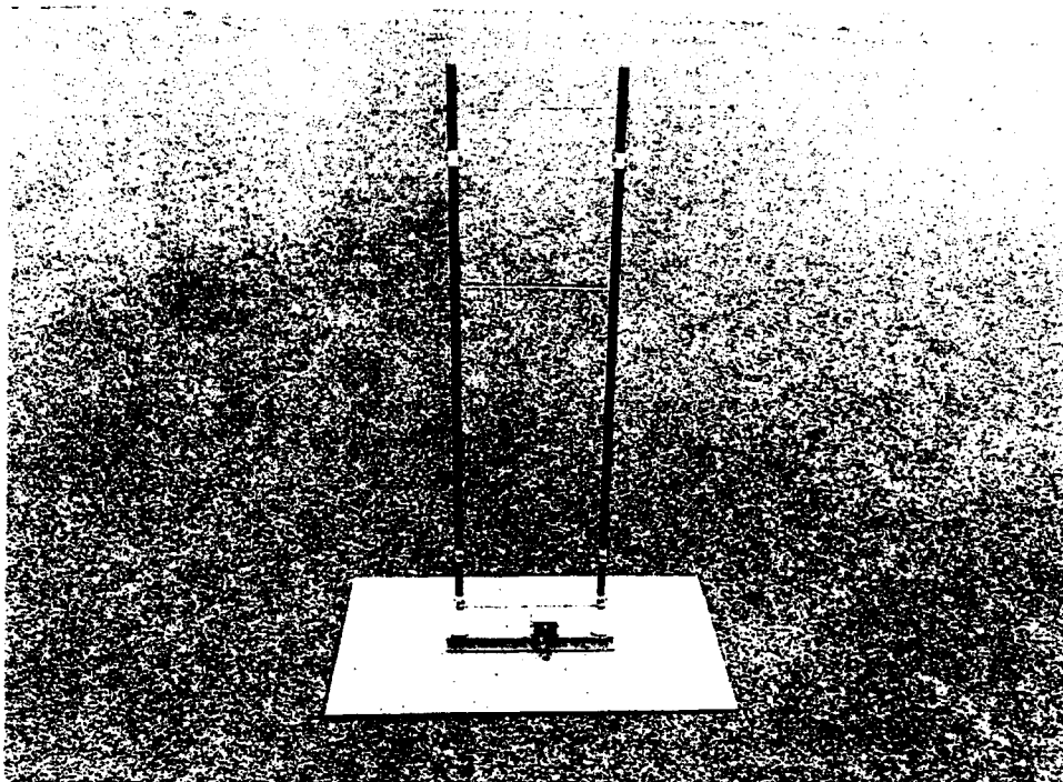
Figure 59. Photograph of 1/10-scale of 11.6-meter, triple-loaded, twin-whip antenna, full view.
