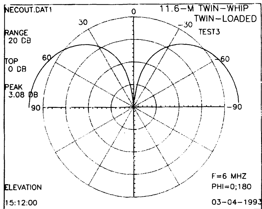
Figure 28. Vertical radiation patterns (calculated) for 11.6-meter, twin-loaded, twin-whip antenna at 6 MHz.
