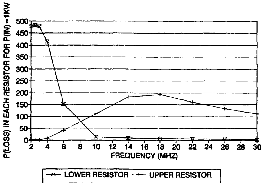
Figure 18. Power dissipation in each loading resistor with 1 kW input to antenna for 11.6-meter, twin-loaded, twin-whip antenna.
