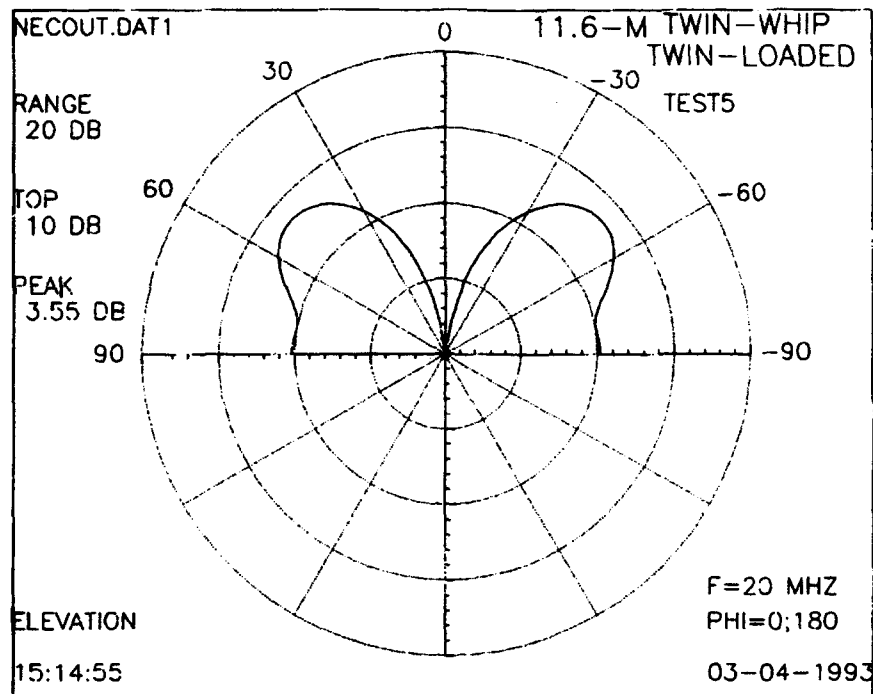
Figure 30. Vertical radiation patterns (calculated) for 11.6-meter, twin-loaded, twin-whip antenna at 20 MHz.
