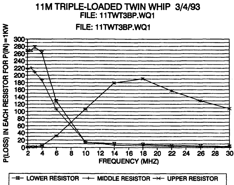
Figure 24. Power dissipation in each loading resistor with 1-kW input to antenna for 11.6-meter, triple-loaded, twin-whip antenna.
