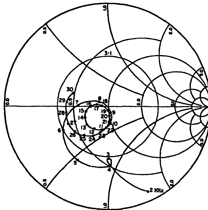
Figure 3. Impedance of Halpern and Mittra 12-meter, twin-loaded, single-whip antenna, reprinted from reference 1.
