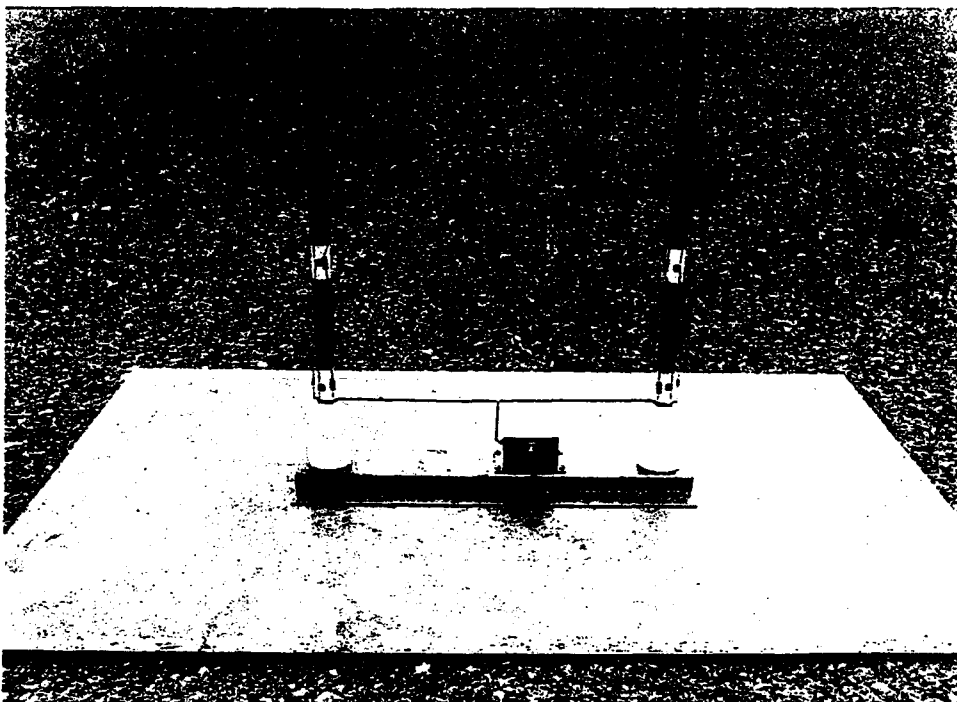
Figure 60. Photograph of 1/10-scale of 11.6-meter, triple-loaded, twin-whip antenna, lower view.
