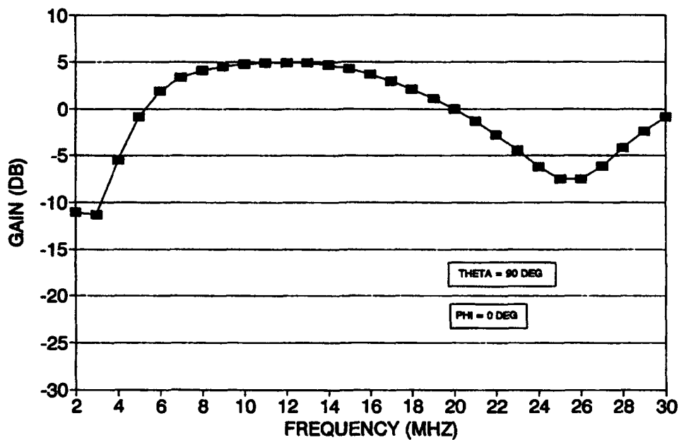
Figure 54. Gain versus frequency in horizontal plane for 11.6-meter, triple-loaded, twin-whip antenna.
