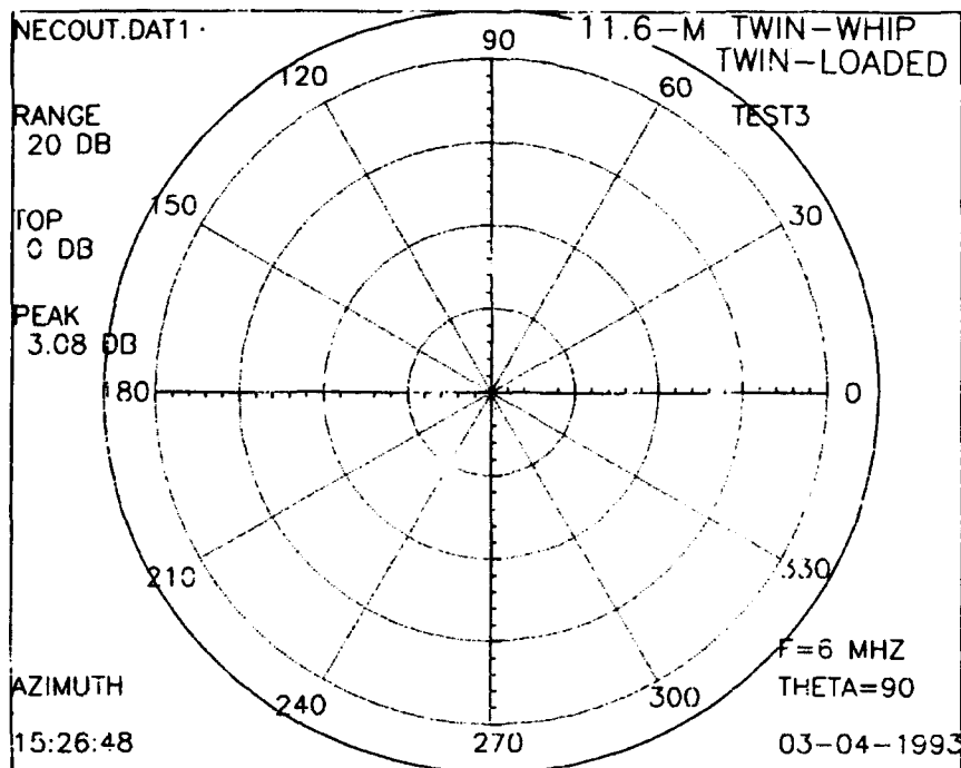
Figure 34. Horizontal radiation patterns (calculated) for 11.6-meter, twin-loaded, twin-whip antenna at 6 MHz.
