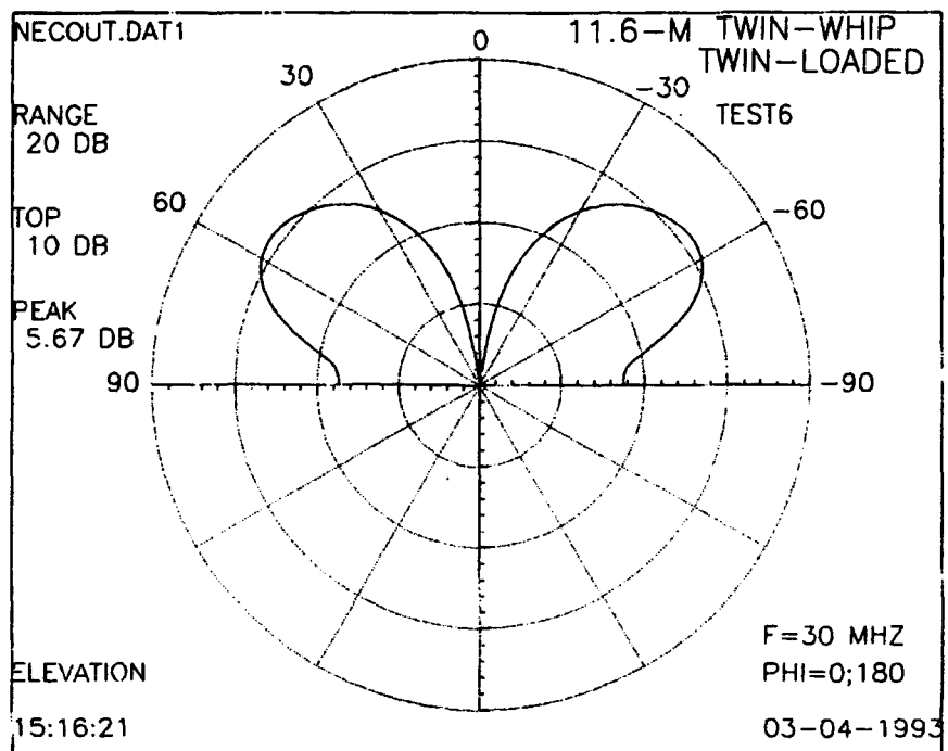
Figure 31. Vertical radiation patterns (calculated) for 11.6-meter, twin-loaded, twin-whip antenna at 30 MHz.
