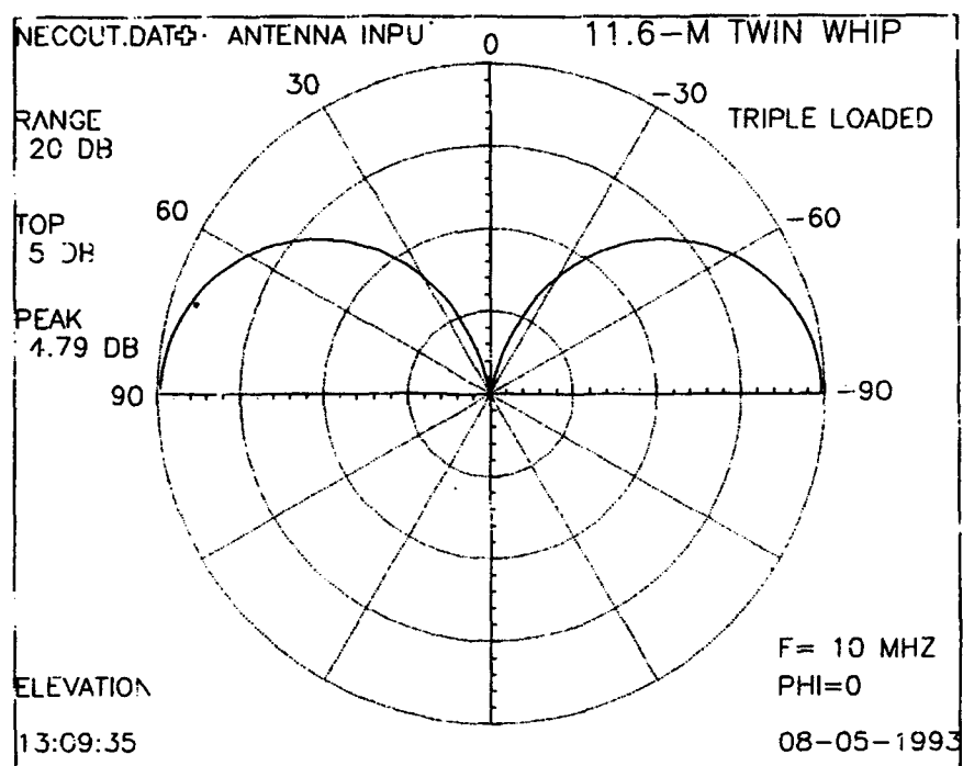
Figure 41. Vertical radiation patterns (calculated) for 11.6-meter, triple-loaded, twin-whip antenna at 10 MHz.
