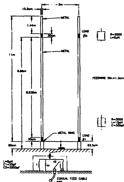
Figure 13. Drawing of final 11.6-meter, twin-loaded, twin-whip antenna design.
