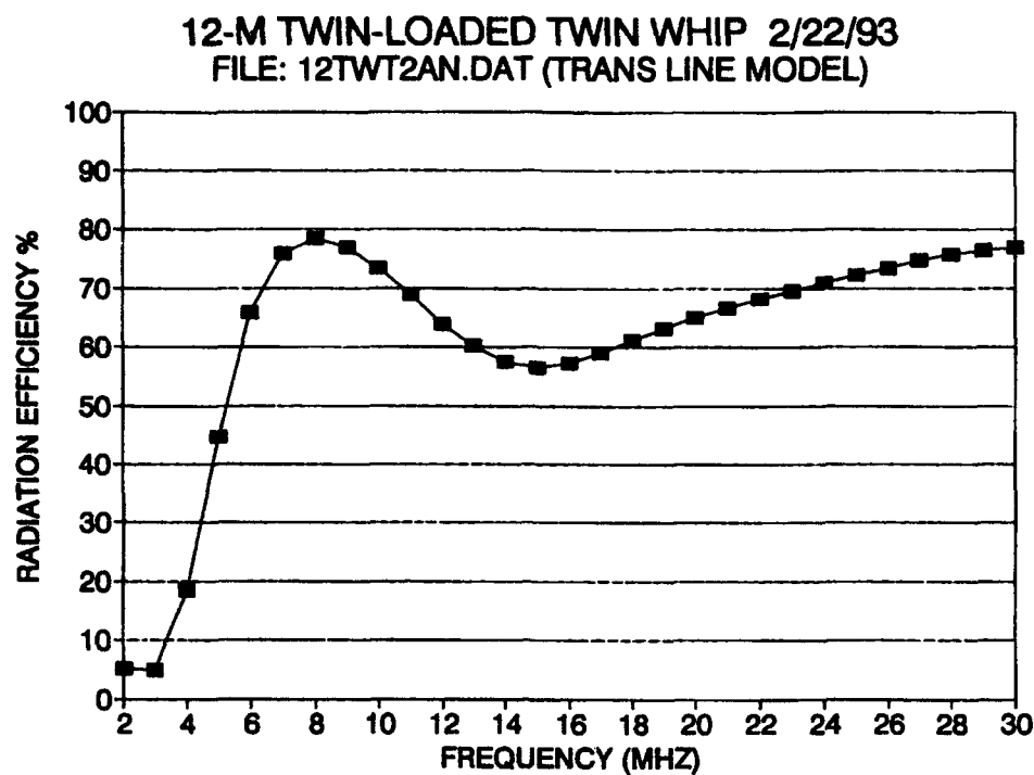
Figure 12. Radiation efficiency of final 12.6-meter, twin-loaded, twin-whip antenna.
