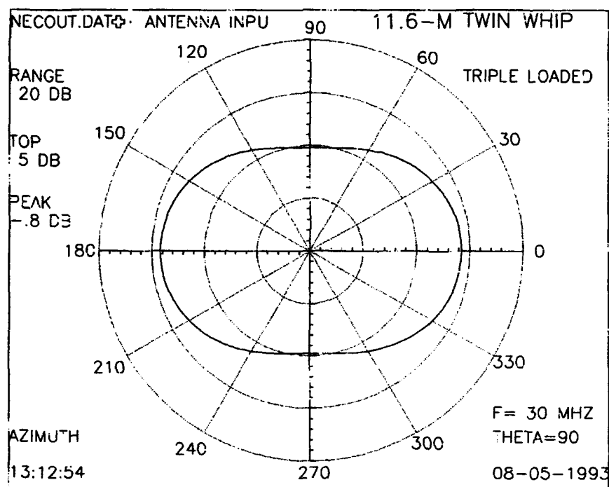
Figure 49. Horizontal radiation patterns (calculated) for 11.6-meter, triple-loaded, twin-whip antenna at 30 MHz.
