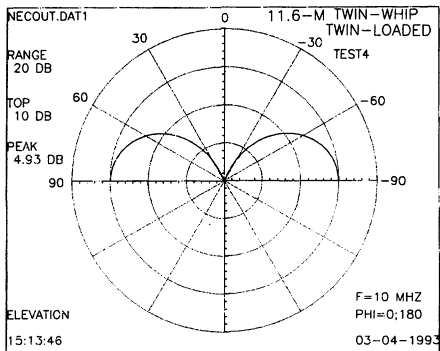
Figure 29. Vertical radiation patterns (calculated) for 11.6-meter, twin-loaded, twin-whip antenna at 10 MHz.
