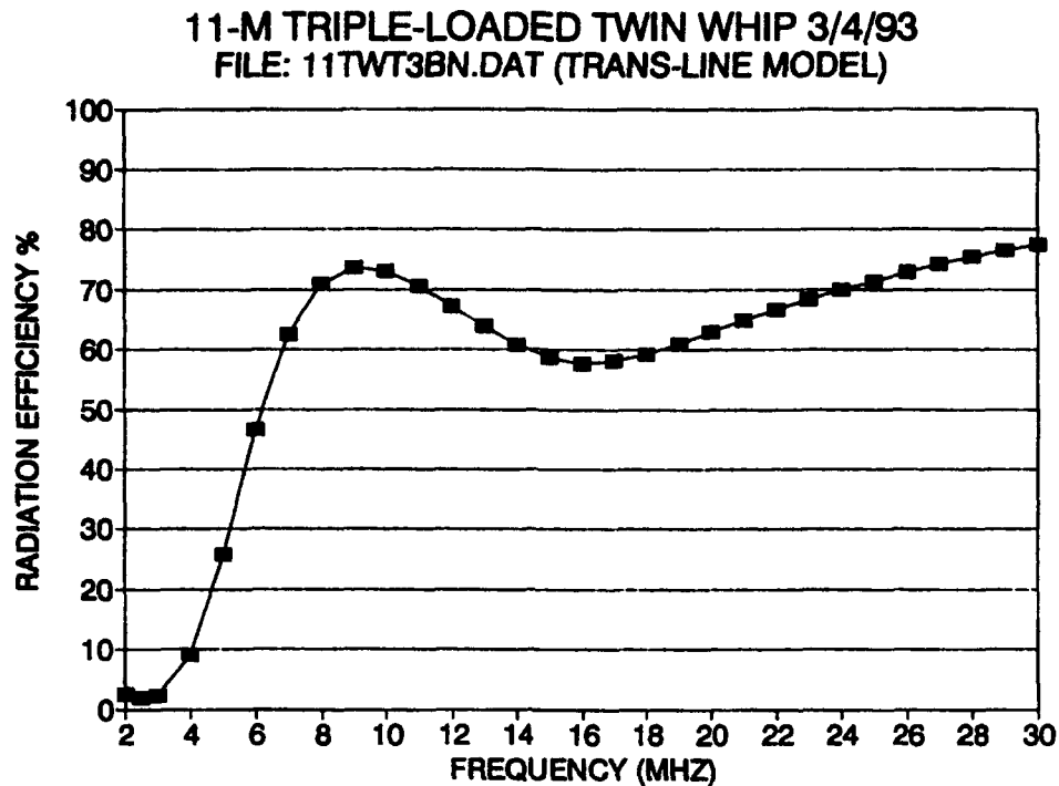
Figure 23. Radiation efficiency of final 11.6-meter, triple-loaded, twin-whip antenna.
