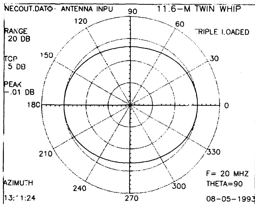
Figure 48. Horizontal radiation patterns (calculated) for 11.6-meter, triple-loaded, twin-whip antenna at 20 MHz.
