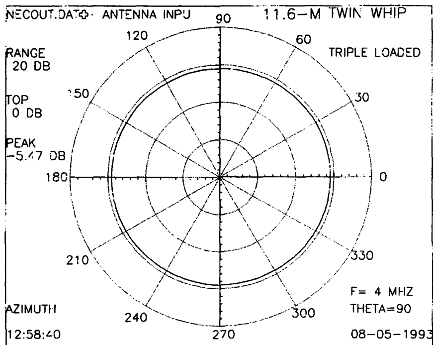
Figure 45. Horizontal radiation patterns (calculated) for 11.6-meter, triple-loaded, twin-whip antenna at 4 MHz.
