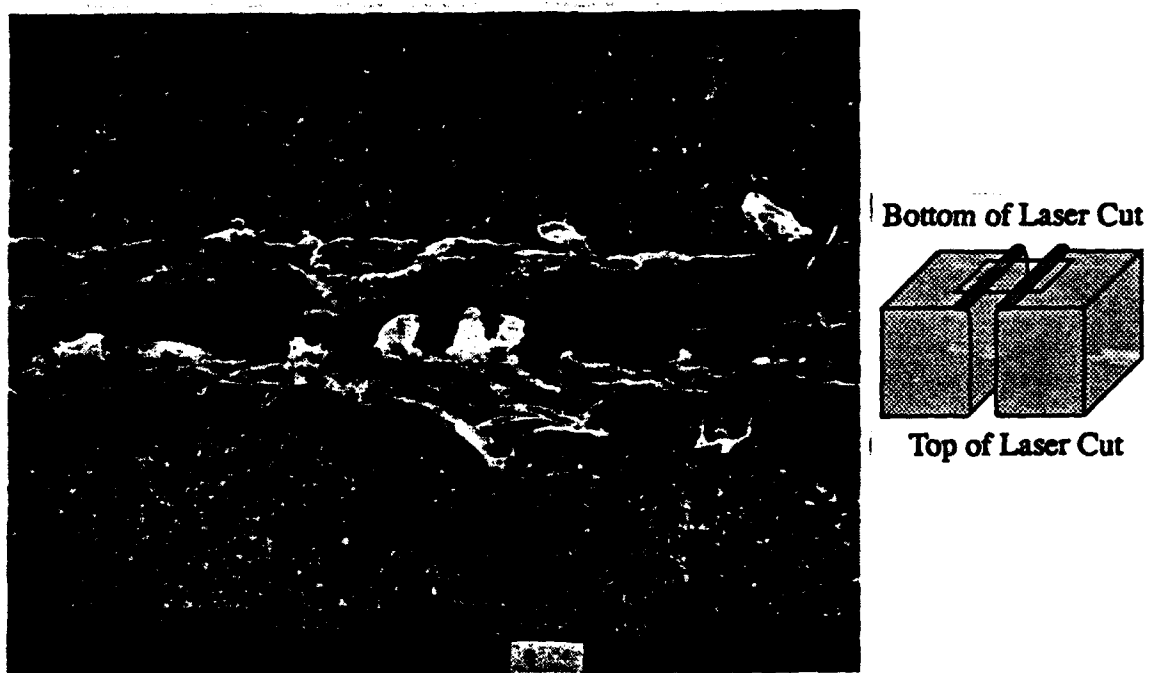
Figure 12.2. SEM micrograph of the cut exit of a 3 mm thick section of the 6061/ \text{Al}_2\text{O}_3 /20p composite cut at 6 cm/s.
