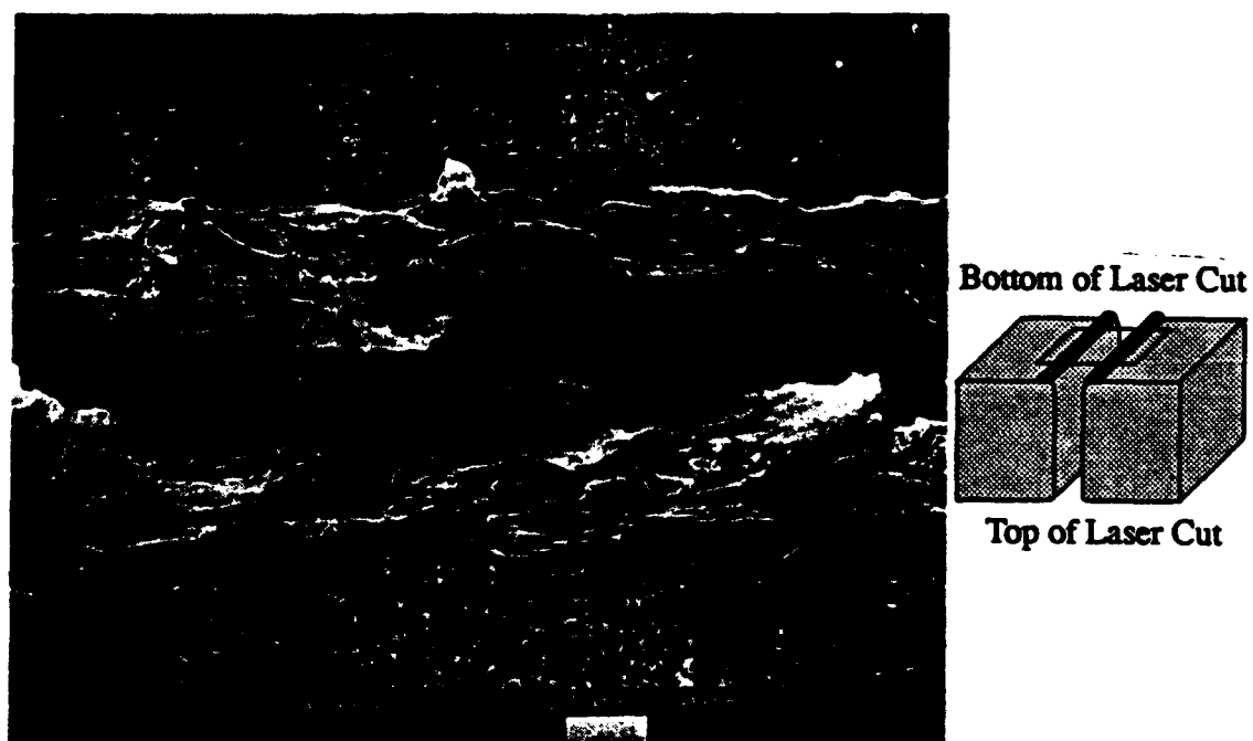
Figure 13.2. SEM micrograph of the cut exit of a 3mm thick section of the 6061/ \text{Al}_2\text{O}_3 /20p composite cut at 4 cm/s.
