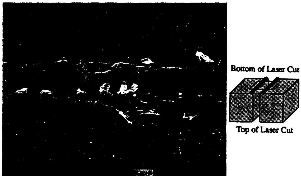
Figure 13.1. SEM micrograph of the cut exit of a 3mm thick section of the 6061/ \text{Al}_2\text{O}_3 /20p composite cut at 6 cm/s.
