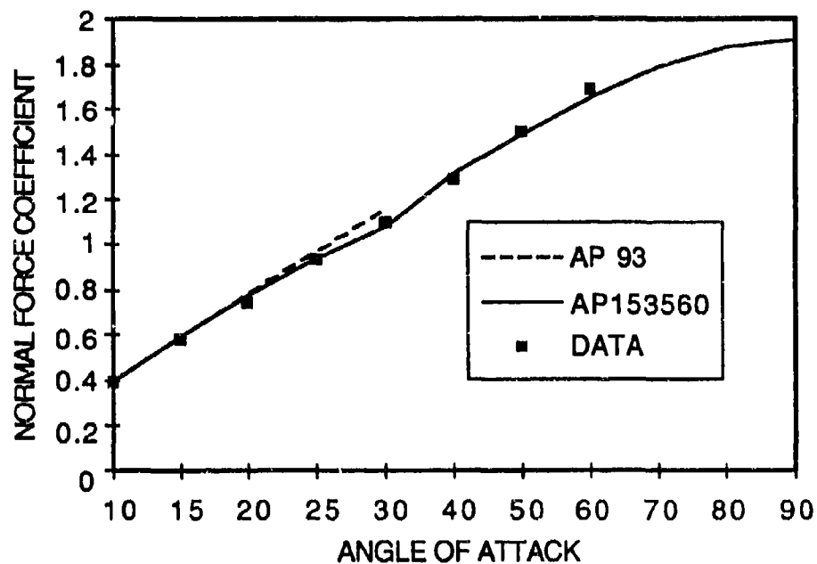
FIGURE 22. COMPARISON OF PREDICTED WING ALONE NORMAL FORCE COEFFICIENT WITH DATA ( AR = 2.0 , \lambda = .5 , M_\infty = 4.5 )
