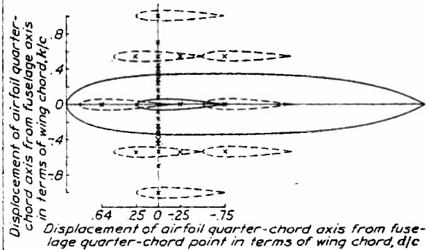
FIGURE 1.—A diagram of the various wing positions with respect to the fuselage.
