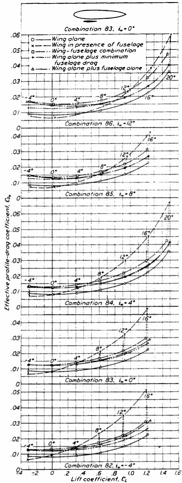
FIGURE 12.—Effect of mutual interference of wing and fuselage on disconnected low-wing combinations.
