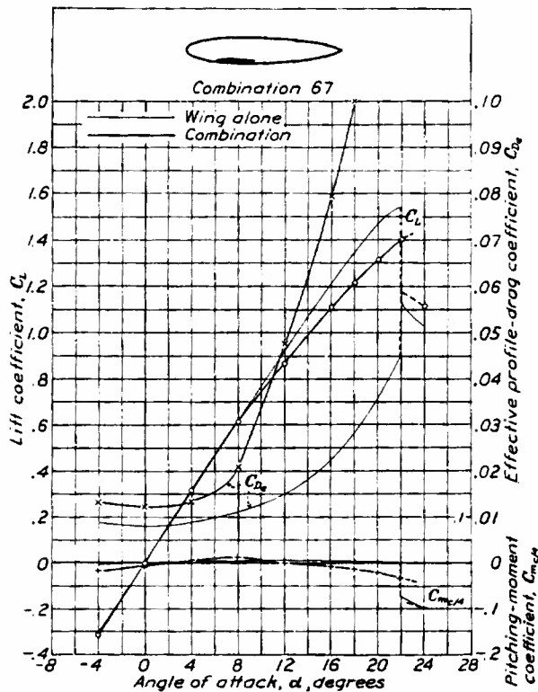
FIGURE 9.—Aerodynamic characteristics of a typical low-wing combination.
