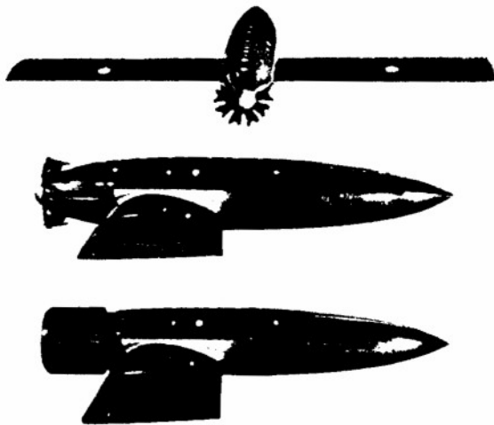
FIGURE 25.—Combinations showing round fuselage with cowed and uncowed engines.
