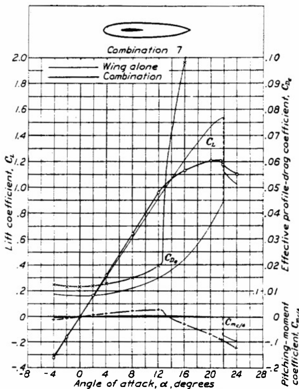
FIGURE 4.—Aerodynamic characteristics of a typical mid-wing combination.
