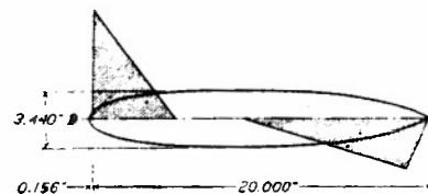
Source-sink distribution for round fuselage.
