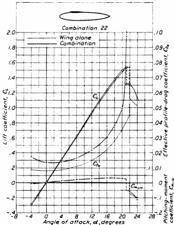
FIGURE 5.—Aerodynamic characteristics of a typical high-wing combination.
