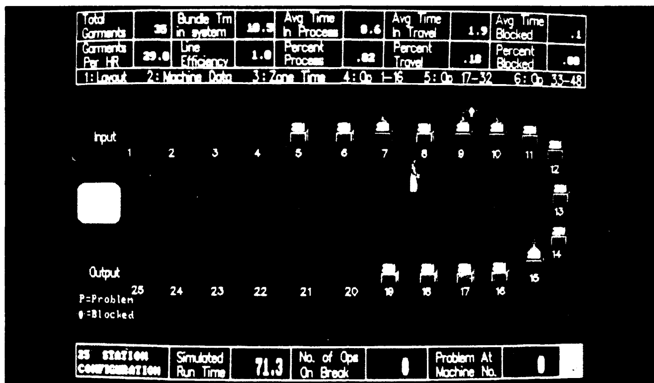
Simulation of a Modular Manufacturing Cell
