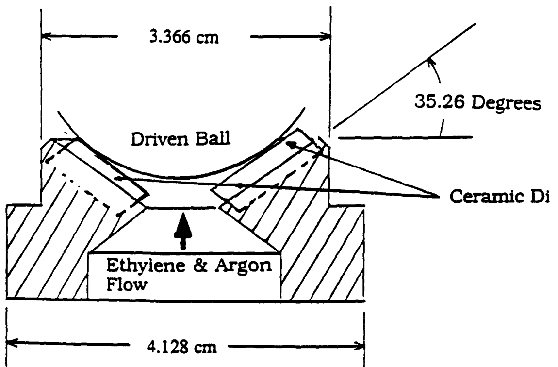
Fig. 2b Top view of modification showing the location of flat plates which replace lower bottom balls
