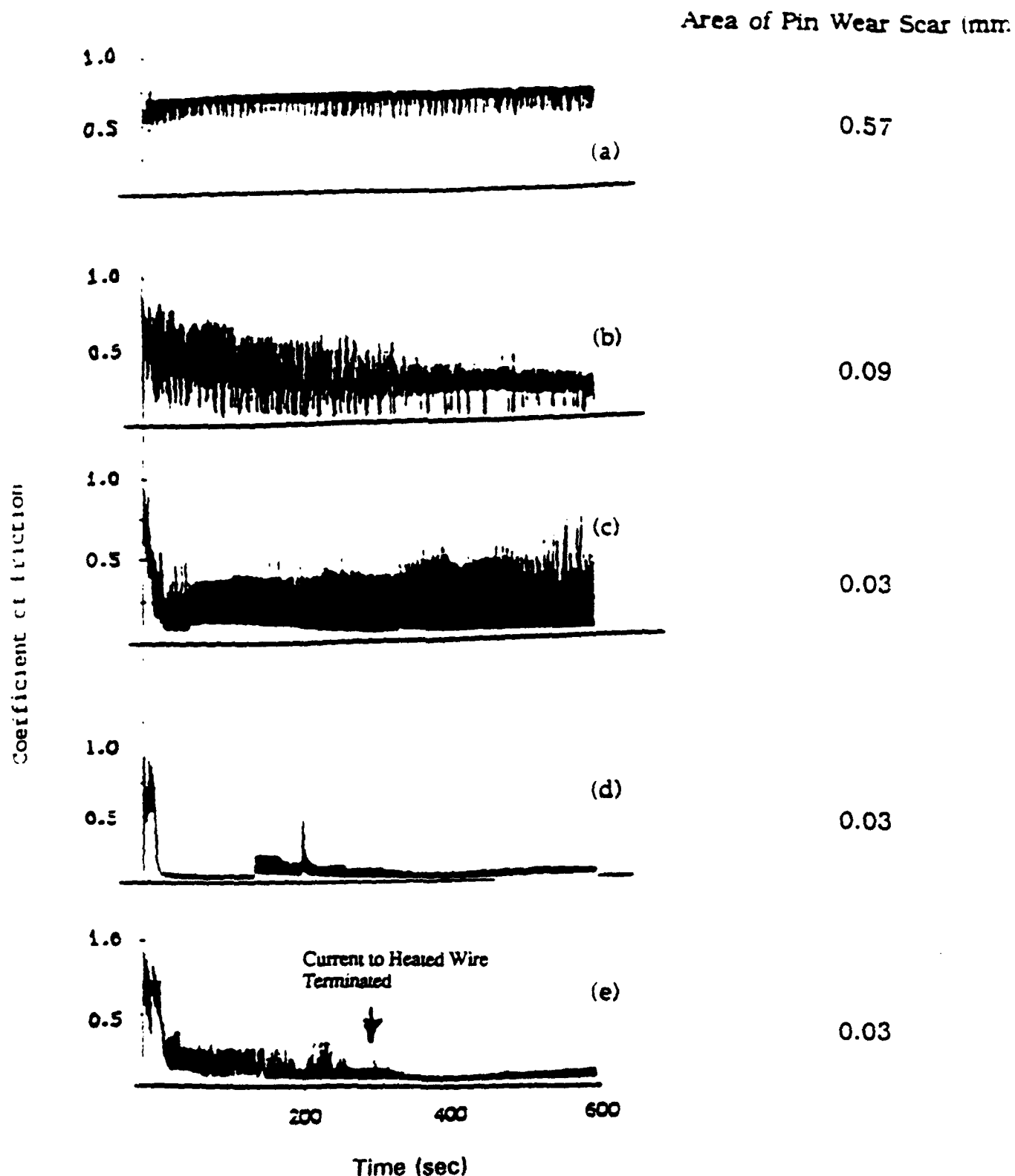
Fig 3. Silicon nitride pin-on-disc friction traces of 10 minutes duration and corresponding wear scar areas on the pin.
