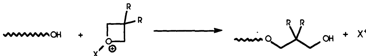
Figure 1. Depicted in this figure is the proposed mechanism for the propagation step of oxetane polymerization by the standard method and by the activated monomer method. The key difference is the activated monomer method involves attack of an alcohol on an activated monomer, which ensures rapid and complete initiator incorporation into the polymer chain.
