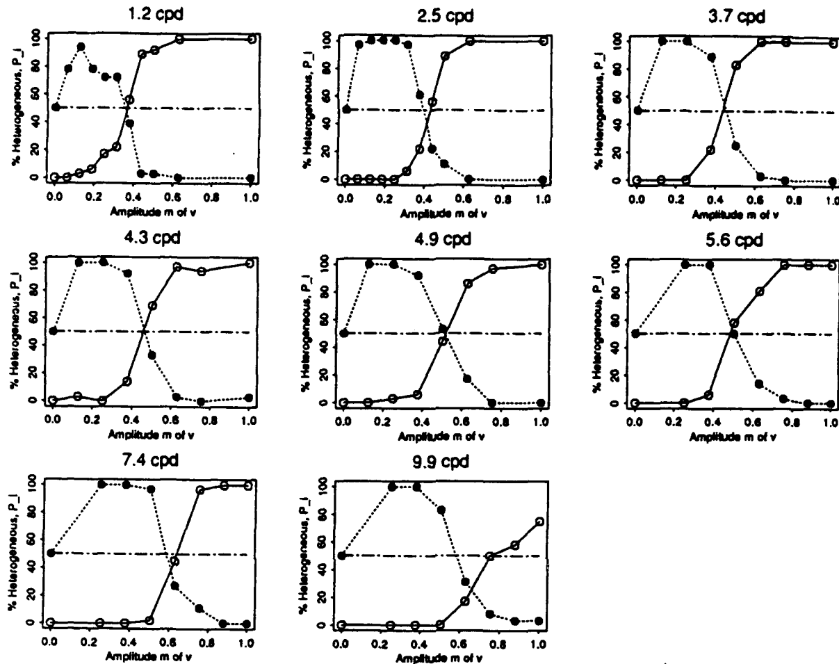
FIGURE 6. Probability P_1(m_v; \omega_v) of dominance of a heterogeneous motion path over a homogeneous motion path is shown as a function of the amplitude m_v of texture v for different spatial frequencies \omega_v of texture v for two subjects. Open circles represent the probability P_1(m_v; \omega_v) for Scheme I (Fig. 3); solid circles P_2(m_v; \omega_v) for Scheme II (Fig. 4). The horizontal dashed guide line indicates a 50% probability of heterogeneous motion dominance. The amplitude m_s and spatial frequency \omega_s of texture s is the same for all panels: m_s = 0.5 and \omega_s = 4.9 c/deg. (a) Subject PW; (b) subject JS.
