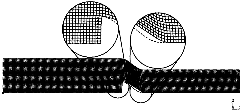
Figure 19: Nodal displacements with no nodes released; axial load in tension
