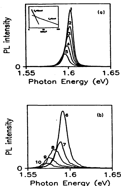
FIG. 7. The photoluminescence spectra of a CdTe/Cd 0.79 Zn 0.21 Te single-quantum-well heterostructure of well width L_w = 75 Å, measured at different temperatures between (a) 10 and 50 K (step 10 K), and (b) 60 and 100 K, under indirect excitation with Ar + -ion laser line 488 nm. The inset shows the Arrhenius plot of integrated PL intensity versus 1/T which reveals two activation energies 25 and 5 meV.
