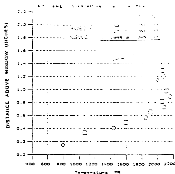
Fig. 12 Comparison between rake survey of pitot pressure and total temperature over HED window in NSWC and shock tunnel facilities.
