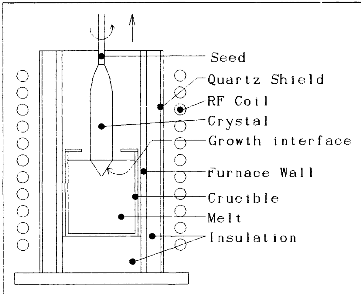
Figure 1 Czochralski (CZ) Crystal Setup
