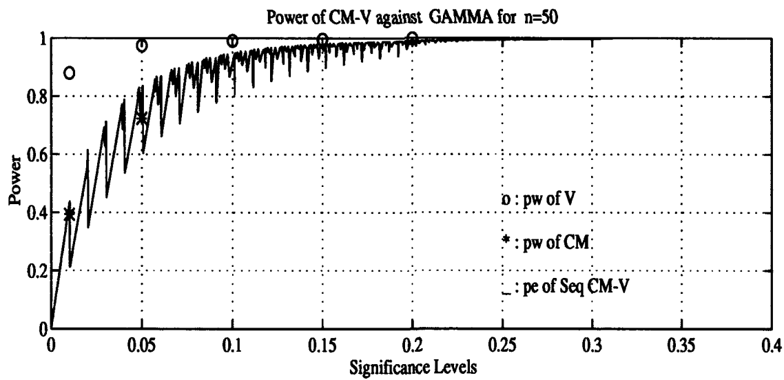
Figure D.4 Power comparisons of CM - V against Gamma
