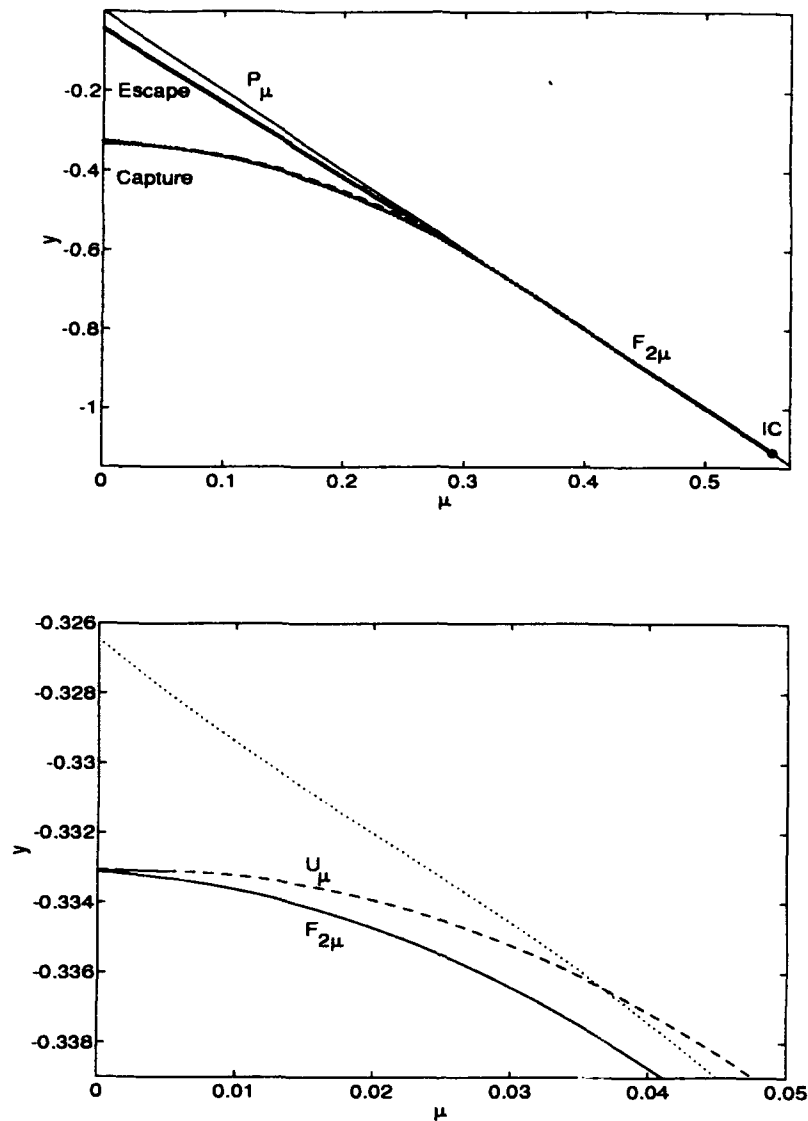
Figure 20. Capture and Escape of Two Identical Spacecraft Having Kinsey's Geometric Parameters and Different Motor Torques. Capture: K = 0.4 . Escape: K = 1.2 . These are shown by the dark lines in the upper plot. The lower plot is a closeup of the "captured" trajectory toward the conclusion of spinup.
