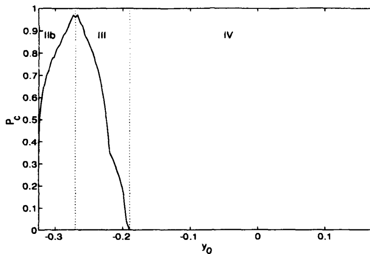
Figure 37. Probabilities of Capture in the Domain of O_\mu ( \varepsilon = -0.01 and \mu = 0.1 ). i_1 = 0.7, i_2 = 0.3, i_3 = 0.8, \alpha_1 = 0.5, \alpha_3 = 0.866
