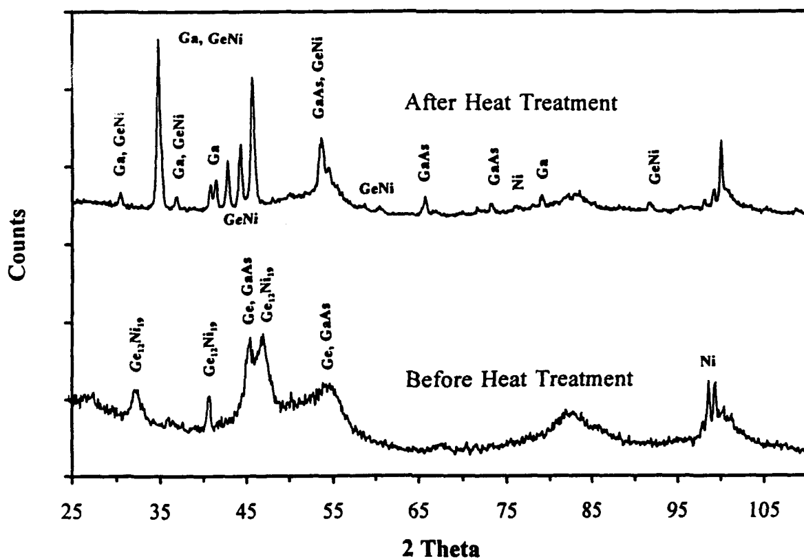
Figure 3. XRD spectra of NiGe/n-GaAs system before and after heat treatment at 500C for 1 min. Heat treatment produces the \text{NiGe} product phase.
