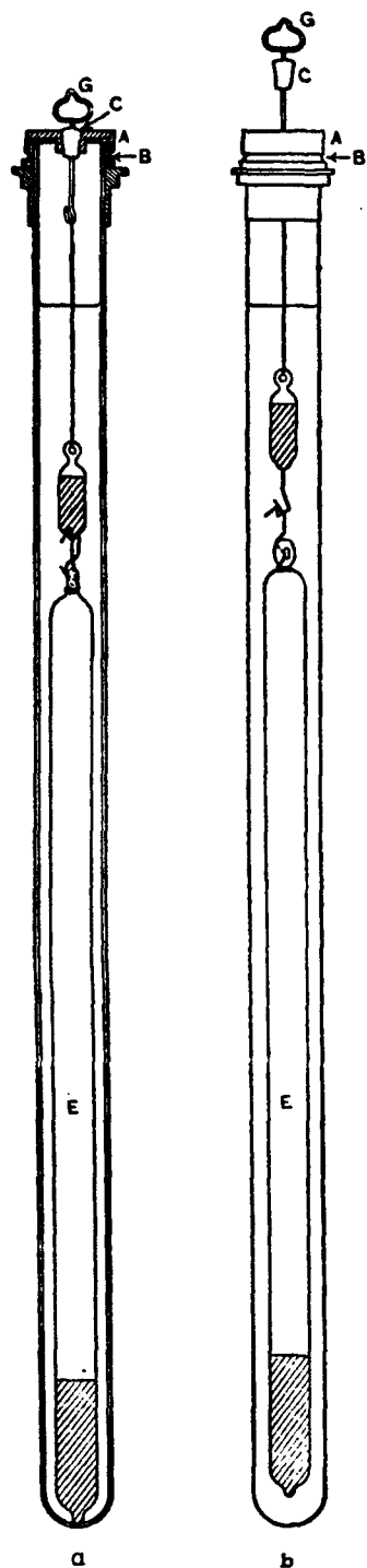
FIGURE 1. Densimeter tube, one-third size (Osborne).
