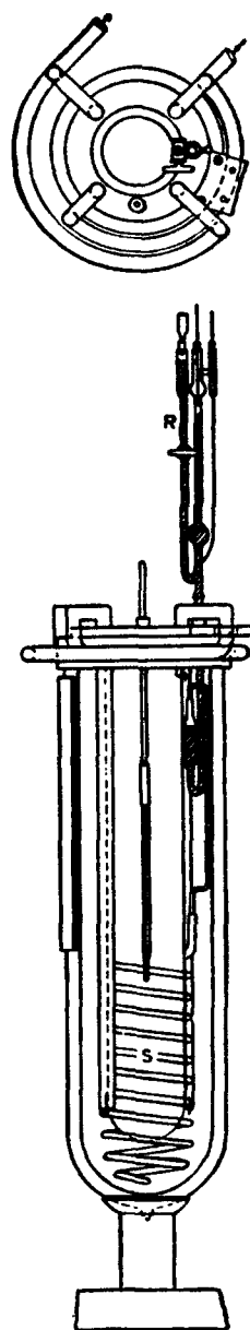
FIGURE 4. Bath for use in determination of density by hydrostatic weighing method, one-eighth size (Osborne).
