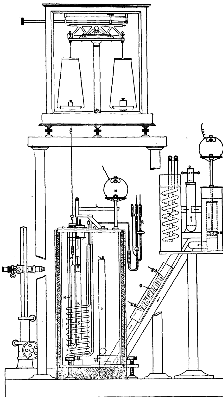
FIGURE 3. Apparatus for determination of density by hydrostatic weighing method, one-ninth size (Osborne).
