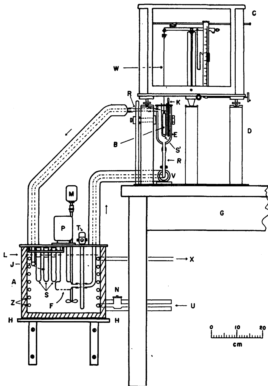
FIGURE 6. Density balance for determinations of the density of liquids (Fcrziati, Mair, and Rossini.)
