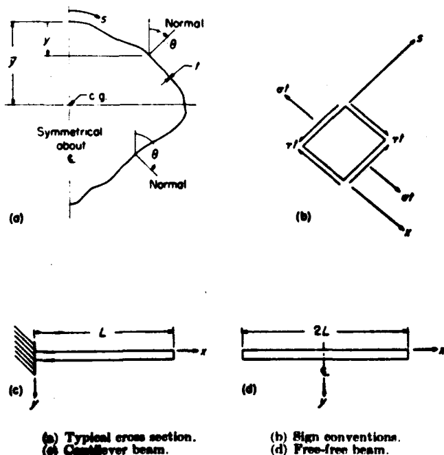
FIGURE 1.—Coordinate systems and sign conventions.
