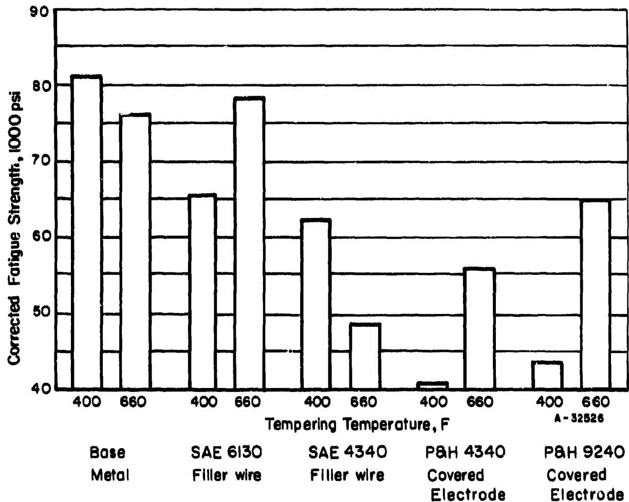
FIGURE 1. FATIGUE STRENGTHS OF WELD JOINTS IN 1/4-INCH-THICK AMS 6434 STEEL(7)
