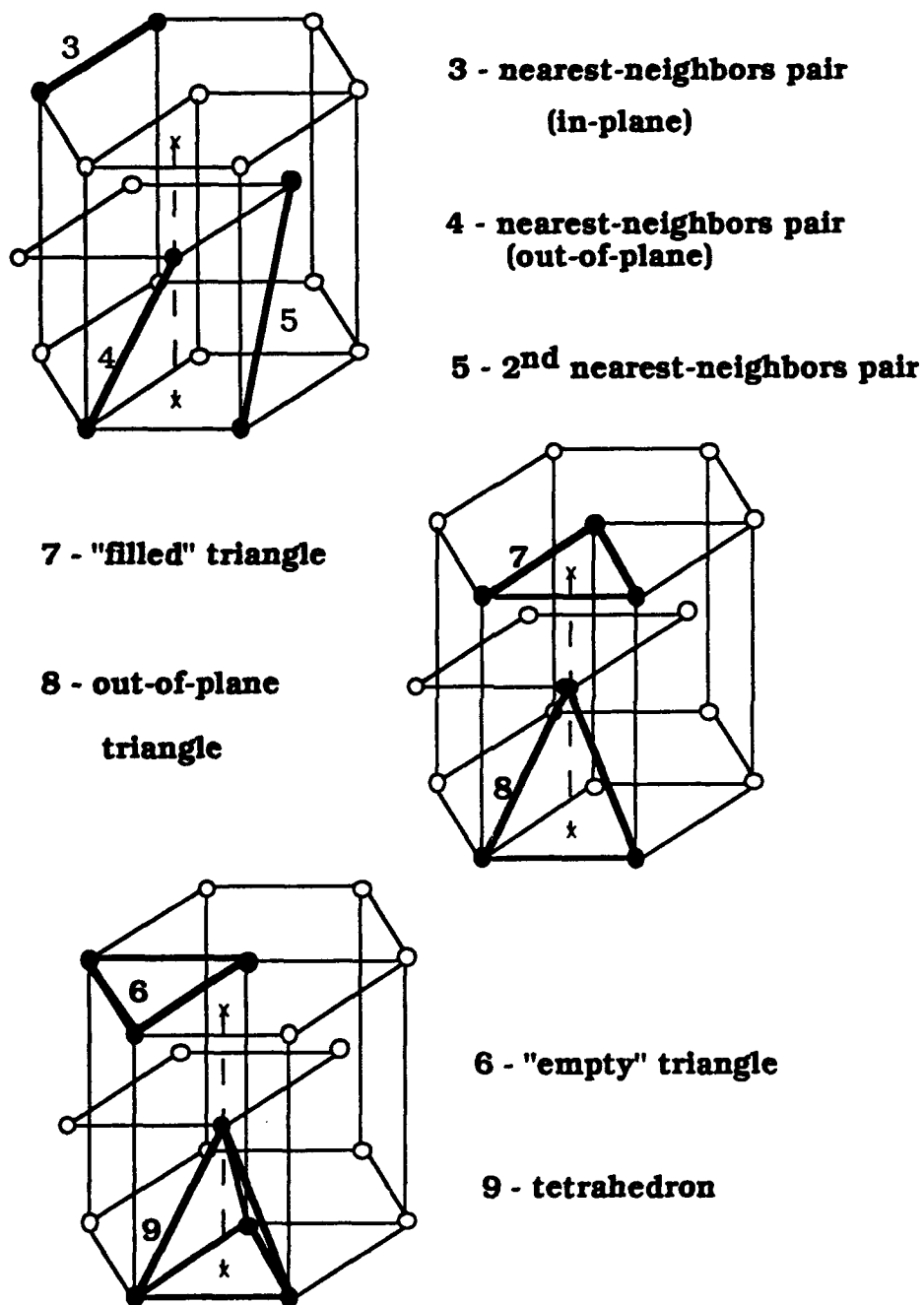
Figure 2.1 b. Typical clusters and their designated numbers for the hcp lattice.
