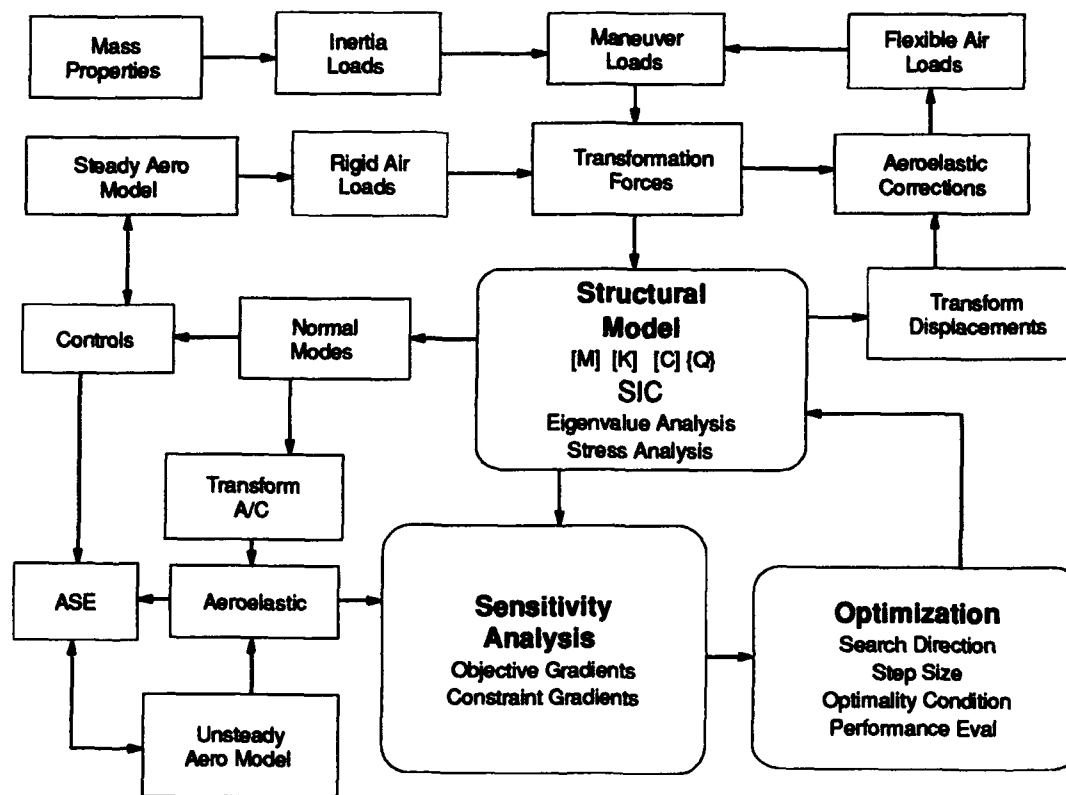
Figure 1.1 ASTROS Interdisciplinary Design
