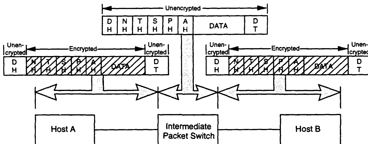
(b) Effect of Link Encryption on Headers
