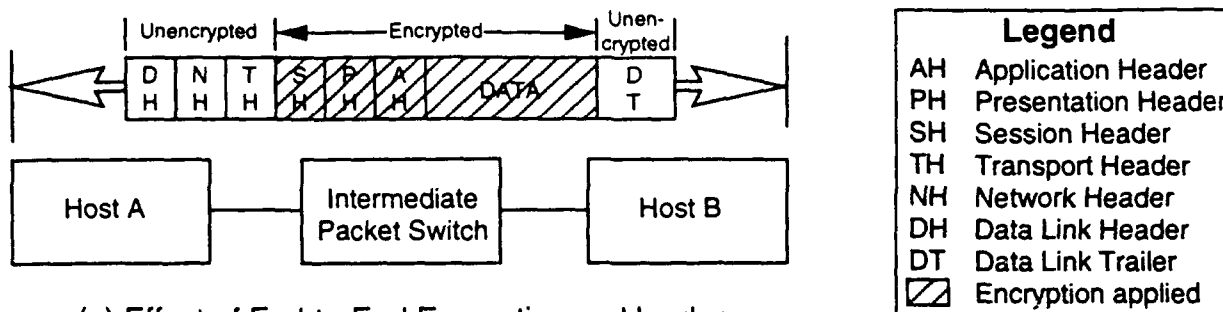
(a) Effect of End-to-End Encryption on Headers
