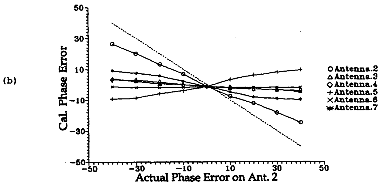
Figure 5. Calculated Phase Error Corrections Using Mode 2.
