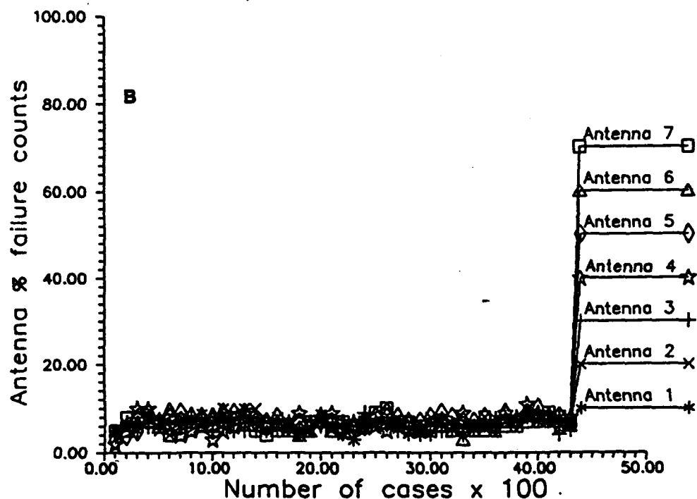
Figure 10. Number of Failure Counts for Phase Testing in Quality Control, Qaanaaq Digisonde 256, Days 87328 through 87330.
