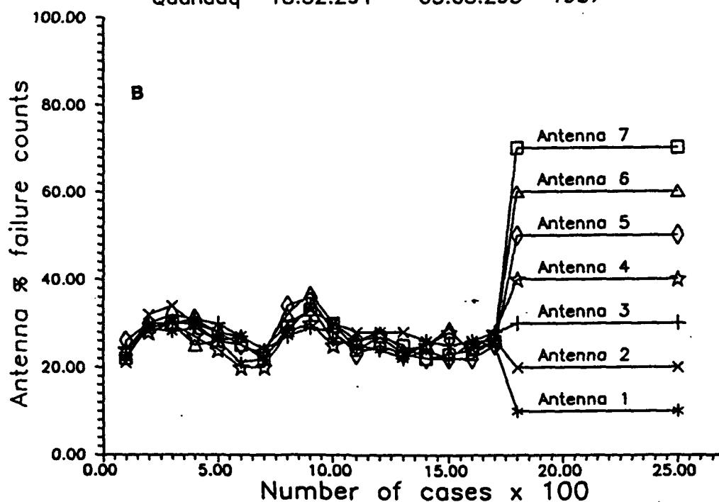
Figure 9. Number of Failure Counts for Phase Testing in Quality Control, Qaanaaq Digisonde 256, Days 87291 through 87293.
