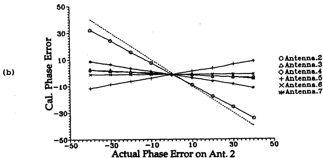
Figure 4. Calculated Phase Errors Using Mode 1.
