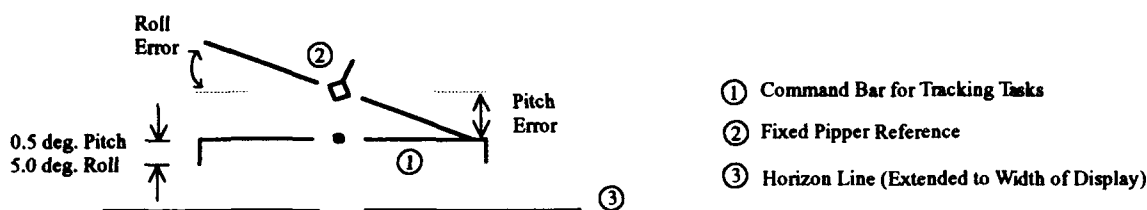
Figure 4-2. Tracking Task Display
