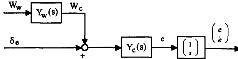
Figure 3-4. Noise Injected at Aircraft Input
