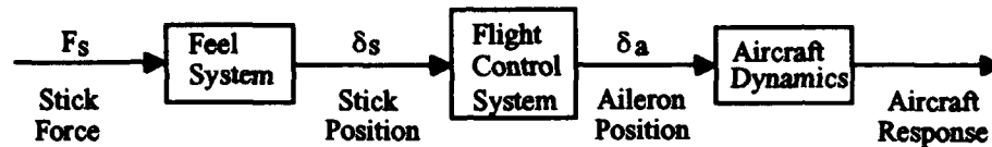
Figure 2-6. Position Command Feel System
