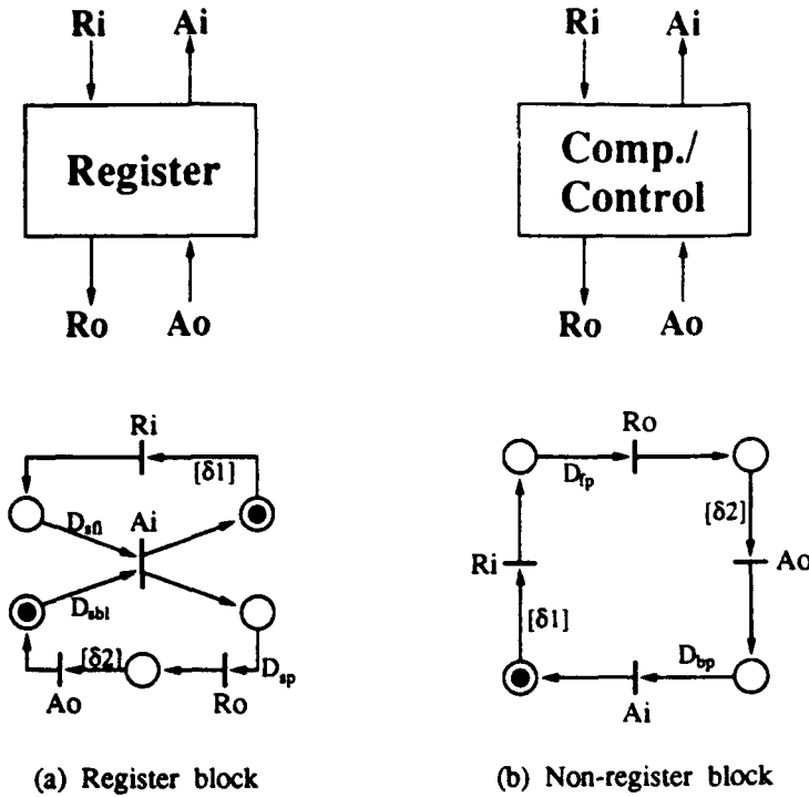
Figure 18: Timing model for asynchronous blocks.
