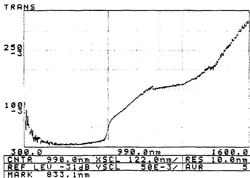
Fig. 5 Transmission of 0.15um thick CdTe Ring
