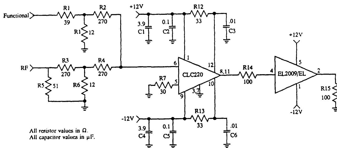
Figure A-1. Op Amp Combiner.
