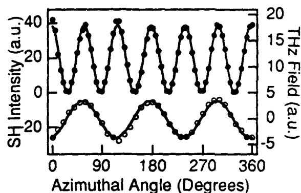
Fig. 3: Same as Fig. 2 except the polarization of the nonlinear signals is detected parallel to the fundamental light. The solid line is calculated from Equations (1) and (3).
