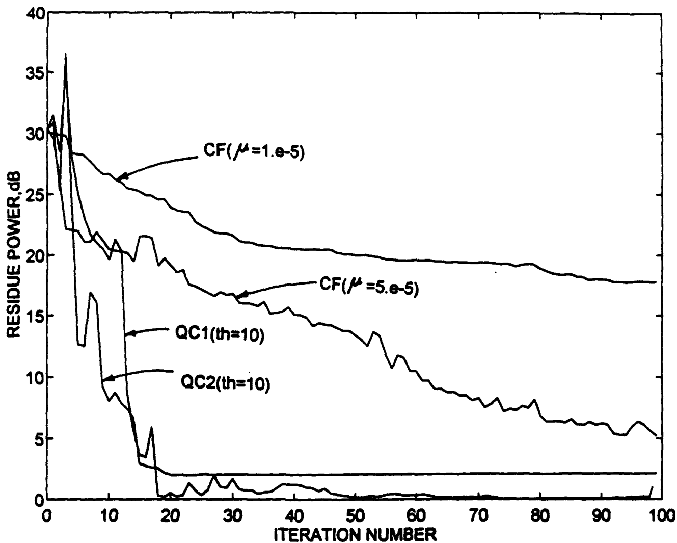
Figure 8. Convergence of various recursive algorithms (two jammers 28dB and 38dB above noise)
