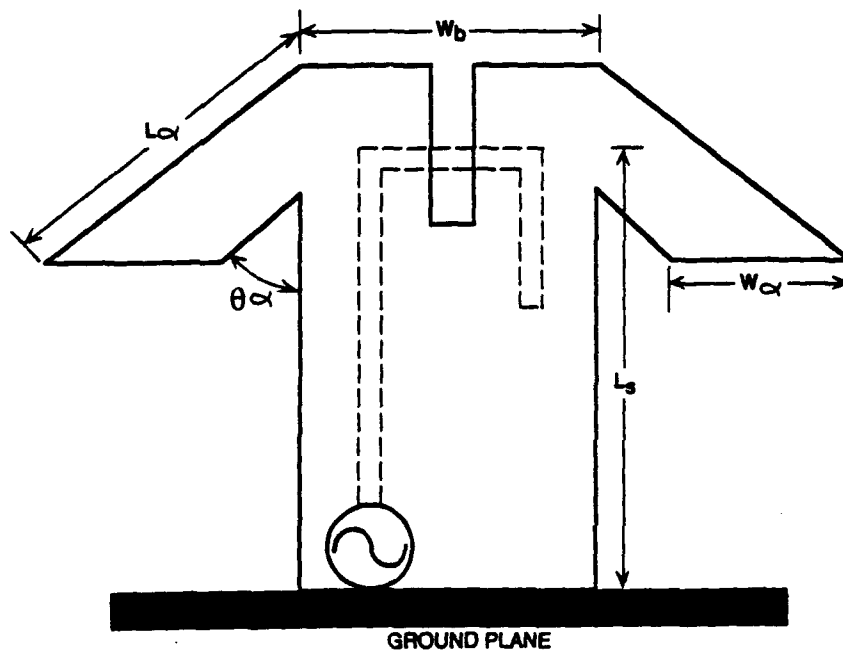
(b) Dipole element with bent arms
