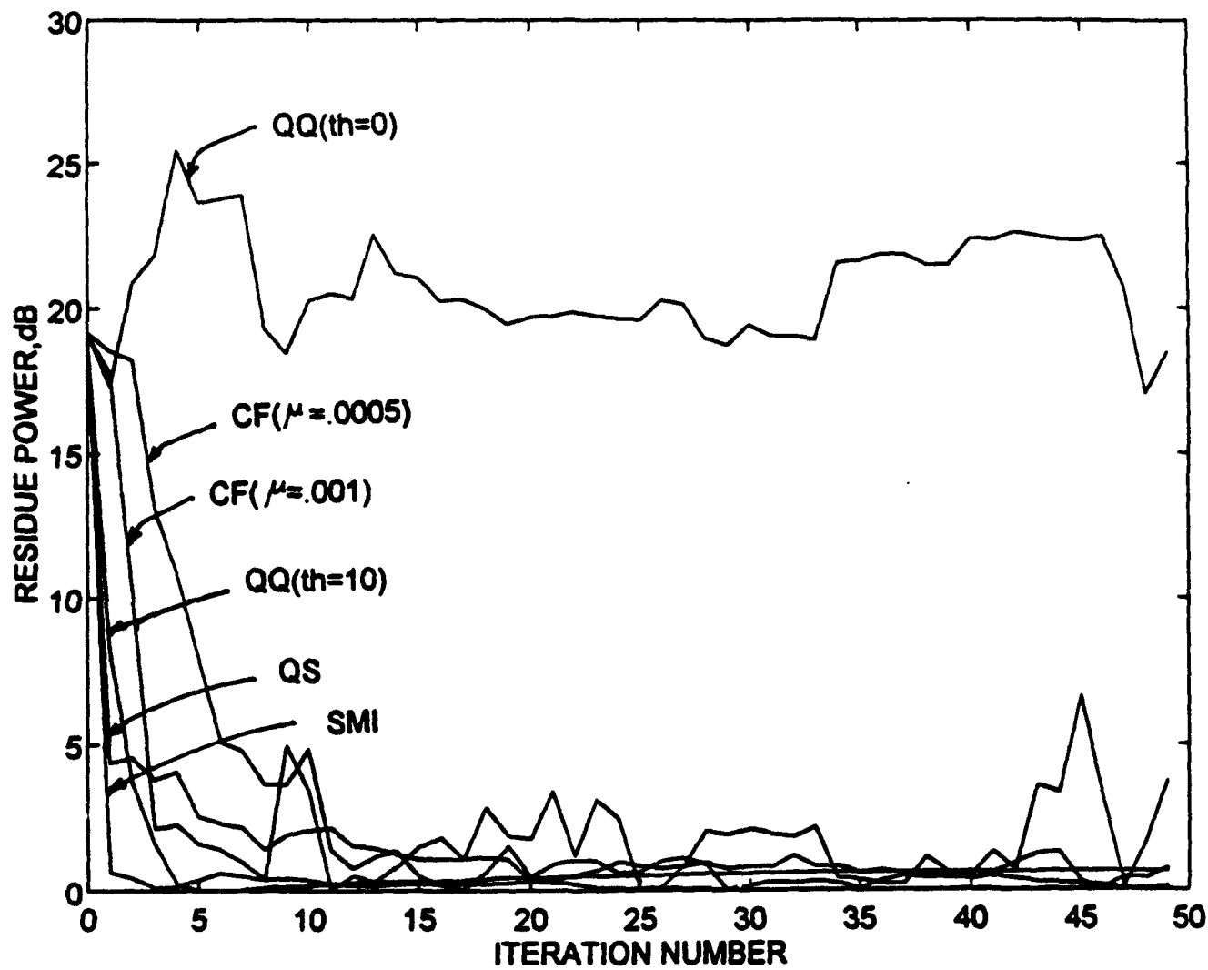
Figure 5. Convergence of various algorithms (single jammer 28 dB above noise)
