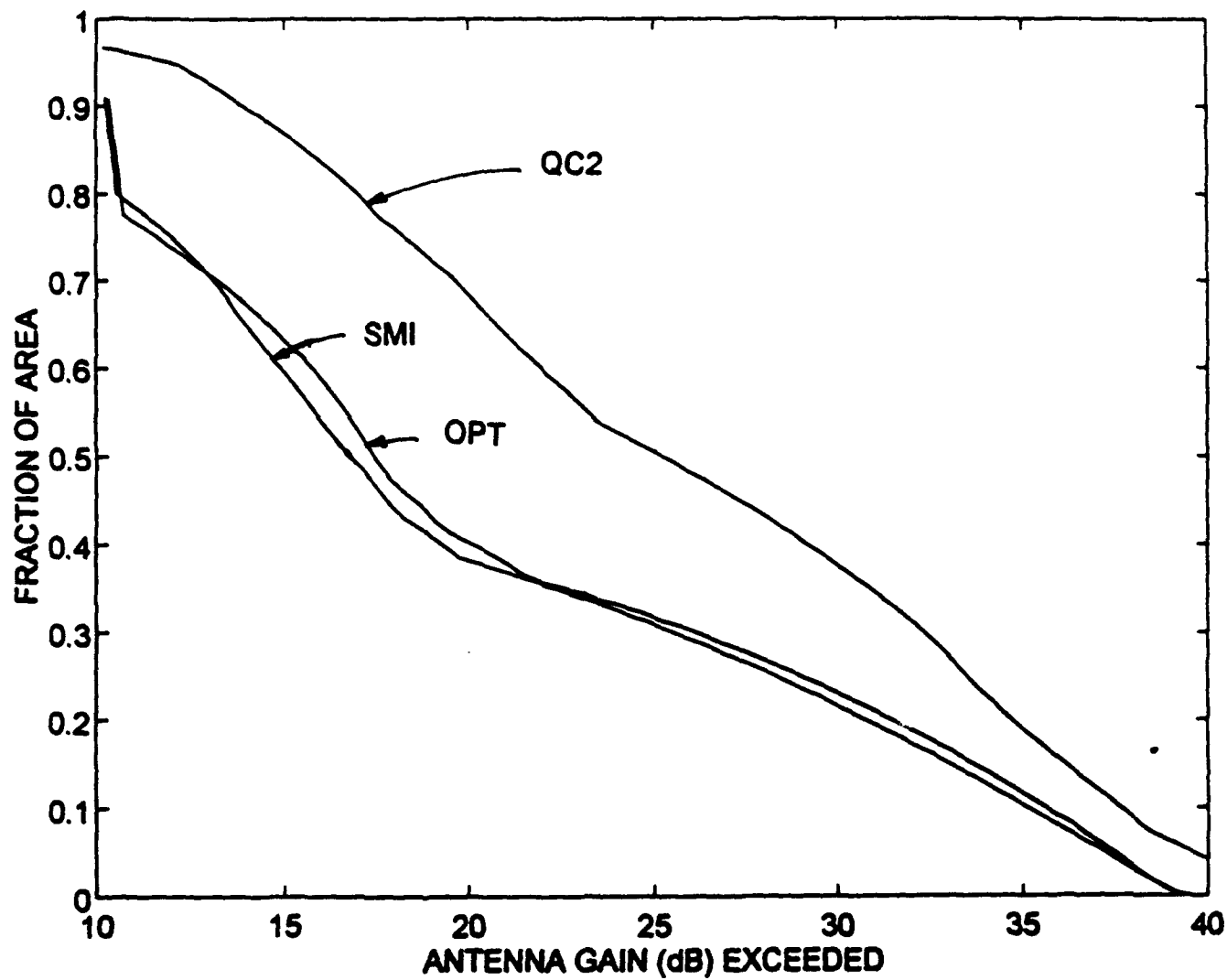
Figure 10. Antenna gain distribution in the region containing jammers
