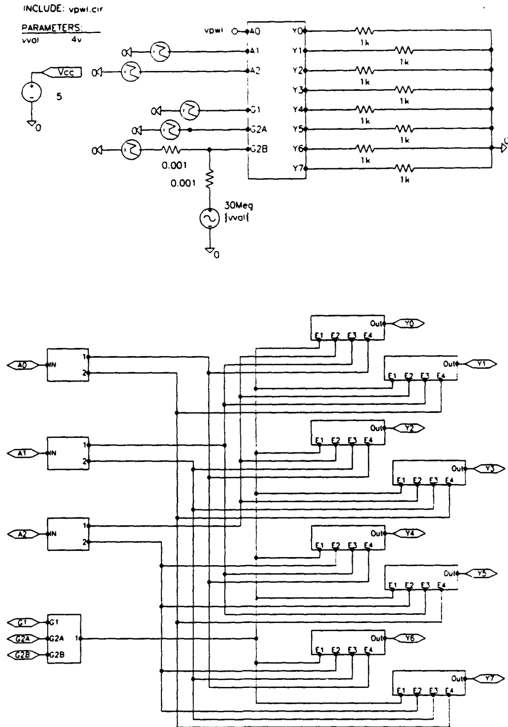
Figure 2. 74S138 3-Line to 8-Line Decoder Schematic (1/2)
