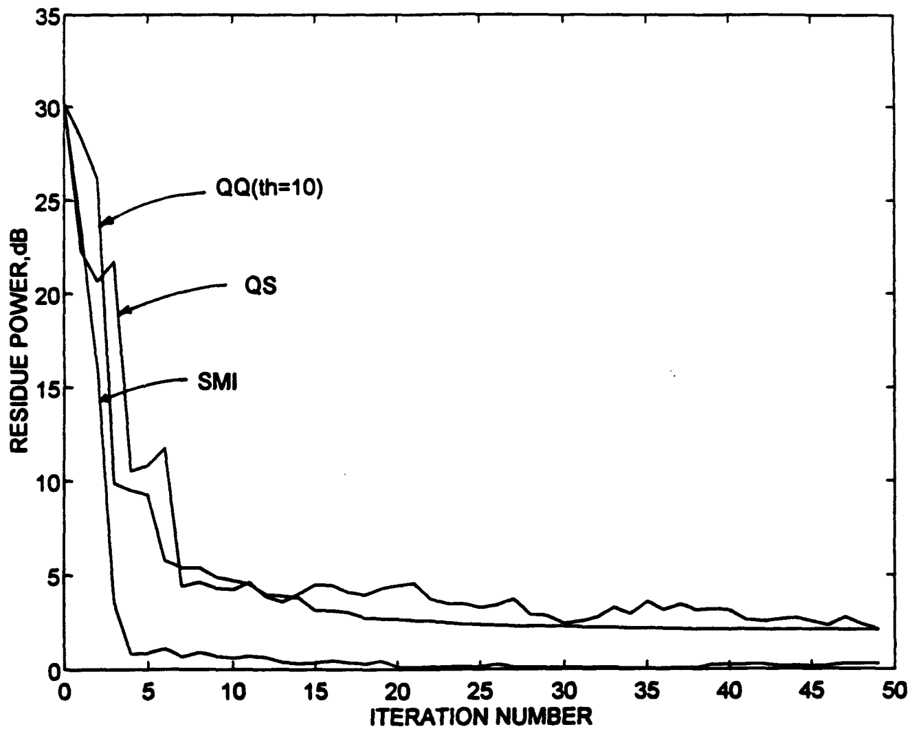
Figure 7. Convergence of various nonrecursive algorithms (two jammers 28dB and 38dB above noise)
