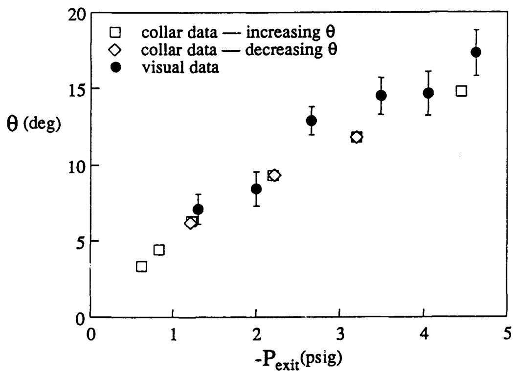
Figure 5: Thrust vector performance curve for T_0=300\text{K} and a gap of 5.0 mm.
