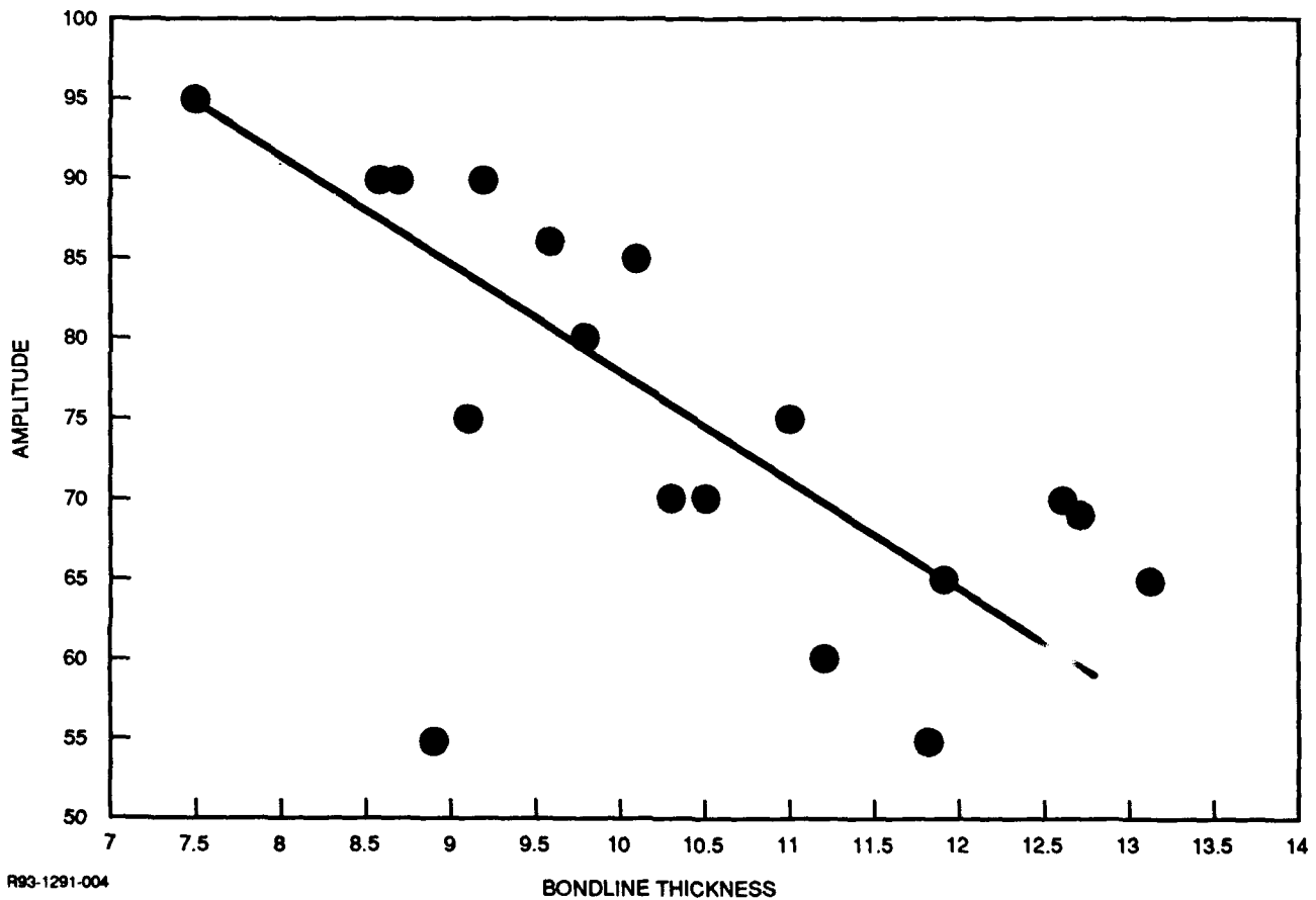
FIGURE 1. EFFECT OF BONDLINE THICKNESS
