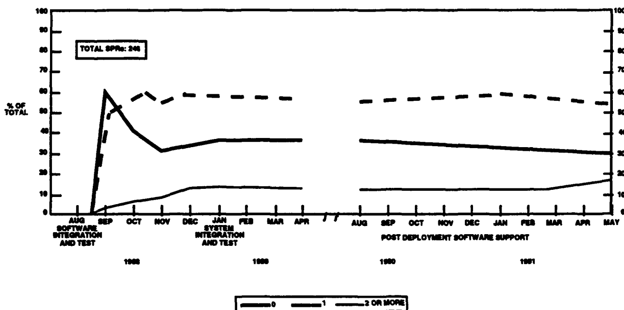
Figure 3.2.2-1 SPRs Categorized By Number of Modules Changed
