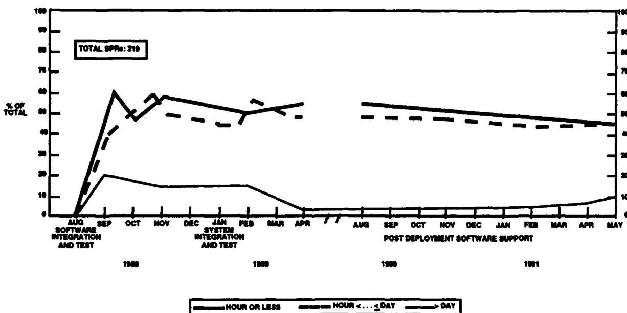
Figure 3.2.3-2 SPR Resolution Effort Categories: Expected Changes Only
