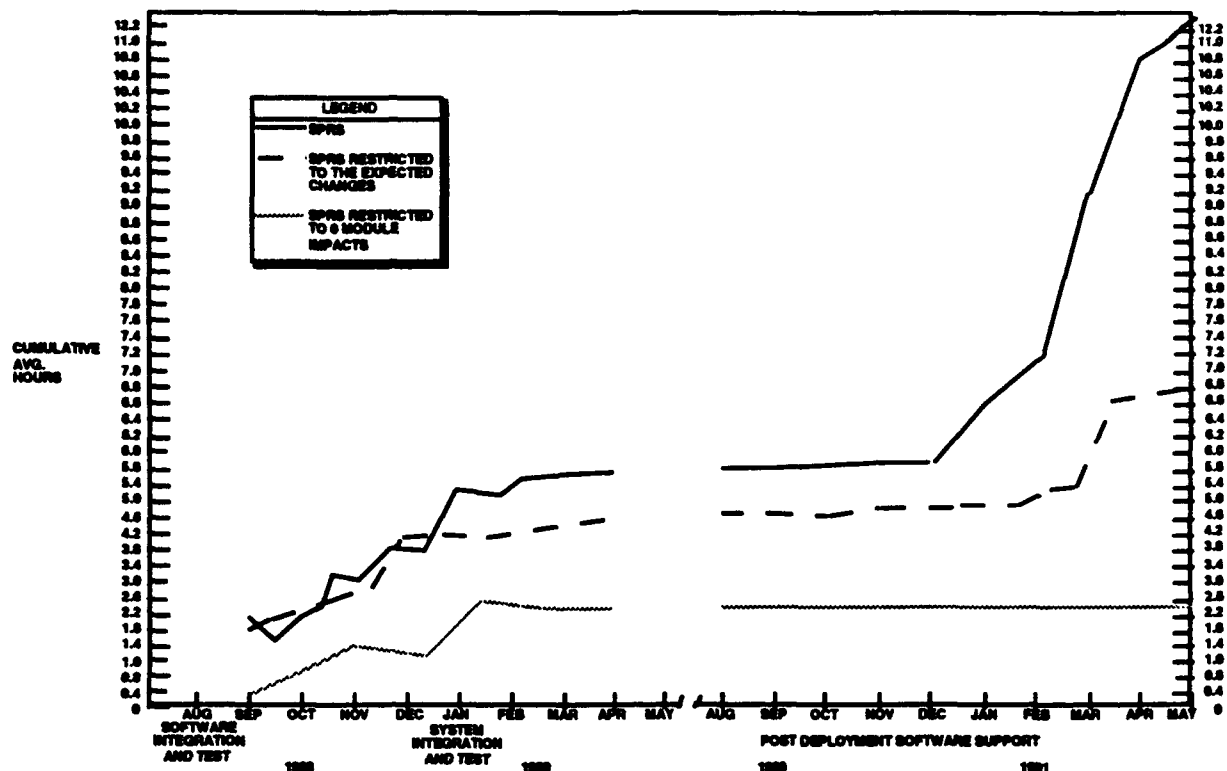
Figure 3.2.5-1 Cumulative Average Resolution Effort: By Close-Out Date
