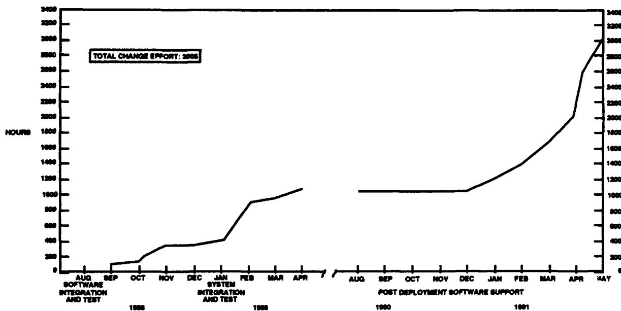
Figure 3.1-2 Cumulative SPR Resolution Effort
