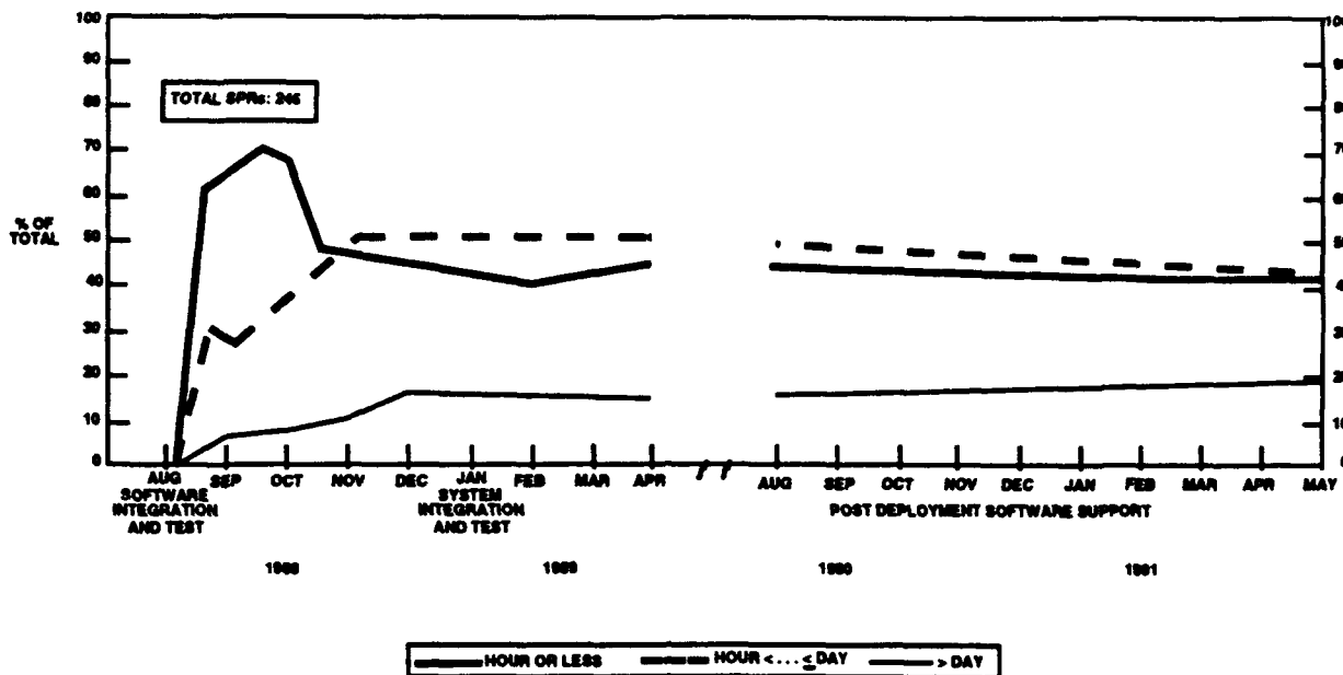
Figure 3.2.3-1 SPR Resolution Effort Categories
