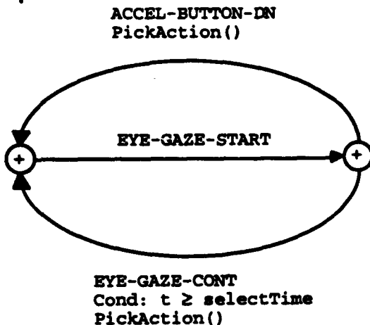
FIGURE 3: STATE TRANSITION DIAGRAMS FOR AN EYE-SELECTABLE OBJECT. Nodes in diagrams represent states in human-computer interaction, waiting for events. Directed arcs represent events triggered by user actions. Upper-case words label events. Expressions which include parentheses indicate function calls. Cond: specifies a condition that must hold before its associated event triggers a state change.
