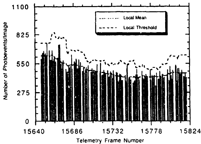
Fig. 55 - Plume camera, total intensity for interval 1
