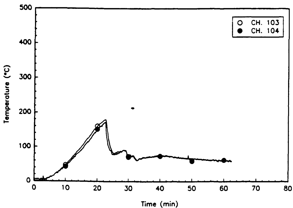
Fig. A86 - CIC deck temperatures, COL_10
