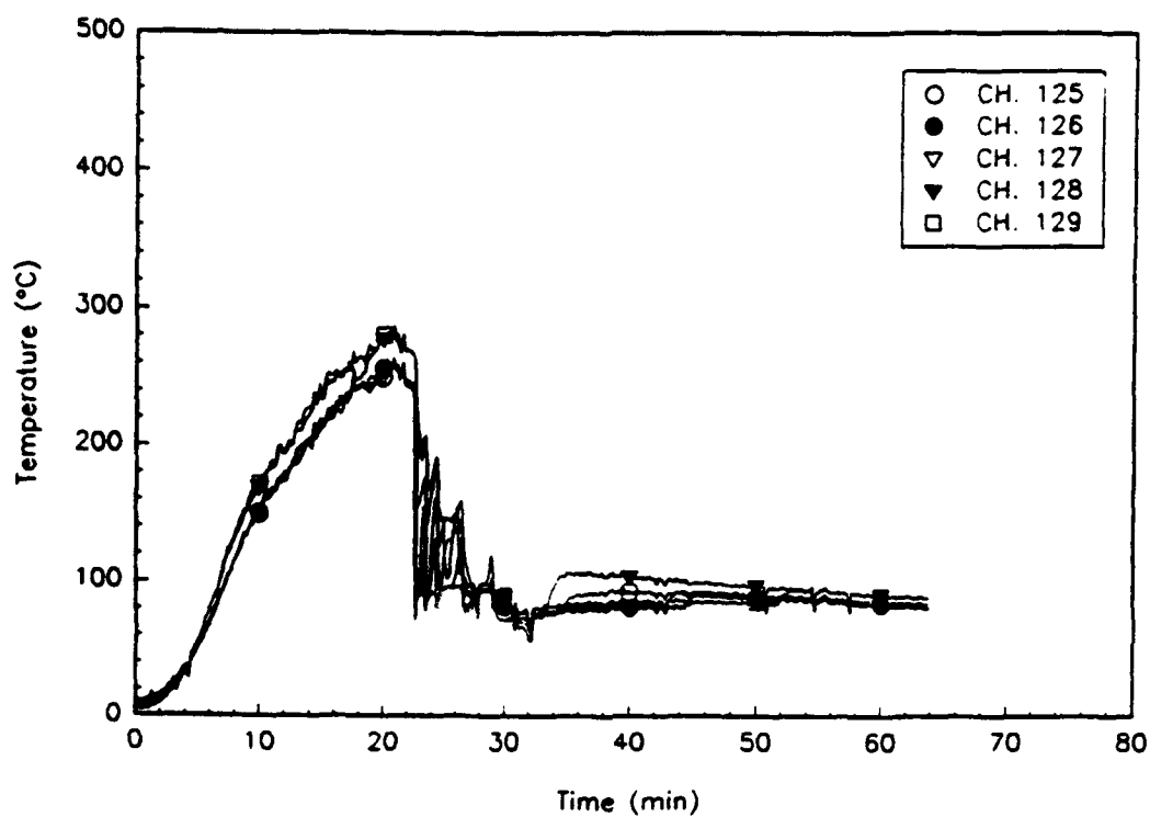
Fig. A46 – RICER 2 air temperatures forward, COL_6
