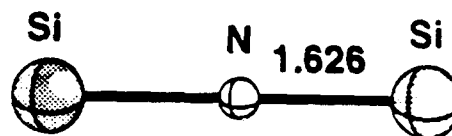
\text{Si}_2\text{N}^-, \text{VI} (\text{D}_{\infty\text{h}}, 3\Sigma_{\text{g}}^-)
