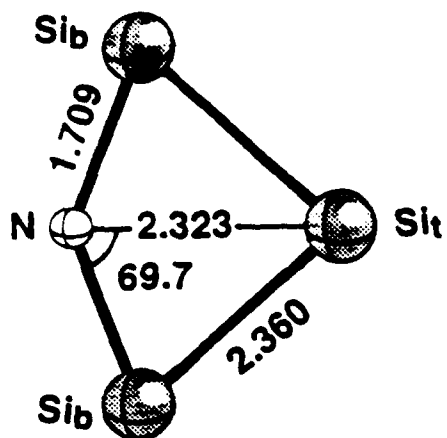
\text{Si}_3\text{N}^- , XXXII ( \text{C}_{2v} , ^1\text{A}_1 ) 18.8
