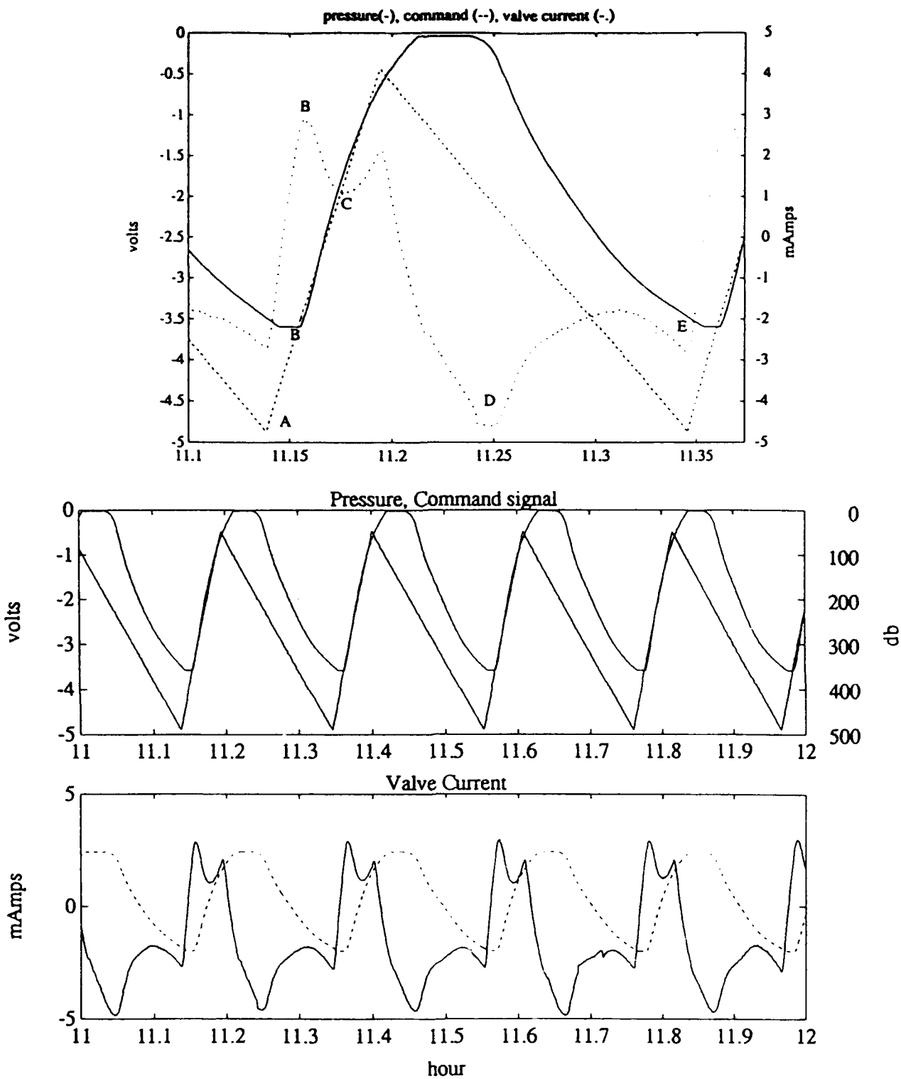
Figure 3: Top: Pressure (solid), command (dashed) and valve current (dash-dot) for one dive cycle. Symbols "A" to "E" are referenced in the text. Middle: 1 hour time series of pressure and command signal. Bottom: 1 hour time series of valve current; pressure (dashed) is included as reference.
