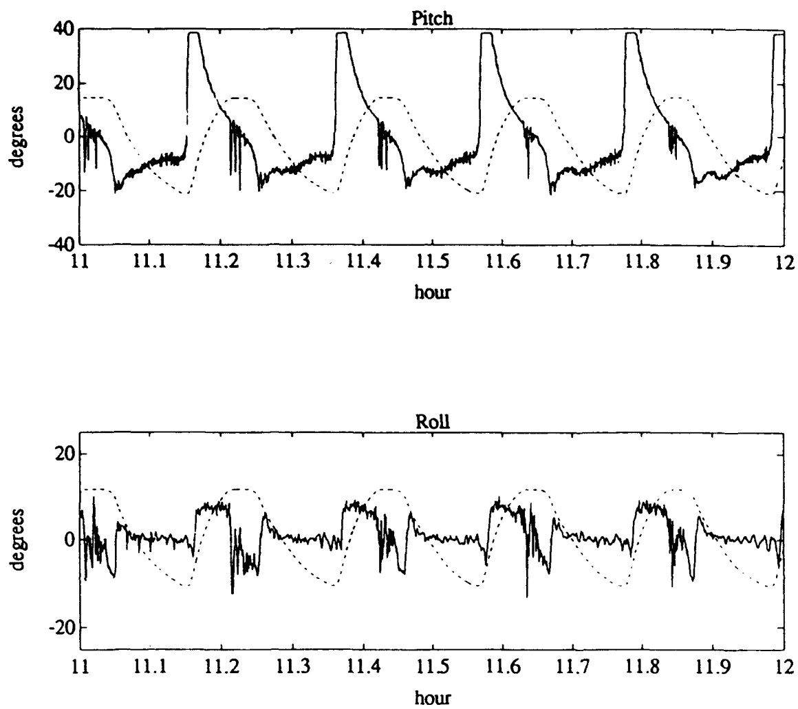
Figure 8: Time series of pitch (top), and roll (bottom); pressure (dashed) is included as reference.
