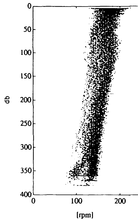
Figure 7: Profile of impeller rotation.
