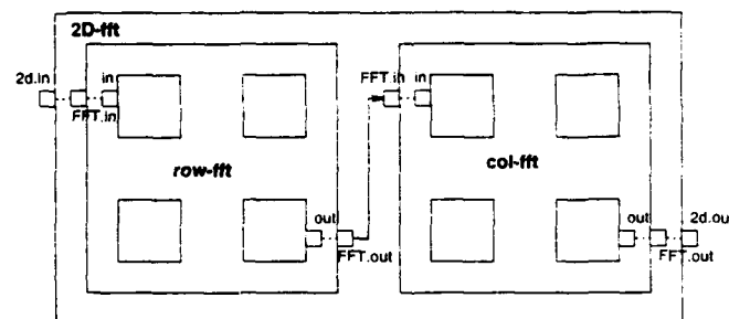
Figure 7: Array module composition of 2D-FFT array module from two 1D-FFT array modules. The dotted lines show mappings between local and external ports.
